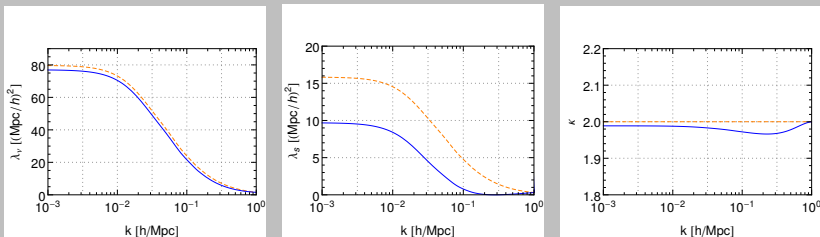
Figure: RG evolution of \lambda_\nu(k) , \lambda_s(k) and \kappa(k) . We have initialized the flow at k = \Lambda = 1 h/ \text{Mpc} with the one-loop values. The solid lines correspond to the solution of the full flow equations, while the dashed lines correspond to the solution of the one-loop approximation.
