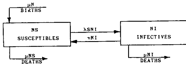
Fig. 1. The compartmental diagram for the SIS model.
