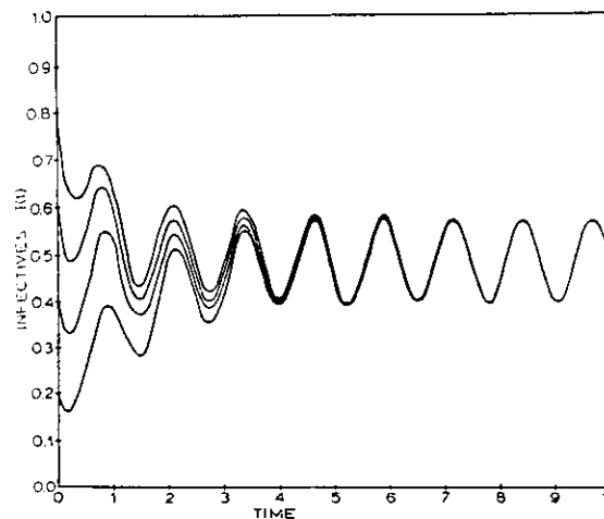
Fig. 4. Solutions as in Fig. 3 except that here \gamma = 1 so that \bar{\sigma} = 2 > 1 . From Hethcote (1973).
