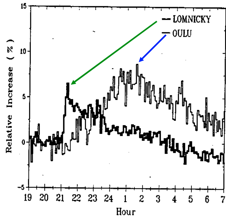
Strongly anisotropic event
