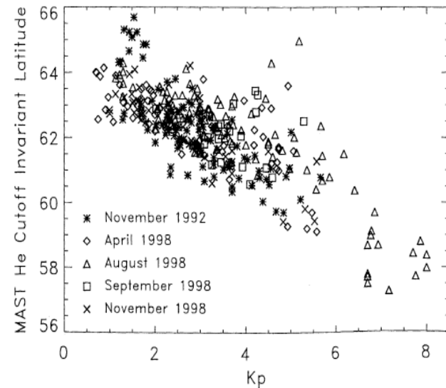
Figure 6. Orbit-averaged cutoff invariant latitude for \sim 8-15 MeV/nucleon He plotted versus K_p interpolated to the same time as the cutoff measurement, for the five time periods indicated.
