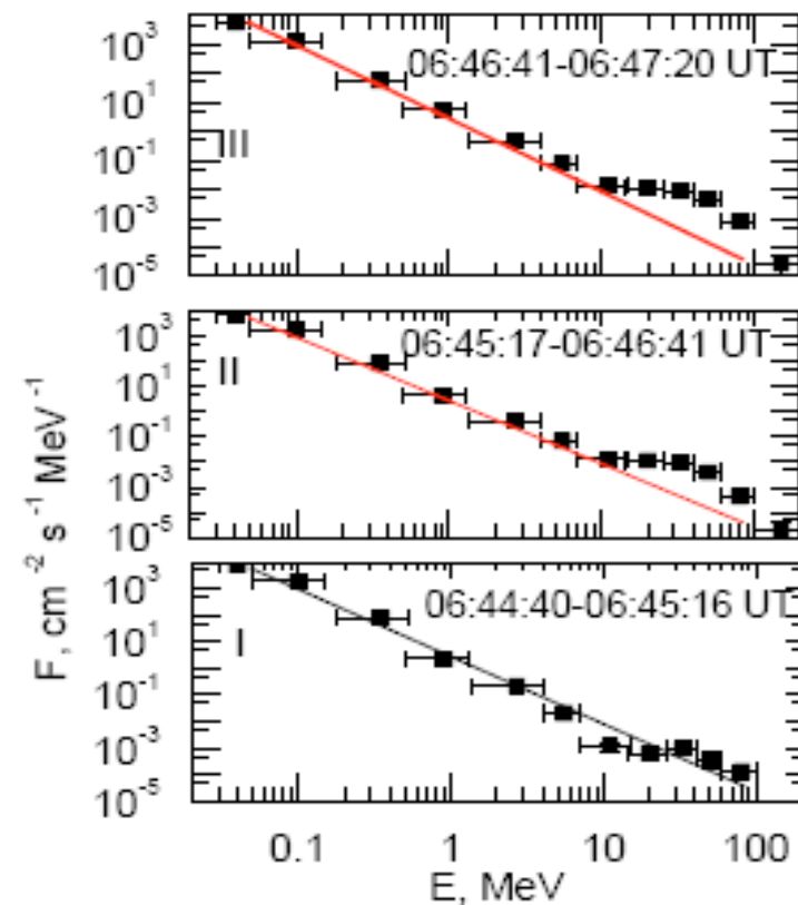
Figure 3. The energy spectra of gamma rays observed by SONG during three time intervals marked in Figure 2.
