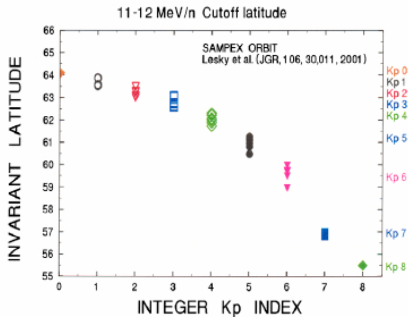
Fig. 9. Comparison of the measured and computed average invariant cutoff latitude. Top: the event summary cutoff latitude measured by SAMPEX. (Reproduced from Leske et al. (2001) by permission of the American Geophysical Union.) Bottom: the event-averaged computed cutoff latitude for 11.5 MeV/n \alpha particles (0.294 GV) from this work.
