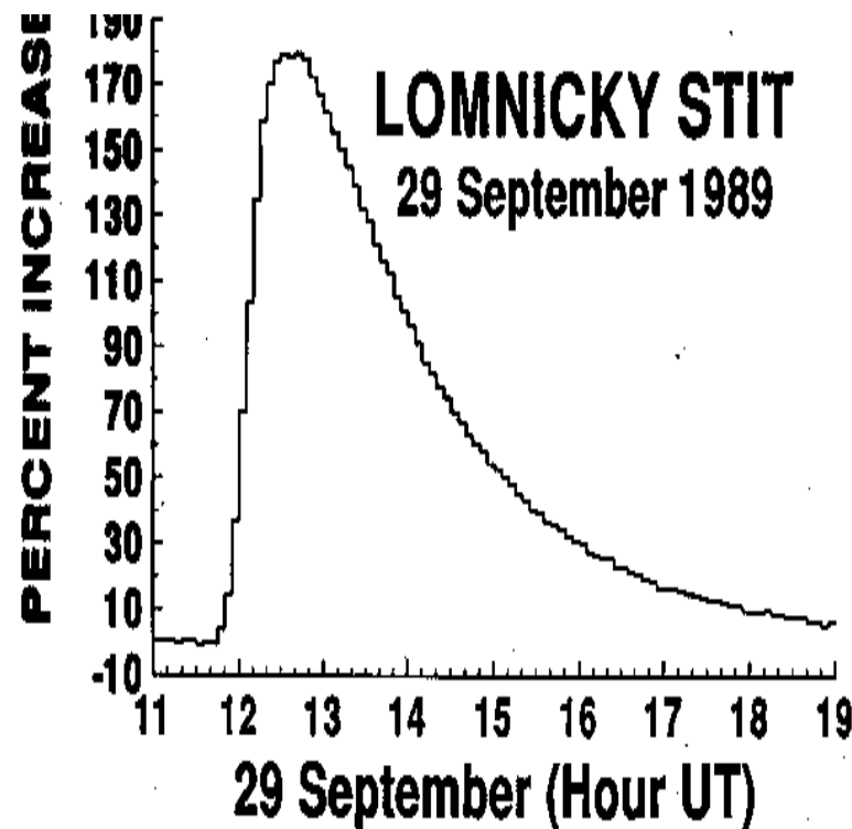
The largest increase from GLE observed at Lomnický Štít (since 1958)
