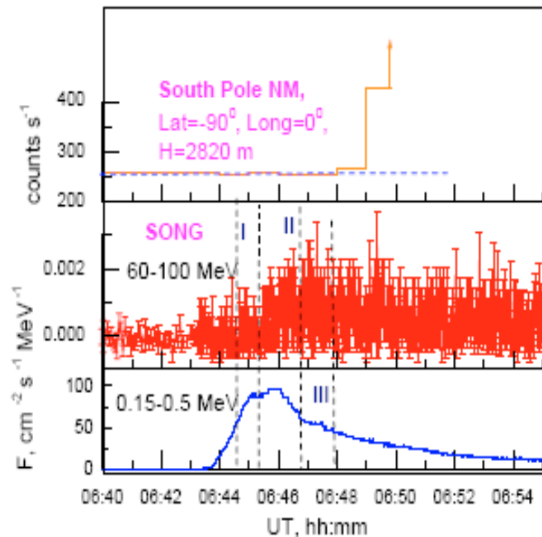
Figure 2. The temporal profile of measurements at two gamma ray channels of SONG along with the onset of GLE observed on South Pole NM.
