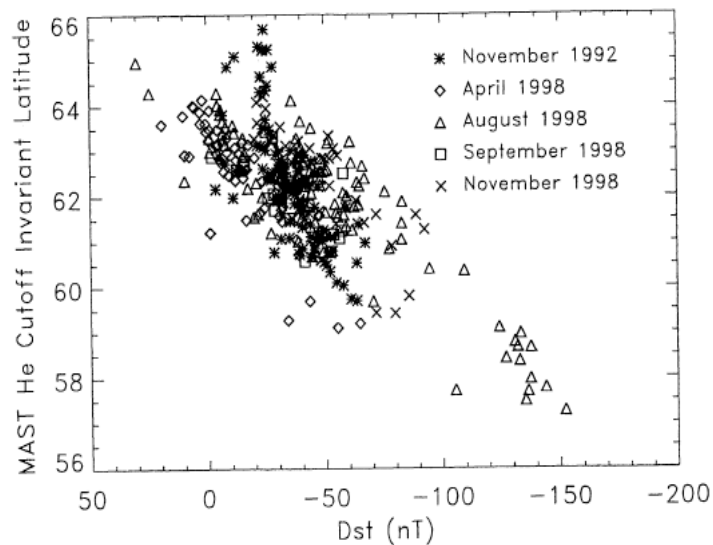
. Orbit-averaged cutoff invariant latitude for \sim 8-15 MeV/nucleon He plotted versus Dst interpolated to the same time as the cutoff measurement, for the five time periods indicated.
