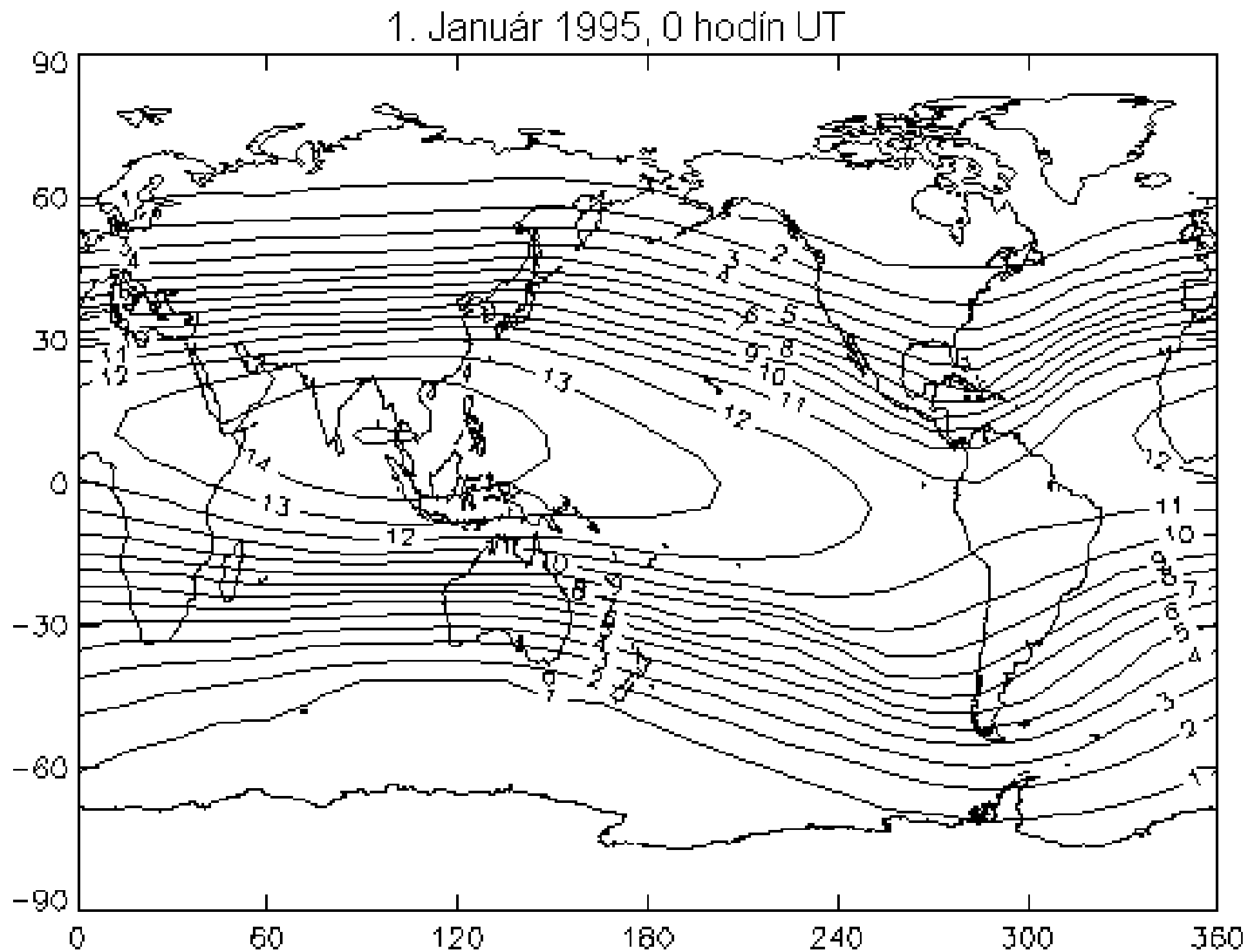
Map of vertical cut-off rigidities computed for AMS with Ts'89 external field, lowest geomagnetic activity level, from grid 5 x 15 degrees (lat x long), (Bobík, P., PhD thesis, 2001)
