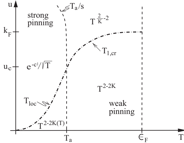
Abbildung 1. u - T phase diagram of the linear conductivity of disordered Luttinger liquids. For strong pinning, u > u_c \sim k_F(k_F a)^{K-1} and T < T_{1,cr} \sim T_a(u/u_c)^{1/(1-K)} , T_a/s separates the variable range hopping from the single impurity hopping regime. For T > T_{1,cr} impurities become weak. For weak pinning, u < u_c , T_{loc} \sim T_a(u/u_c)^{2/(3-2K)} separates variable range hopping from renormalized power law behavior. For T > T_a the power law is unrenormalized.
