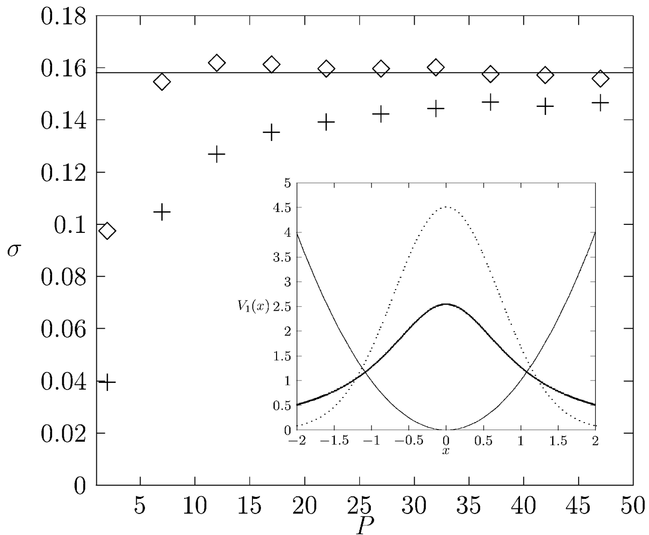
Figure 2: Delocalization \sigma of the harmonic oscillator for various number of beads, generalized (in diamonds) and standard (in crosses). Continuous line is exact quantum result for standard deviation, calculated using Eq. (13). Inset shows probability density for harmonic potential
