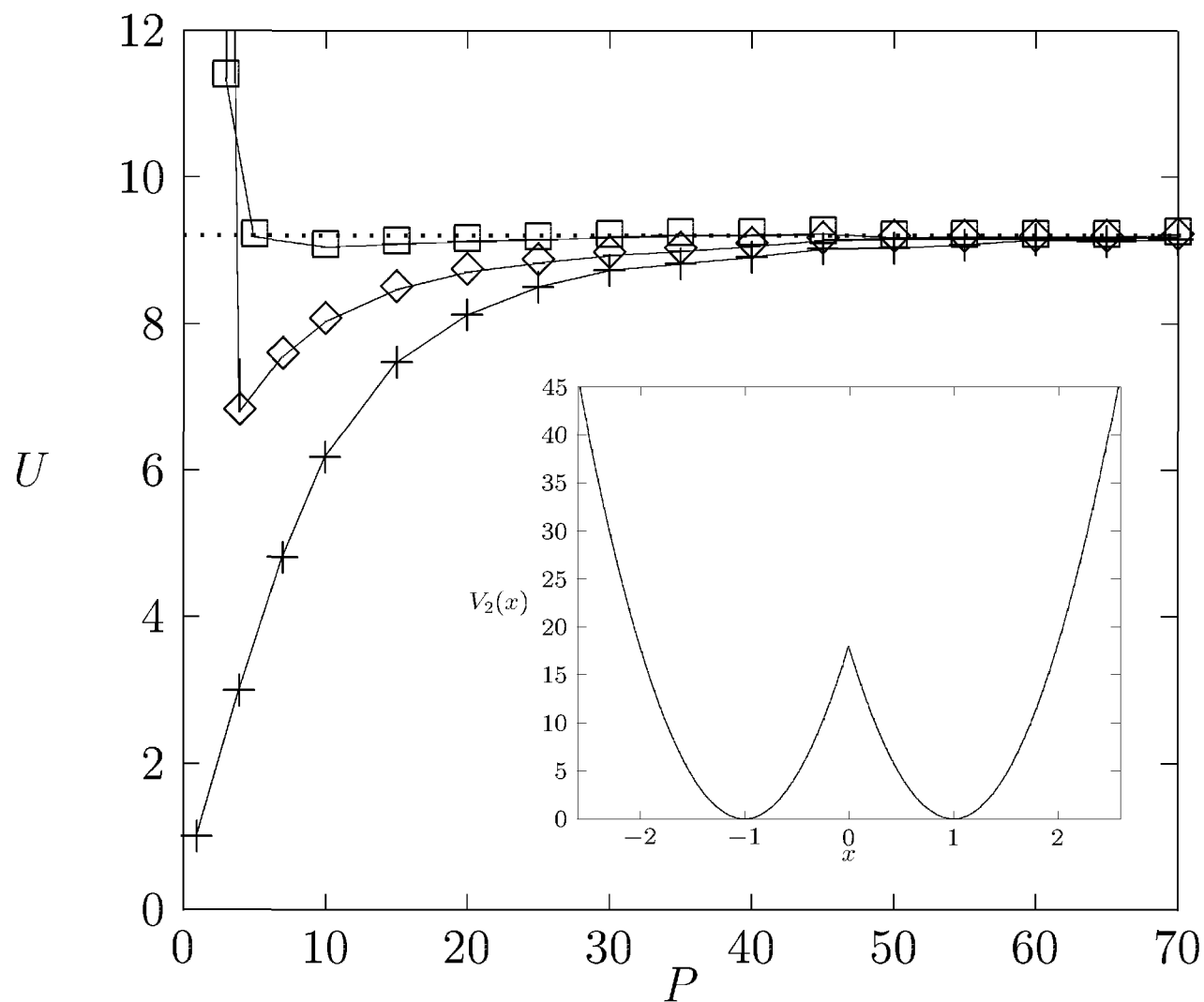
Figure 4: Internal energy of the double oscillator, as a function of the number of beads, with a = 0.4 , kT = 1 , \hbar\omega = 20 . The generalized algorithm results are shown in diamonds ( \alpha = 1 ) and squares ( \alpha = 0.6 ), the ones obtained using the standard primitive algorithm are in crosses.
