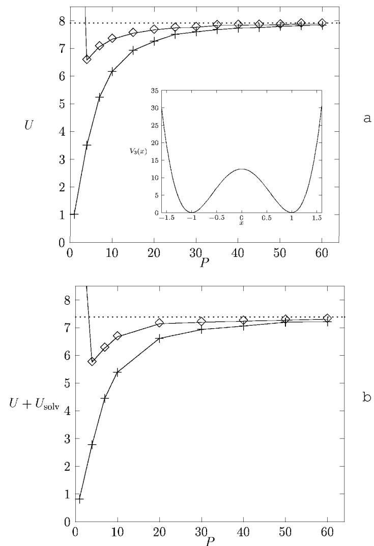
Figure 6: Internal energy of isolated bistable system (a) and in fluctuating adiabatic solvent (b). Exact results are shown with dotted line. When solvent considered, averaged over 500 Gaussian random values of S and run for 200,000 MC sweeps at each value of S . The inset shows
