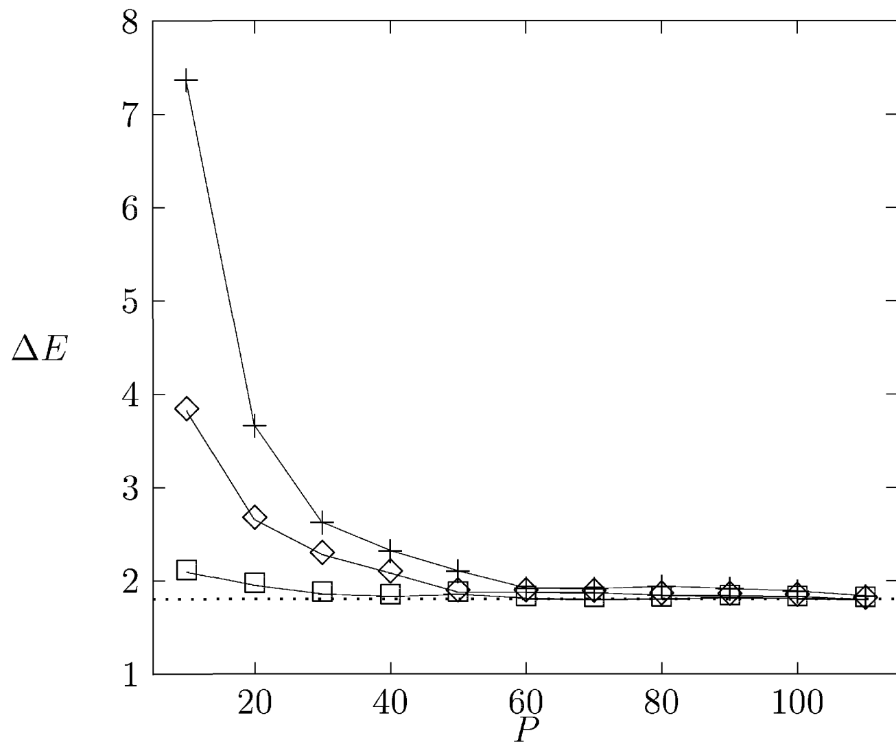
Figure 5: Tunnel splitting for the standard algorithm (in crosses), and the generalized algorithm ( \alpha = 1 in diamonds, and \alpha = 0.6 in squares), together with the exact splitting \Delta E = 1.78 (dotted line) calculated from eigenvalues of Schrödinger equation.
