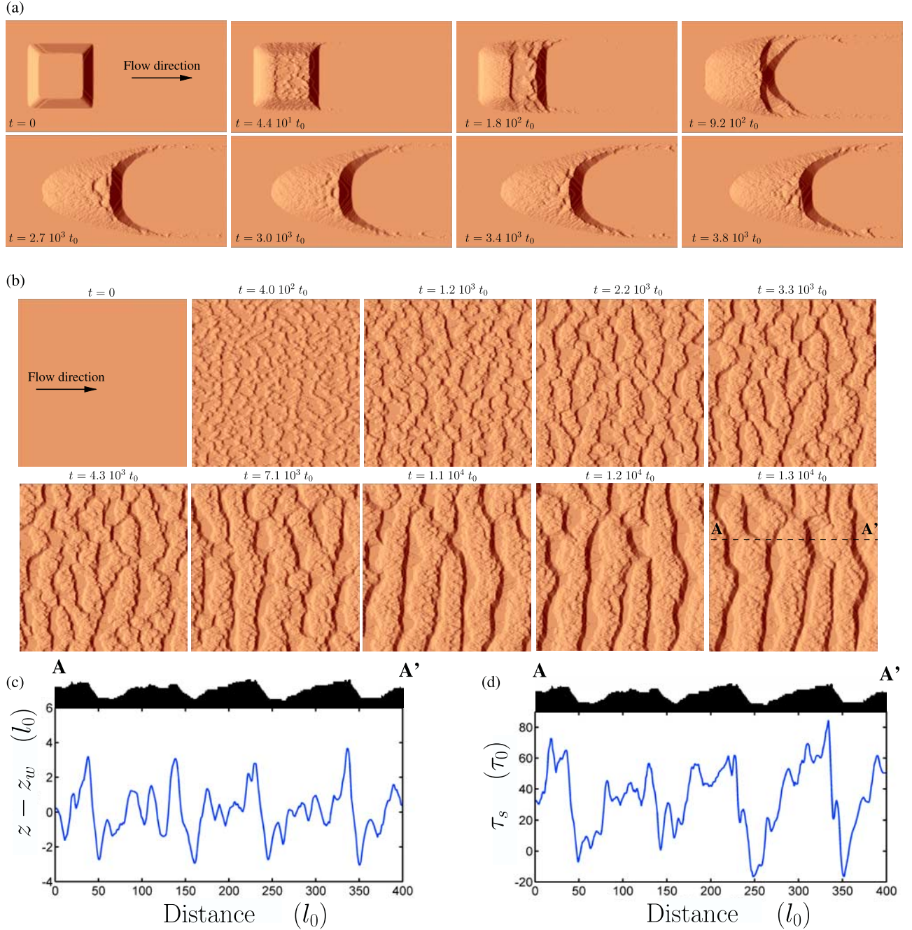
Figure 4. (a) Evolution of a square sand pile until a crescentic barchan shape reaches a quasi-stationary equilibrium state ( H = 100 l_0 , L = 600 l_0 ). (b) Formation of a transverse dune field until it reaches a quasi-stationary equilibrium state ( H = 100 l_0 , L = 400 l_0 ). The average number of dunes, defects, and terminations are almost constant despite some random fluctuations. In Figures 4a and 4b, \tau_1 = 20 \tau_0 . Note the characteristic length scales for the nucleation of dunes over short time and the formation of secondary bed forms over long time. (c) Along a transect line parallel to the direction of the flow (see AA' in Figure 4b), the difference between the elevation z and the local mean elevation z_w averaged over a sliding window of length 40 l_0 . (d) The bed shear stress at the solid fluid interface along the same transect line. In Figures 4c and 4d, the elevation profile is shown in black at the top of the graph.
