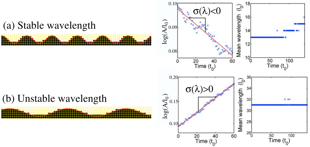
Figure 5. Linear stability analysis in the model with examples of (a) stable and (b) unstable wavelengths. As shown on the left, the initial condition at t = 0 is a flat sand bed disturbed by a sinusoidal wave of wavelength \lambda ( \lambda = 13 l_0 (Figure 5a); \lambda = 31 l_0 (Figure 5b)). The solid line is the continuous profile from which the initial bed profile h(\lambda, x, 0) has been discretized. The autocorrelation function of the bed profile C(\lambda, l, t) = \langle h(\lambda, x, t)h(\lambda, x + l, t) \rangle - \langle h(\lambda, x, t) \rangle^2 gives the amplitude A(\lambda, t) = 2\sqrt{2C(\lambda, 0, t)} and the mean wavelength (the position of the first peak). Assuming a linear regime, A(\lambda, t) is fitted by an exponential function of the form \exp(\sigma(\lambda)t) during the period over which the mean wavelength remains unchanged. If \sigma(\lambda) > 0 , the wavelength is unstable and the pattern is growing; if \sigma(\lambda) < 0 , the wavelength is stable and the pattern is decaying. The most unstable wavelength \lambda_{\max} is the wavelength at which \sigma(\lambda) reaches a maximum.
