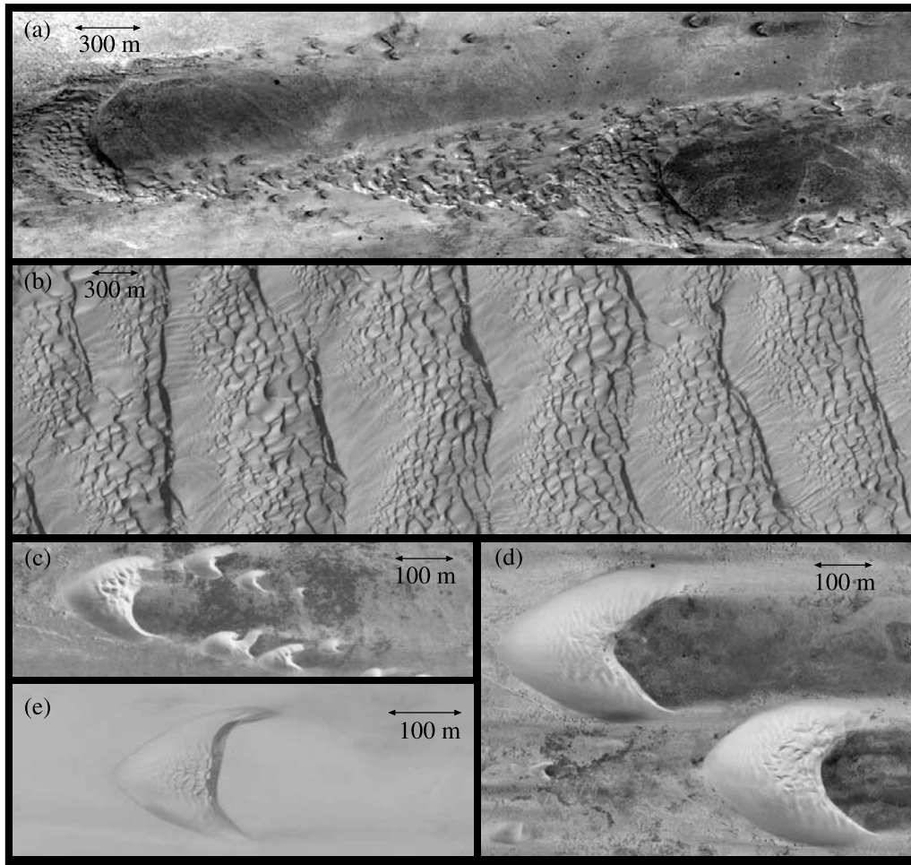
Figure 1. Observations of superimposed dune patterns in nature for (a) megabarchans in Peru ( 6^{\circ}08'47.39''\text{S} 80^{\circ}50'25.47''\text{W} ), (b) transverse dunes in Namibia ( 26^{\circ}6'26.21''\text{S} 15^{\circ}00'23.90''\text{W} ), (c) barchan dunes in Morocco ( 27^{\circ}32'49.52''\text{N} 13^{\circ}12'40.15''\text{W} ), (d) barchan dunes in Morocco ( 21^{\circ}36'51.45''\text{N} 16^{\circ}46'09.86''\text{W} ), and (e) isolated barchan in Peru ( 9^{\circ}5'0.58''\text{S} 78^{\circ}30'39.85''\text{W} ).
