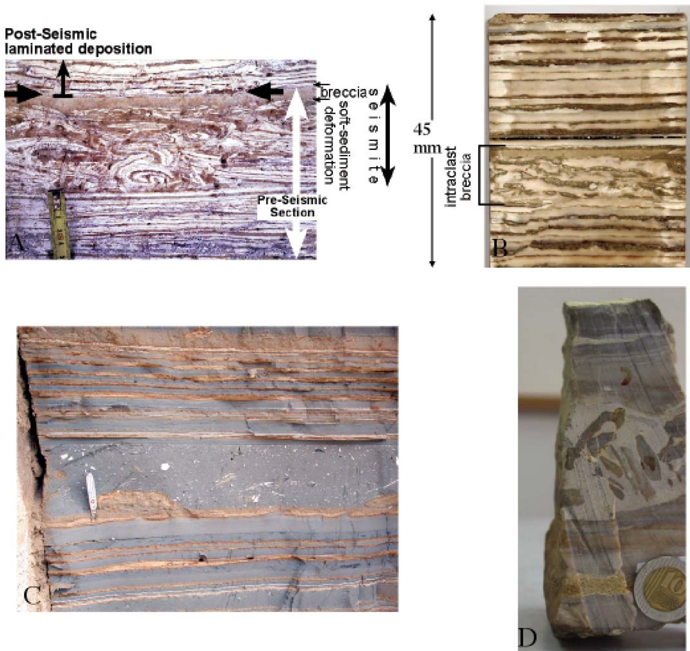
Figure 2. Selected photos of intraclast breccias. (A) An intraclast breccia juxtaposed with an intraformational fault, Lisan Peninsula. (B) A micrograph of a section from the Ein Gedi core. The lowest centimeter displays an undisturbed sequence consisting of six cycles of alternating detritus and aragonite. On top of this sequence, a 1-cm-thick intraclast breccia layer comprises torn laminae of aragonite as well as detritus, topped with a millimeter of fine breccia with mixed components. The intraclast breccia layer is topped in turn by twelve cycles of alternating detritus and aragonite. (C) An intraclast breccia layer identified with the 31 B.C. earthquake (Ken-Tor et al., 2001a, 2001b). (D) An intraclast breccia from Campanian chert, near the Dead Sea rift (photo by Y. Kolodny). Kolodny et al. (2005) point out to the similarity in texture with Lisan Formation breccias and suggest a similar mechanism of formation.
