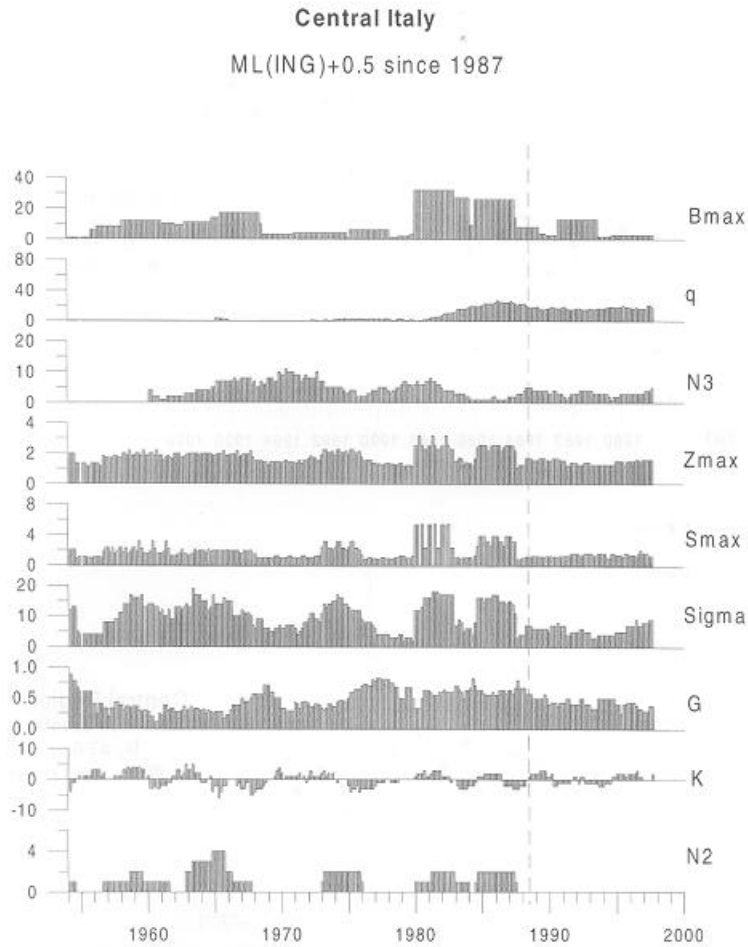
Figure 5. Time diagrams of the CN functions obtained for the Central region using the 'corrected' catalogue, in which the quantity D=0.5 is added to M_L(ING) beginning in 1987.
