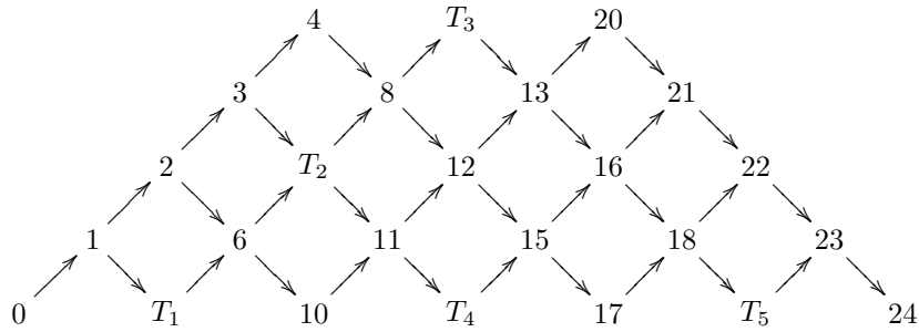
FIGURE 3. A cluster-tilting set in A_5
