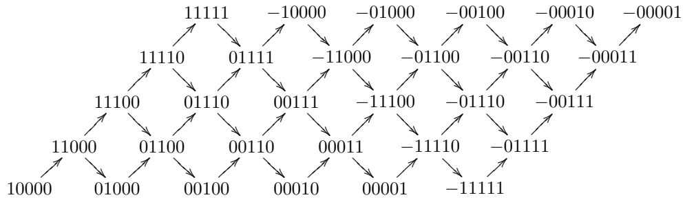
FIGURE 2. Some dimension vectors of indecomposables in \mathcal{D}_{\vec{A}_5}
