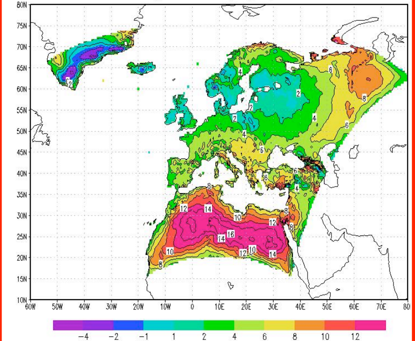
T2m RegCM4-CRU (deg C) JF 1989
