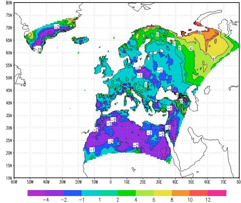
T2m RegCM4-CRU (deg C) JF 1989
