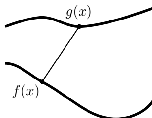
FIGURE 4.1. Straight-line homotopy.
