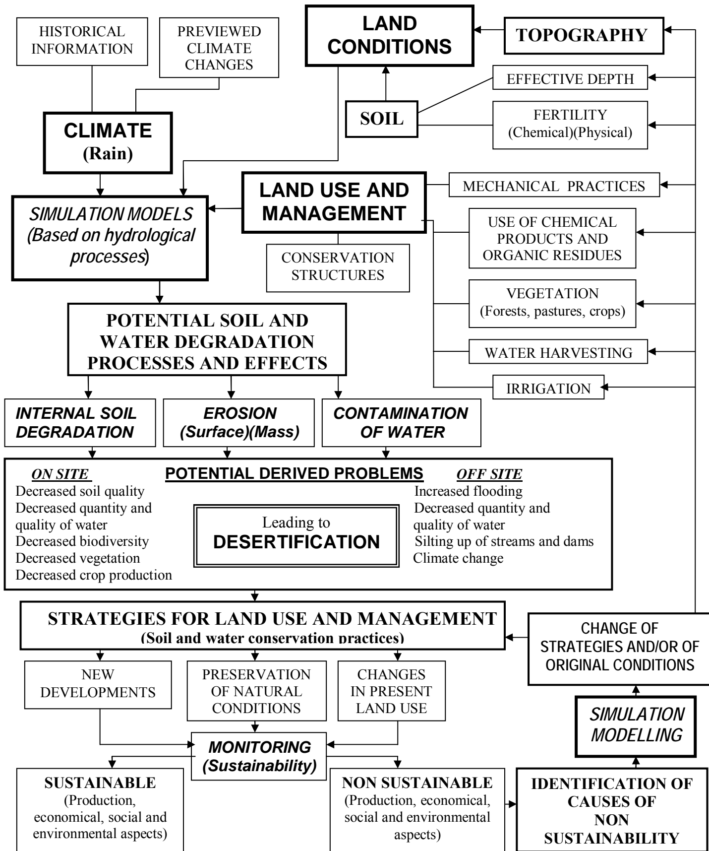
Figure 3. Role of simulation modelling based on hydrological processes (see figures 1&2) for evaluating potential soil and land degradation and desertification, and for planning land use, management and soil and water conservation practices (adapted from: Pla, 1991; 2002b)
