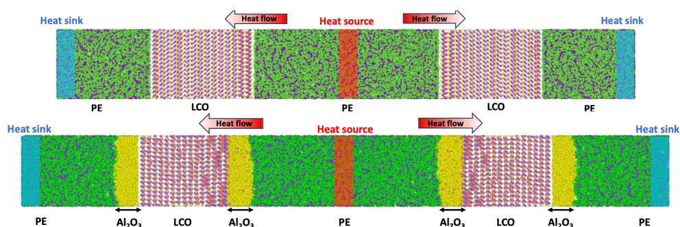
Schematic of heat flow across PE/LCO and PE/ \text{Al}_2\text{O}_3 /LCO interfaces
