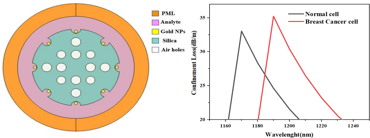
Fig. 1: (a) Cross sectional view of the reported PCF; (b) Spectral variation of CL for normal and cancer cells.
