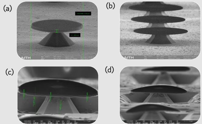
Fig: (a),(b) SEM images of the microdisks of 5µm, 20µm diameter, 300nm thick, and (c),(d) 7.5µm diameter, 100nm thick
