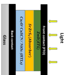
Fig. 1. Solar cell structure used in the simulation.
