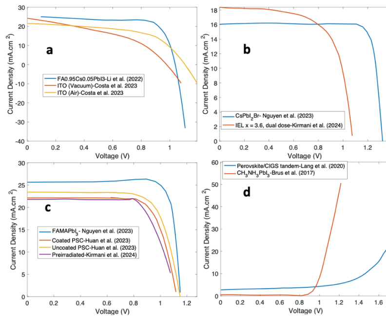
Figure 1: J-V curve for different proton irradiation effect on solar cell
