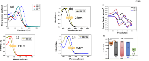
Fig.1. Absorption spectra of MD1-MD3 dyes dissolved in THF (a) and on mesoporous TiO 2 film (b, c, d)
