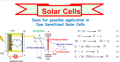
Scheme 1. Electron transformation mechanism in DSSCs
