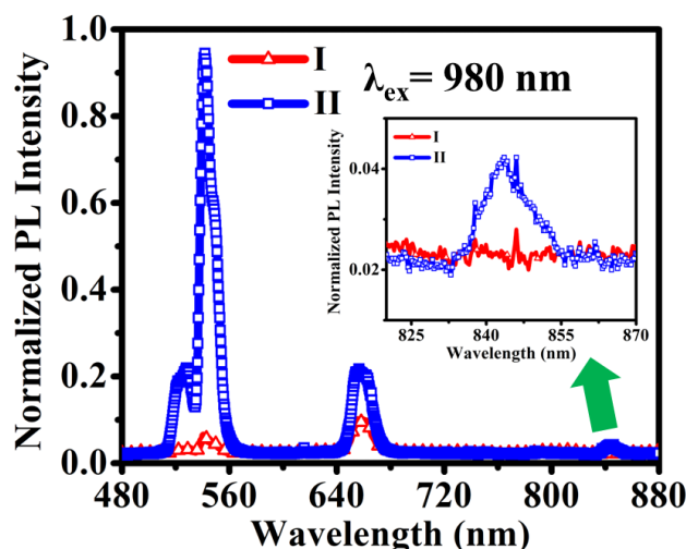
Figure 1: Upconversion photoluminescence of (I) \text{NaYF}_4:\text{Er}^{3+}/\text{Yb}^{3+} and (II) \text{NaYF}_4:\text{Er}^{3+}/\text{Yb}^{3+}/\text{Cr}^{3+}(15\%) nanophosphors under fs laser excitation at 980 nm. Inset shows an expanded representation between 820 nm to 870 nm.
