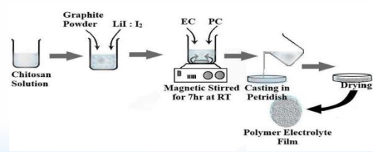
Preparation of Polymer electrolyte via solution cast technique
