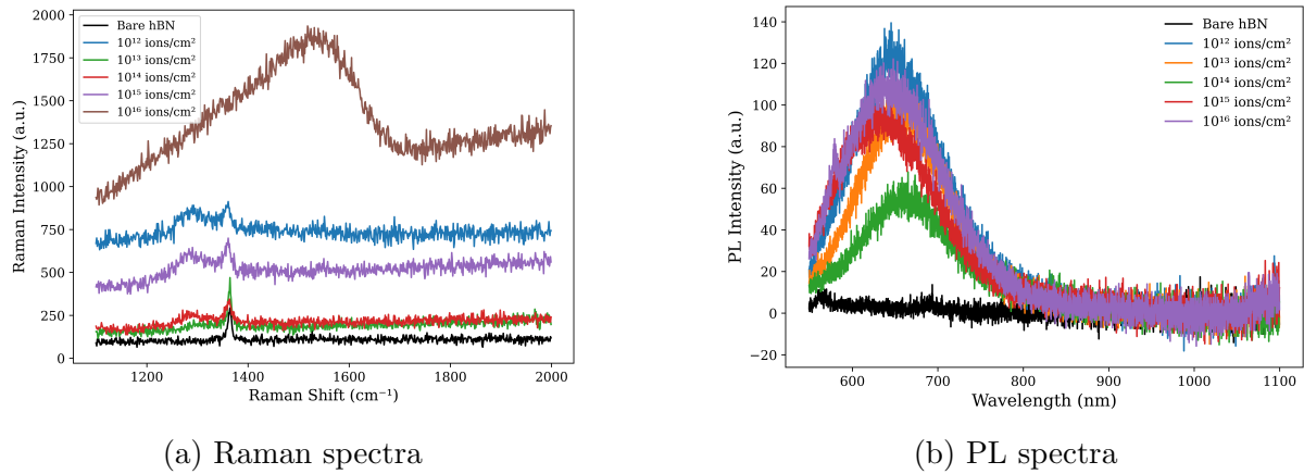
Figure 1: Raman and PL comparison for bare and ion-implanted hBN.
