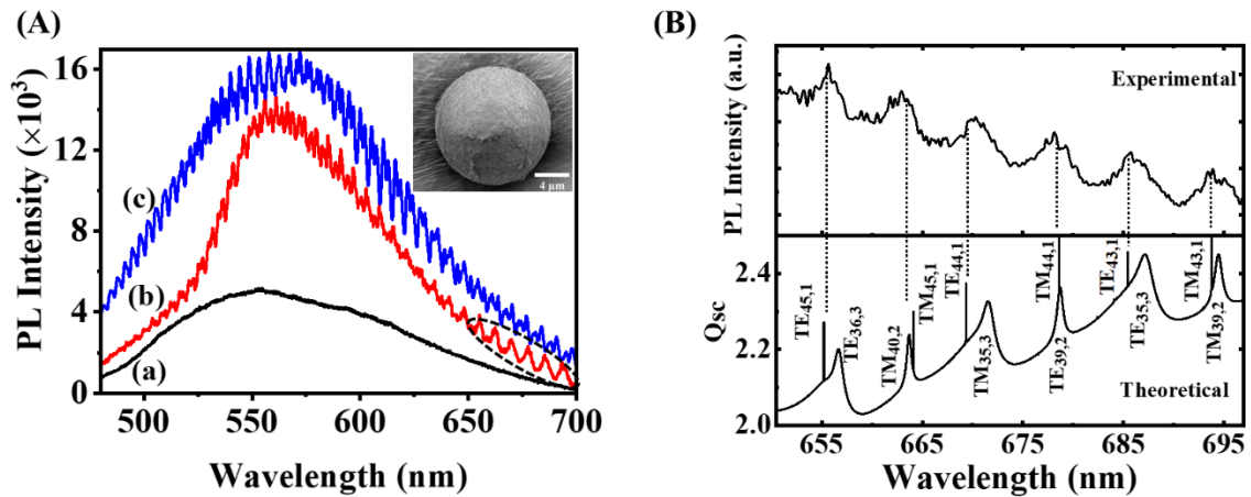
Figure 1. (A) PL of (a) hBN QDs, and hBN QDs coupled PST microspheres of radii (b) \sim 3 \mu\text{m} , and (c) \sim 7 \mu\text{m} . Inset shows the scanning electron microscope image of QDs coupled PST microsphere, and (B) theoretical fitting (bottom panel) of WGMs for a part of PST microsphere (encircled portion in Panel A). From the fitting, the radius ( r ) of the PST microsphere is determined as \sim 3.3845 \mu\text{m} . The dotted lines are guide to the eye.
