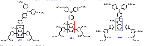
Scheme 2. Molecular structure of MD dyes
