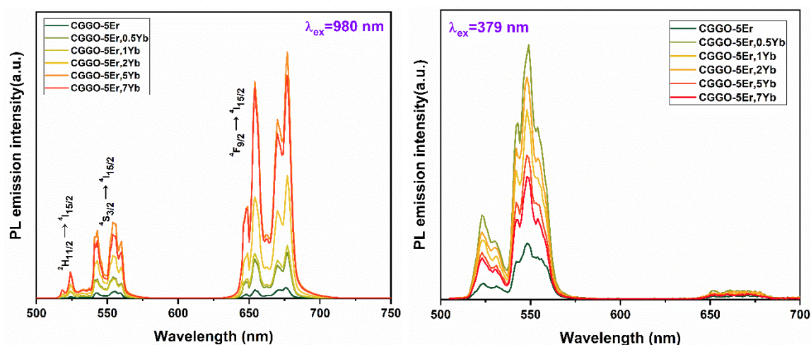
Figure A: (a) Upconversion (b) downconversion of CGGO-5Er, x%Yb
