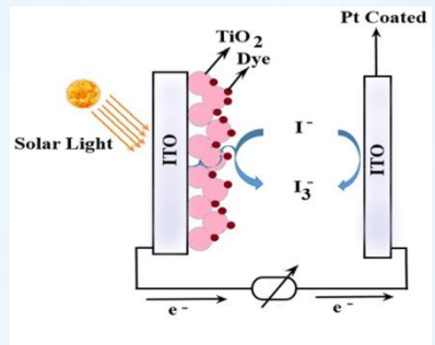
Major Components Of Dye Sensitized Solar Cell
