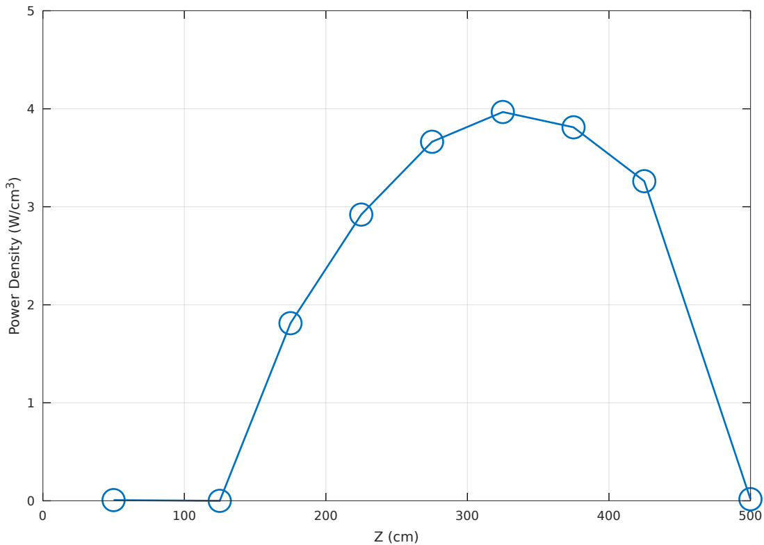
Axial Power Distribution in the Central Channel
