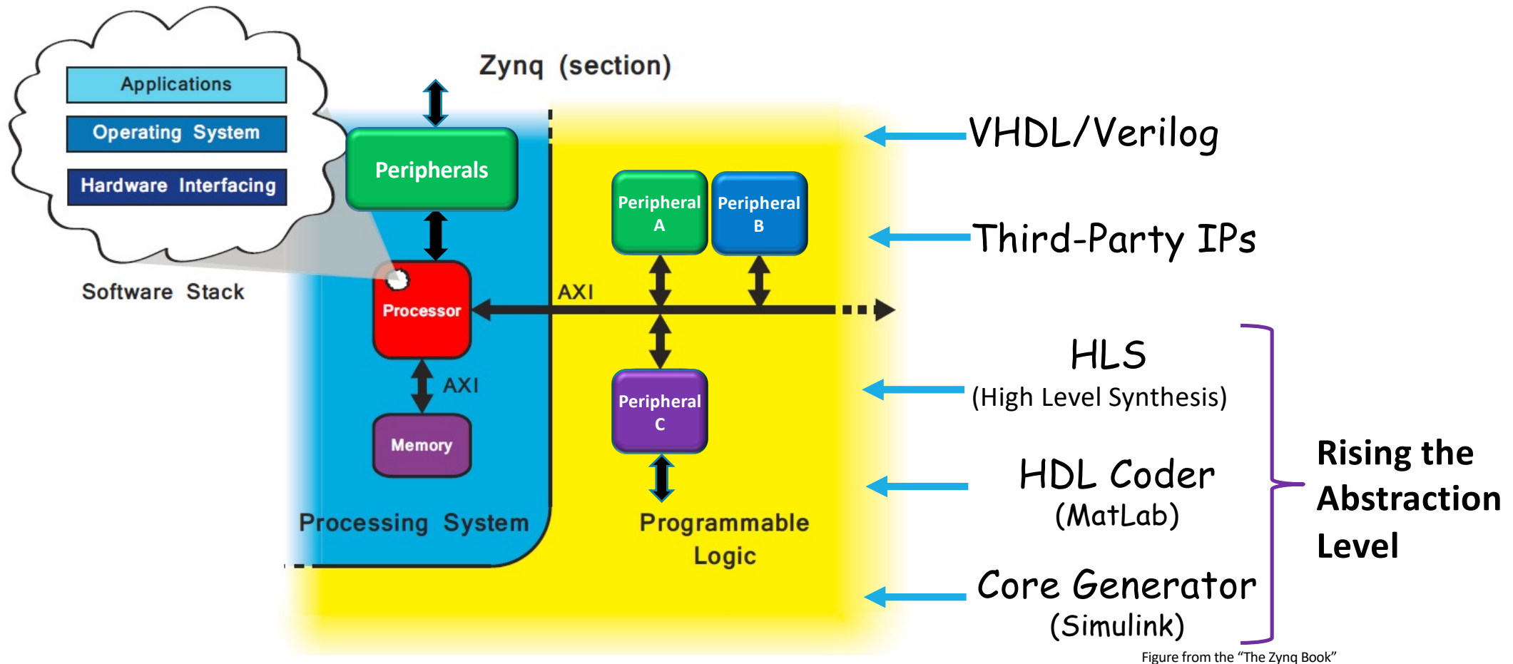
Figure from the "The Zynq Book"
