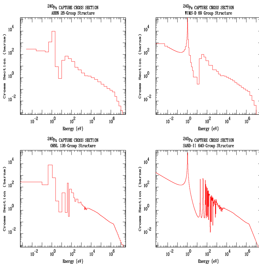
Figure 2. ^{240}\text{Pu} radiative capture cross section from the ENDF/B-VI evaluated data library represented in various group structures.
