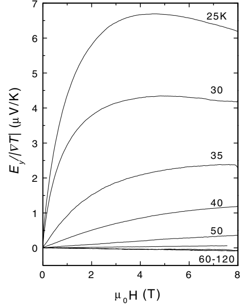
FIG. 5. Variation of E_y / |\nabla T| vs. H in \text{Bi}_2\text{Sr}_{2-y}\text{La}_y\text{CuO}_6 (Sample B2 with y = 0.5 ) at temperatures 25 to 120 K. Compared with LSCO, the curves display more pronounced curvature at temperatures high above T_c .
