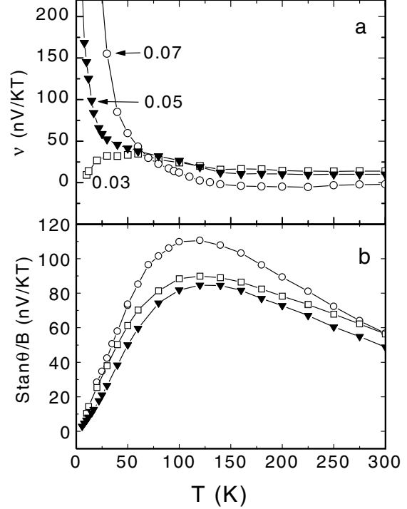
FIG. 3. (a) The T dependence of \nu in very underdoped LSCO (Samples L1, L2, L3, with x = 0.03 , 0.05 and 0.07, respectively). At low T , the different behaviors of \nu in L1 (compared with L2 and L3) indicate distinct origins of the Nernst signal. In L1 (open squares), \nu is entirely from the carriers, while in L2 and L3, it is from vortex-like excitations. The lower panel (b) displays S \tan \theta/B measured in L1-L3 (symbol association same as in (a)). Above 150 K, cancellation is nearly complete between the two normal-state currents, S \tan \theta/B and \alpha_{xy}^n . At lower T , however, a significant residual \nu_N is observed especially in L1.
