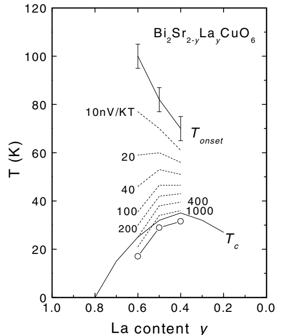
FIG. 10. The y dependence of T_\nu and the contours of the vortex-like Nernst signal in \text{Bi}_2\text{Sr}_{2-y}\text{La}_y\text{CuO}_6 determined from \nu - \nu_N using the procedure of Xu et al. [7]. The solid line for T_c is from Ono et al. [11] (open circles are T_c measured in B1-B3). The contours bear a strong resemblance to those in LSCO (Fig. 9).
