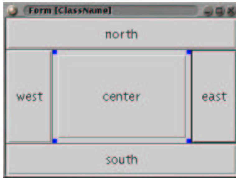
Figure 7.6: The BorderLayout
