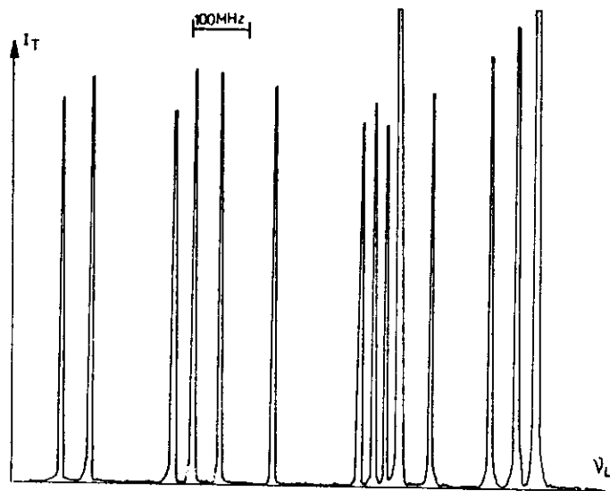
Fig.10.41. Polarization spectrum of the hfs components of the R(98), 58 - 1 line of I 2 at 514.5 nm (compare with Fig.10.23)
