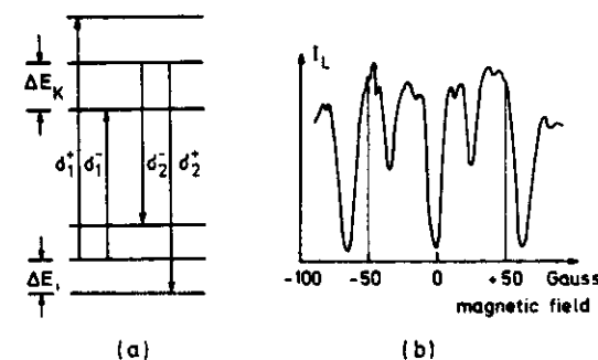
Fig. 10.32a,b. Three-level laser spectroscopy with a multimode laser and Zeeman scanning. (a) Level scheme, (b) resonances in the laser output as a function of the magnetic field [10.47]
