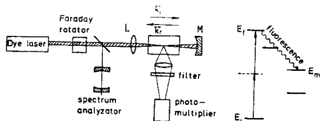
Fig. 10.49. Experimental arrangement for the observation of Doppler-free two-photon absorption
