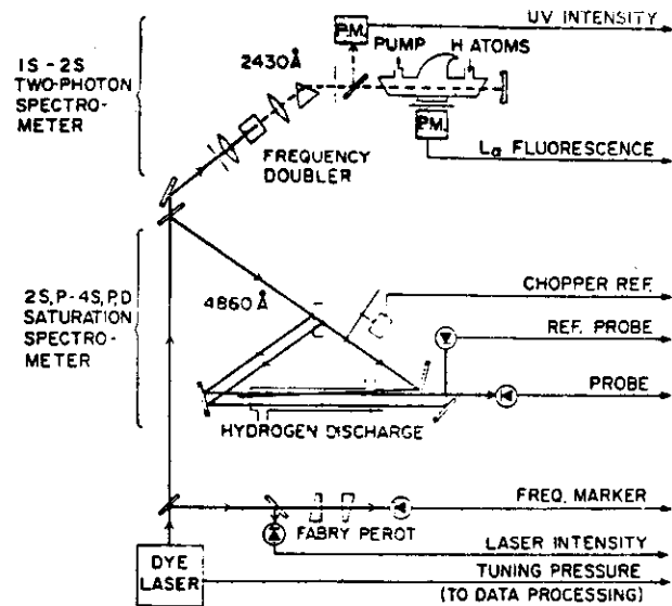
Fig.10.55. Experimental setup for the determination of hydrogen 1S Lamb shift by combination of saturation and two-photon spectroscopy [10.78]
