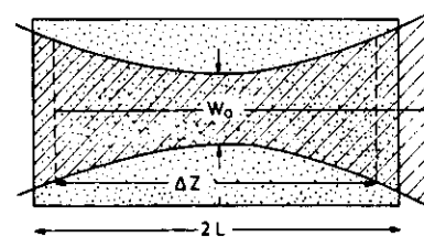
Fig.10.52. Optimum focussing with \Delta z = 2L gives maximum signals in two-photon spectroscopy
