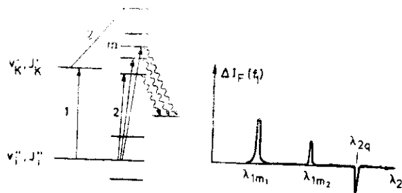
Fig. 10.12. Labeling of specified upper or lower levels ( v, J ) by optical pumping and successive probing (optical-optical double resonance)
