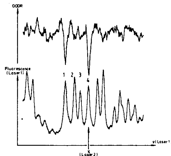
Fig. 10.14. Section of linear \text{NO}_2 spectrum around \lambda = 488 \text{ nm} (lower trace) and double-resonance spectrum (upper trace). The pump laser was stabilized on line No. 4 while the probe laser was tuned [10.26]
