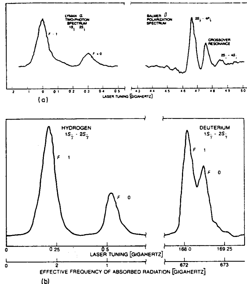
Fig.10.56. (a) Simultaneous measurement of the 1S \rightarrow 2S transition and the Balmer \beta line ( 2S - 4P_{1/2} ) of the H atom. (b) Hfs of the 1S_{1/2} \rightarrow 2S_{1/2} transition in hydrogen and deuterium, resolved with two-photon spectroscopy [10.31a]
