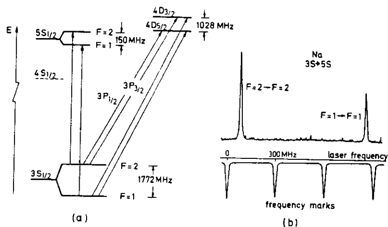
Fig. 10.53. (a) Level scheme of the Na atom. The hfs splitting is not to scale. (b) Two-photon transitions 3s \rightarrow 5s with frequency markers from an F.P.I. with d = 25 cm [10.74]
