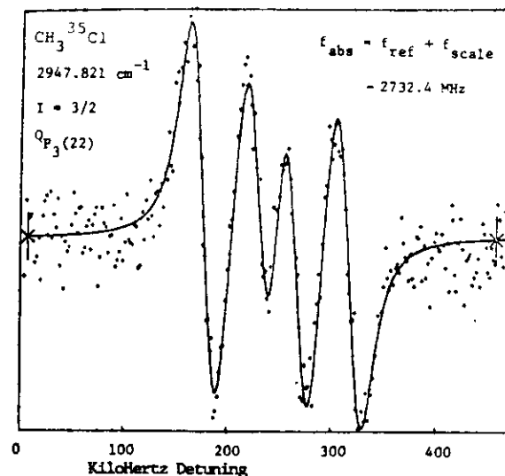
Fig.10.26. Saturated absorption spectrum of \text{CH}_3^{35}\text{Cl} at \lambda = 2947.821 \text{ cm}^{-1} . The spectrum represents the derivative of four hfs components of the Q_P(22) rotational line [10.40]
