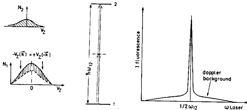
Fig.10.51. Schematic illustration of Doppler-free two-photon signal with Doppler-broadened background. The background amplitude is greatly exaggerated
