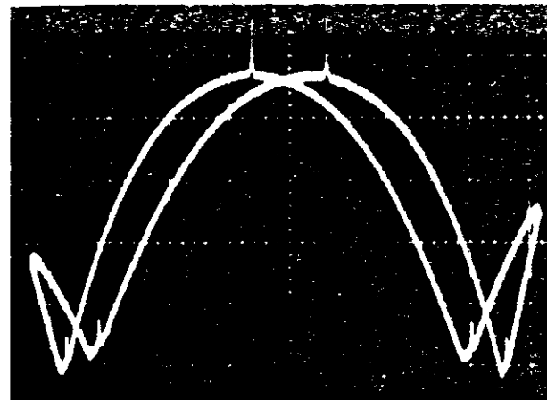
Fig.10.25. Saturation peak in the output of a He-Ne laser at \lambda = 3.39 \mu m caused by the Lamb dip of a CH_4 absorption line [10.43]. The laser frequency was swept twice over the gain profile
