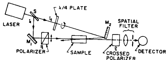
Fig.10.34. Schematic experimental arrangement for polarization spectroscopy [10.57]
