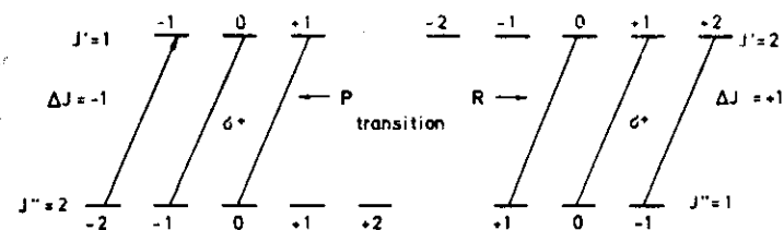
Fig.10.35. Selective depopulation of different M'' sublevels and selective population of different M' sublevels by optical pumping with circularly polarized \sigma^+ light
