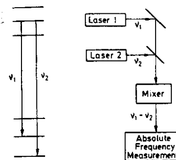
Fig.10.48. Schematic diagram of heterodyne spectroscopy using two stabilized lasers
