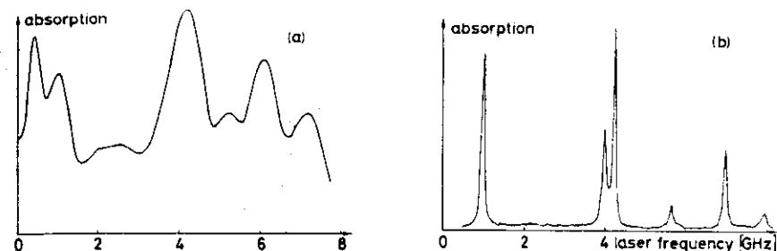
Fig.10.3a,b. Section of the excitation spectrum of the \text{Cs}_2 molecule in the spectral range around \lambda = 476.5 \text{ nm} . (a) Excited in a cesium vapor cell, (b) excited in a collimated cesium beam
