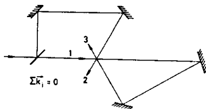
Fig. 10.50. Possible arrangement for Doppler-free three-photon spectroscopy
