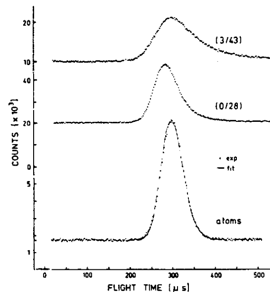
Fig.10.11. Time-of-flight spectrum of \text{Na}_2 molecules in two different quantum states ( v''=3, J''=43 ) and ( v''=0, J''=28 ) in comparison with the Na atom velocity distribution [10.24]
