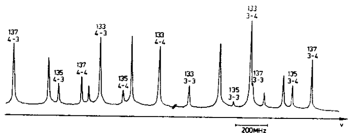
Fig. 10.22. Survey scan of the saturation spectrum of all hfs components of the 6^2S_{1/2} \rightarrow 7^2P transition at \lambda = 459.3 nm in a vapor mixture of Cs 133, 135, and 137 [10.32]
