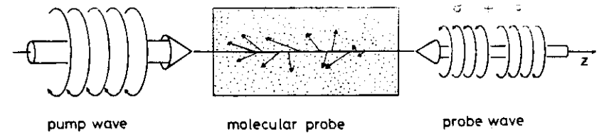
Fig.10.36. Schematic illustration of partial alignment of angular momenta by the left-hand circularly polarized ( \sigma^+ ) pump wave, which results in different absorption coefficients for \sigma^+ and \sigma^- probe light
