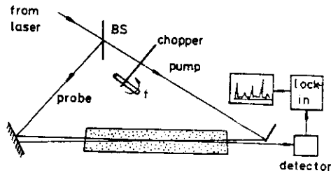
Fig.10.20. Possible experimental arrangement for saturation spectroscopy outside the laser resonator
