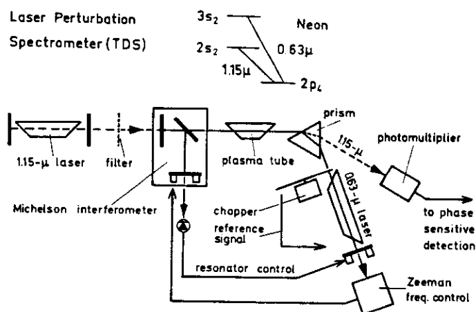
Fig.10.33. Optical-optical double resonance of two coupled Ne laser transitions studied in a tuned differential laser spectrometer [10.50]
