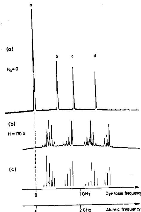
Fig. 10.54a-c. Zeemann effect of the 3S-4D transition in Na. (a) hfs with zero magnetic field, (b) Zeeman pattern at 170 Gauss, (c) calculated positions and intensities of the Zeeman components for \Delta M = 2 transitions [10.74]
