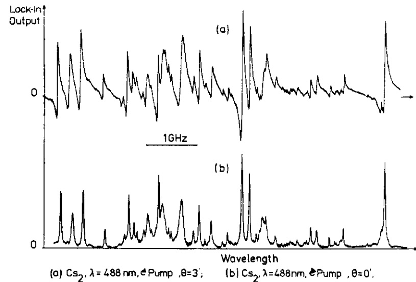
Fig. 10.38a,b. Two identical sections of \text{Cs}_2 polarization spectra obtained with circular pump polarization and linear probe polarization, but different uncrossing angles \theta of the two polarizers [10.59]
