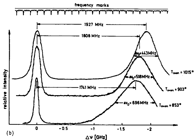
Fig.10.6a,b. Doppler shift laser spectroscopy of the velocity distributions of \text{Na}_2 molecules and their dependence on the vapor pressure p(T) in the oven. (a) Experimental arrangement, (b) velocity distributions n(v, v''=0, J''=28) of molecules in the vibrational level v''=0 and rotational level J''=28 at three different oven temperatures [10.17]
