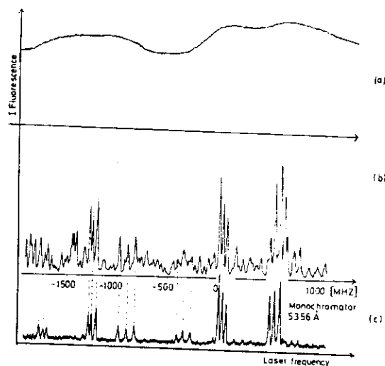
Fig.10.4a-c. Section of the excitation spectrum of \text{NO}_2 obtained with a single-mode argon laser, tunable around \lambda = 488 \text{ nm} . (a) In an \text{NO}_2 cell ( p = 0.01 \text{ torr} ), (b) in a collimated \text{NO}_2 beam with a collimation ratio of 1:80, (c) filtered excitation spectrum. Instead of the total fluorescence as in (b) only the (0,1,0) fluorescence band was monitored
