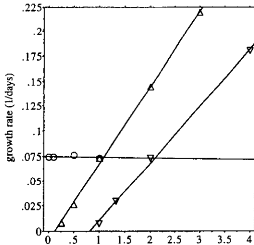
FIG. 11. Estimated growth rates in the coupled model as a function of model parameters: \Delta indicates the values of r_e^{-1} (days), O indicates the values of \partial_z \bar{T}_{sub} ( ^{\circ}\text{C m}^{-1} ), and \nabla indicates the values of H_1^{-1} \times 10^2 (m). Fitted data using linear regression is shown by solid lines.
