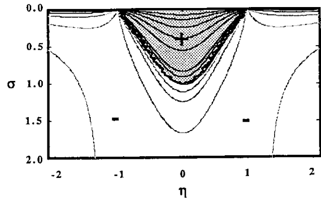
FIG. 3. Distribution of the refraction index l^2 = R(\eta, \sigma)/P(\eta, \sigma) as a function of \eta and \sigma . The shaded area is the region where the coupled instability could occur. This region is bounded by a curve P(\eta, \sigma) = 0 .
