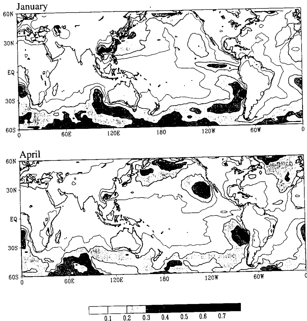
FIG. 3. The fractional stratus cloud cover, on the basis of ISCCP climatology, for January, April, July, and October; contour interval is 0.1.
