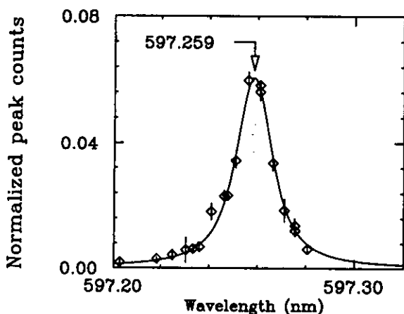
FIG. 11. Above: Time dependence of the delayed annihilation of antiprotons in \bar{p}\text{He}^+ induced by laser irradiation at 597.259 nm, and below: line-shape of the resonance (after Ref. 162).
