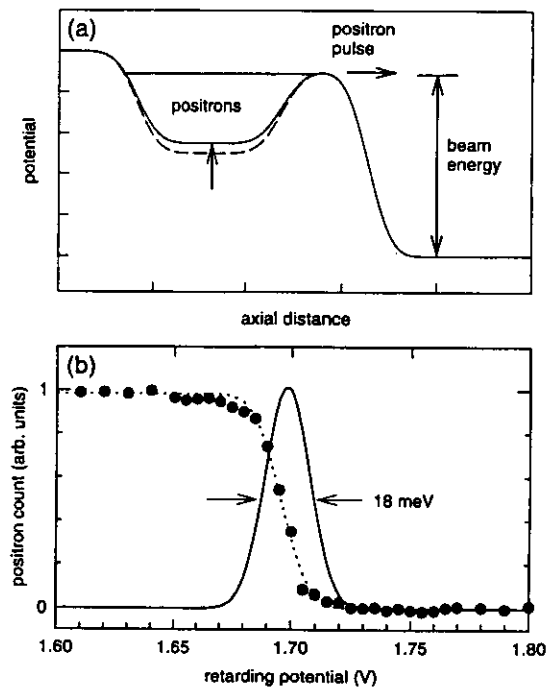
FIG. 10. (a) Electrostatic potential in a positron trap for producing cold pulsed beams of positrons. (b) Energy spread of a typical pulsed beam, measured using a retarding potential analyzer; ( \bullet ) number of positrons reaching the collector as a function of the retarding potential; dotted line: fitted error function; solid line: energy distribution function of the beam, calculated by differentiating the fit to the data.
