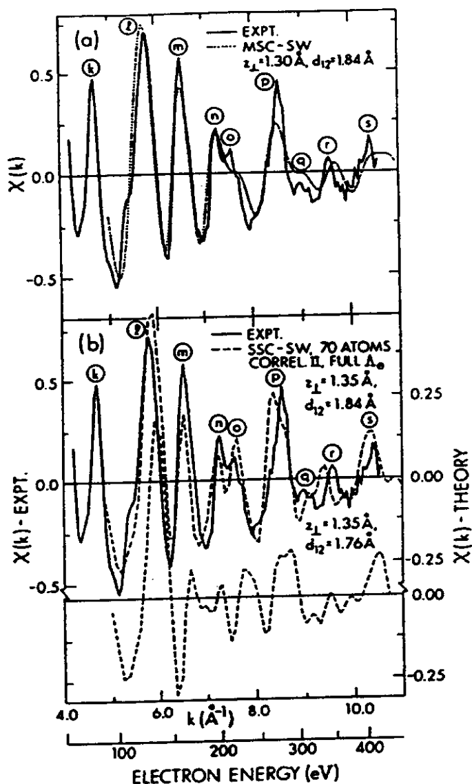
FIGURE 19. Comparison of scanned-energy S 1s data for c(2 \times 2) S on Ni (001), \theta_{\text{inc}} = 70^\circ , \theta_{\text{sc}} = 0^\circ (From Ref. 8) with: (a) a multiple-scattering cluster spherical-wave (MSC-SW) calculation due to Barton and Shirley (From Ref. 25), and (b) single-scattering cluster spherical wave (SSC-SW) calculations due to Sagurton et al. (From Ref. 21). Both the sulfur vertical distance z and the first Ni-Ni interplanar distance d_{12} are specified. (Fig. from Ref. 21.)
