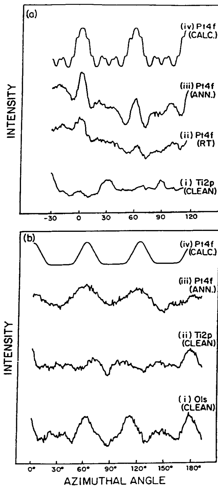
FIGURE 33. (a) Azimuthal XPD data for Pt 4f and Ti 2p emission from Pt on \text{TiO}_2(110) at \theta = 40^\circ are compared to PW cluster calculations including double scattering for Pt emission from a (111)-oriented metal cluster of about 15 \text{ \AA} diameter. Al K\alpha radiation was used for excitation. (b) As in (a) but for Pt 4f, Ti 2p, and O 1s emission from Pt on \text{TiO}_2(100) at \theta = 45^\circ . (From Ref. 120.)
