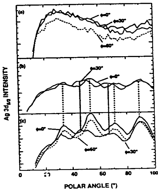
FIGURE 30. Polar XPD scans of Ag 3d_{5/2} intensity at 1120 eV from: (a) the (\sqrt{3} \times \sqrt{3}) Ag structure on Si (111) formed after annealing an \approx 1.3 -ML Ag overlayer to 550^\circ\text{C} ; (b) a Ag overlayer of approximately 2 ML average thickness at 450^\circ\text{C} ; and (c) a thick Ag overlayer of approximately 6 ML thickness at ambient temperature. (From Ref. 50.)
