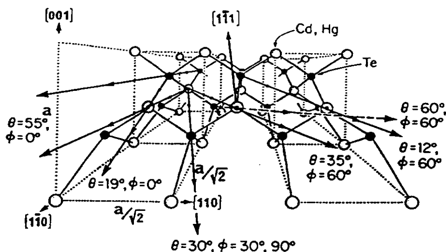
FIGURE 27. Perspective view of the unreconstructed (111) surface of \text{Hg}_{1-x}\text{Cd}_x\text{Te}(111) in the Model A surface termination of Fig. 26, with the \theta , \phi coordinates of various near-neighbor/low-index directions along which forward scattering might be expected to be strong. These directions would be the same for the unreconstructed (111) surfaces of any material with the zincblende or diamond structure, as will be used later in discussing Fig. 36.
