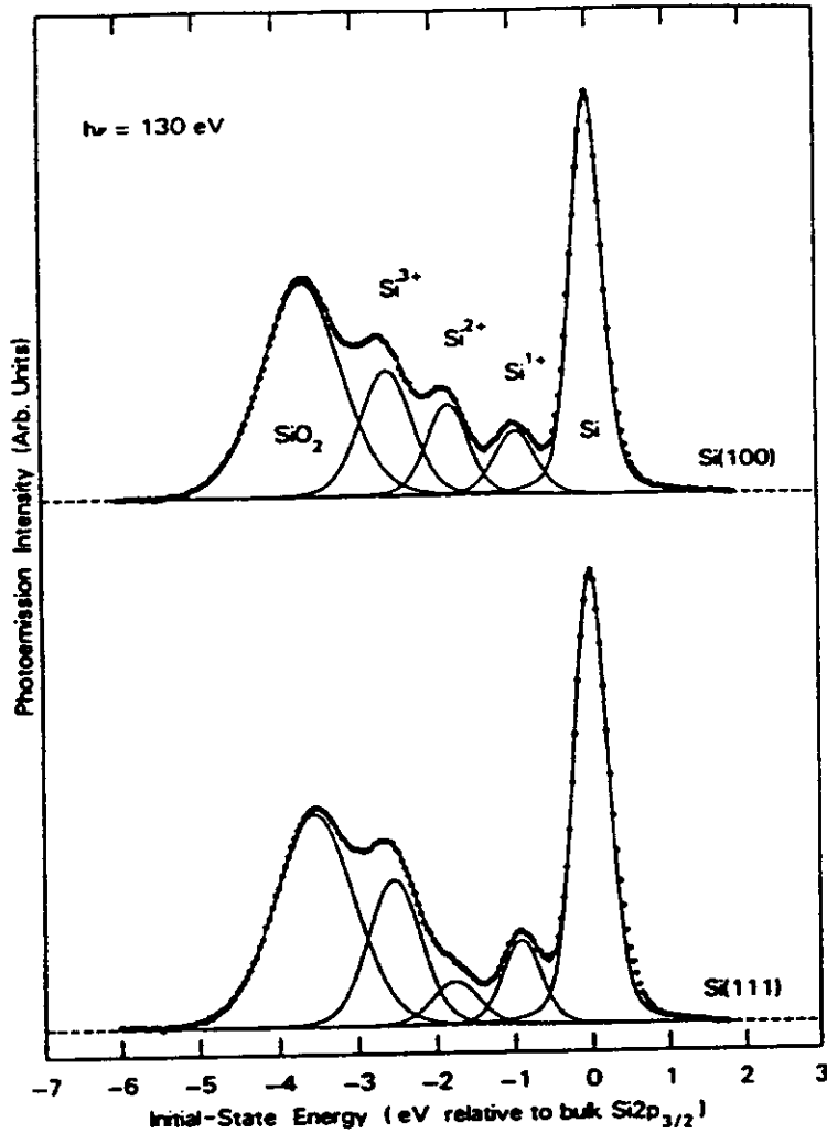
FIGURE 35. The Si 2p_{3/2} components of Si 2p spectra from thin oxide films of approximately 5 Å thickness thermally grown on Si (100) and Si (111) surfaces. Note the reduced intensity of Si 2+ for Si (111), assumed to be due to structural differences in the interface. [From Ref. 123(c).]
