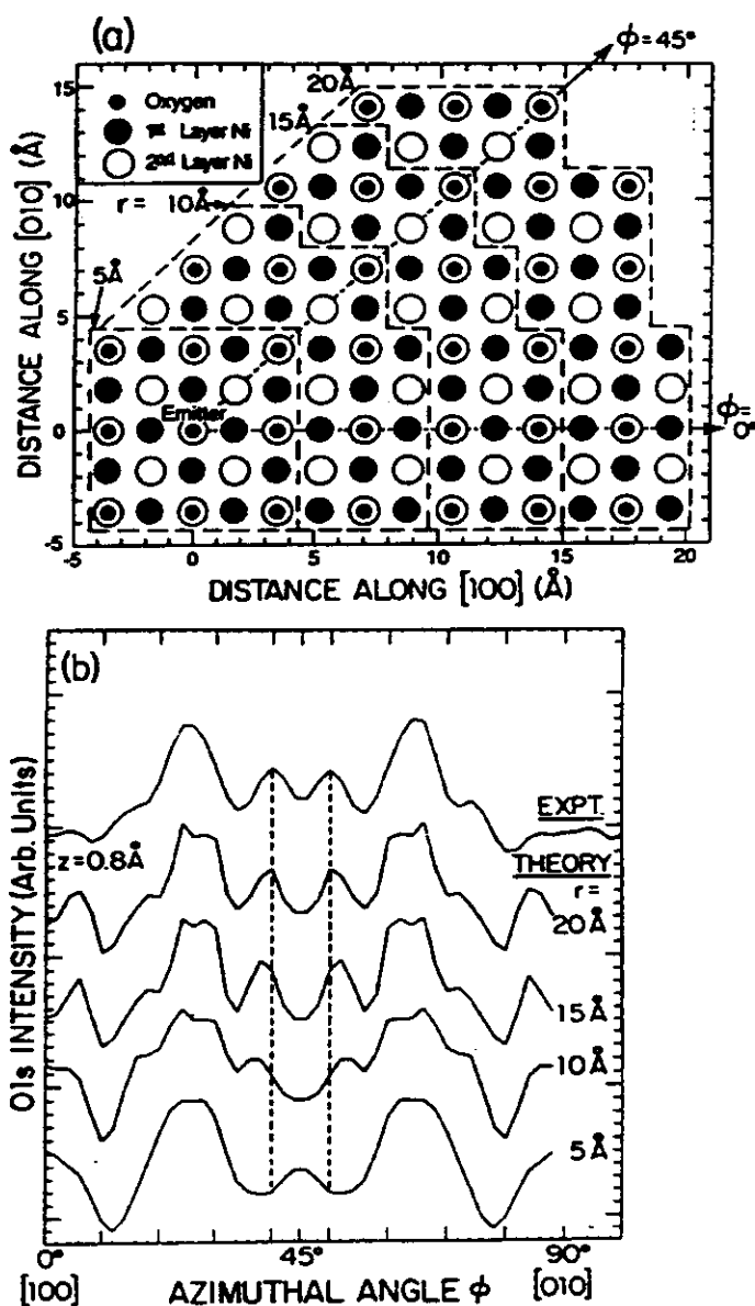
FIGURE 16. (a) Choices of cluster. Different-sized clusters used in testing the convergence of the SSC-SW curves for \theta = 8^\circ in Fig. 15(a), labelled with the approximate radii outward from the emitter that they represent. (b) Convergence with cluster size. Calculated curves for the clusters of (a) with z = 0.8 \text{ \AA} are compared to experiment. Note that a radius of at least 20 \text{ \AA} is required to yield optimum agreement. (From Ref. 26.)
