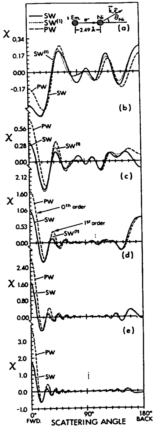
FIGURE 5. As in Fig. 4, but comparing plane-wave (PW) and spherical-wave (SW) scattering from a single Ni scatterer at a distance of 2.5 \text{ \AA} from the emitter with energies of (a) 50 eV, (b) 100 eV, (c) 200 eV, (d) 500 eV, and (e) 950 eV. Here, PW results are compared to SW results for the case of l = 0 ( s emission to a single p channel). Polarization is parallel to the emission direction. The curves labelled SW^{(1)} represent a first-order approximation to the full SW scattering. (From Refs. 21 and 58.)
