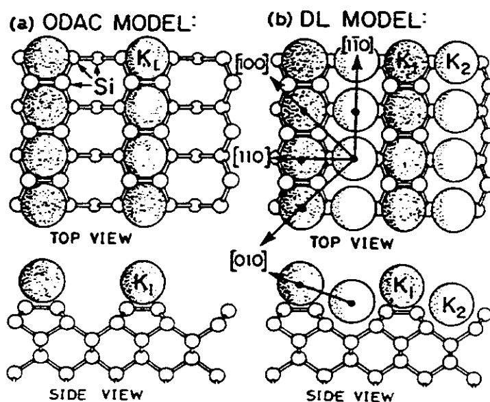
FIGURE 28. Schematic illustration of two structural models for the Si (001) (2 × 1) surface saturated with K: (a) one-dimensional-alkali-chain (ODAC) model, (b) double-layer (DL) model proposed from an analysis of azimuthal XPD data (see Fig. 29). Silicon dimers appear along the [1, -1, 0] rows in both models. Each model can exist in two domains rotated by 90° with respect to one another. Some strong forward-scattering directions in the DL model are shown by arrows. (From Ref. 114.)
