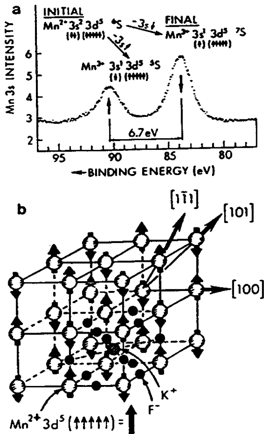
FIGURE 39. (a) The Al K\alpha -excited Mn 3s spectrum of \text{KMnF}_3 , with the initial and final states leading to the multiplet splitting indicated, together with the predominant photoelectron spin expected in each peak. (b) The crystal structure of \text{KMnF}_3 , with the antiferromagnetic ordering of the \text{Mn}^{2+} spins also indicated. [From Ref. 134(a).]
