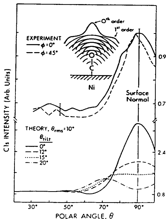
FIGURE 8. Comparison of polar-scan C 1s XPD data from c(2 \times 2) CO on Ni (001) at a kinetic energy of 1202 eV with SSC-PW theory. The inset indicates the type of intramolecular forward scattering and interference involved. Note definitions of zeroth-order and first-order effects, as shown also in Figs. 4 and 5. (From Ref. 69.)
