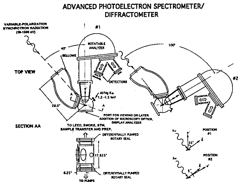
Fig. 6. Schematic drawing of the advanced photoelectron spectrometer/diffractometer (APSD) presently situated on beamline 9.3.2 of the Advanced Light Source. The rotation of the main chamber, including electron analyzer, and the range of photon-electron geometries possible are also indicated.
