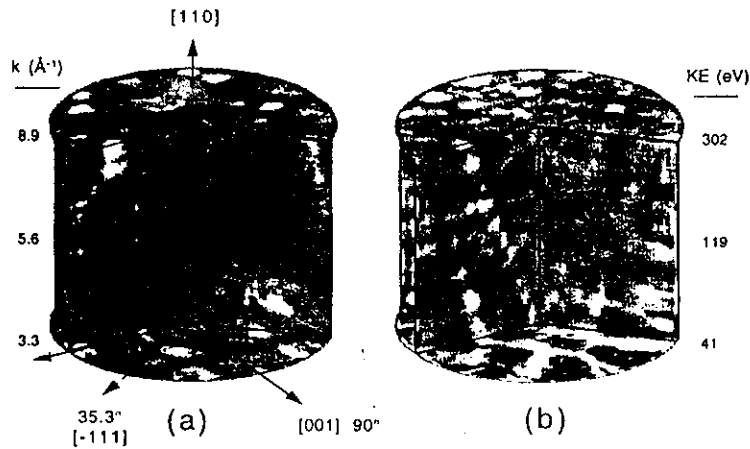
Fig. 21. Cutaway views of volume representations of the normalized intensities \chi(\mathbf{k}) for W 4f_{7/2} emission from clean W(110), with (a) from the bulk peak and (b) from the surface peak (as shown in Fig. 8(b)). The vertical scales are kinetic energy (KE) and wavevector, and each plane represents a stereographic projection of a nearly full-hemisphere data set taken over directions from the surface normal to within 10^\circ of the surface. [From ref. 50.]
