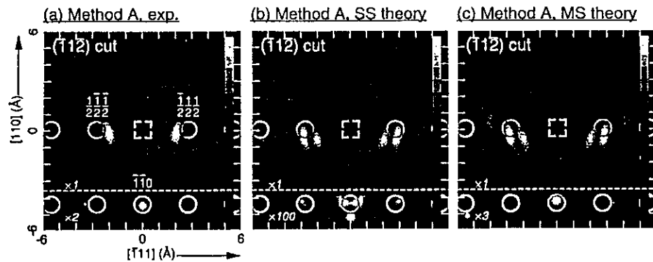
Fig. 22. W(110) holographic atomic images in the vertical (\bar{1}1\bar{2}) plane, as reconstructed using Eq. (2) from (a) the experimental surface-resolved W 4f_{7/2} data set of Fig. 21(b); (b) corresponding single scattering calculations, and (c) corresponding multiple scattering calculations. The surface-atom emitter is indicated by a dashed square, and the near-neighbor scatterers by circles. Image intensities for vertical coordinates \leq 3.5 Å have been rescaled, with the scale factors indicated on the figures. [From ref. 50.]
