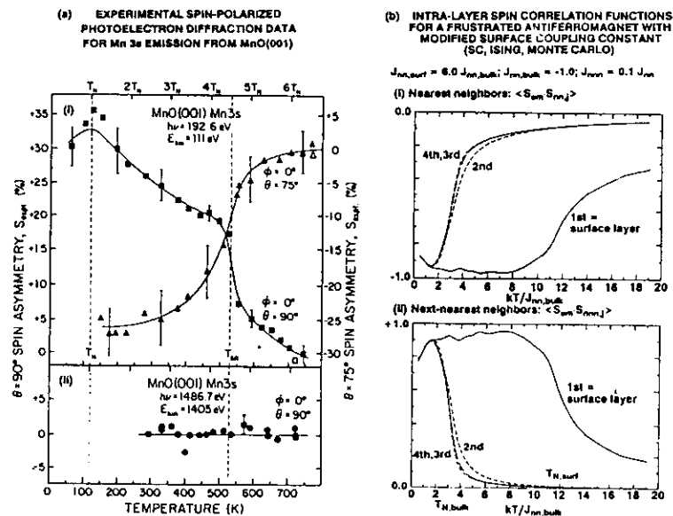
Fig. 18. (a) Temperature-dependent experimental spin-polarized photoelectron diffraction asymmetry data based upon Mn 3s spectra from MnO(001): In the top panel (i), the electron energy is 111 eV and data for two different directions are shown; in the lower panel (ii), the energy is 1405 eV, and only one direction (normal emission) is shown. [From refs. 9(c),(d).] (b) Monte Carlo theoretical calculations showing an elevated surface Néel temperature for a surface exchange interaction that is six times stronger than that in the bulk. [From ref. 44.]
