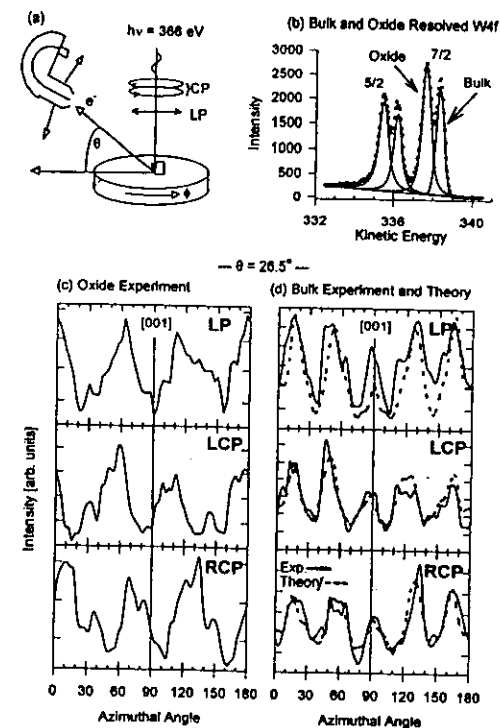
Fig. 13. Circular dichroism in the angular distributions of photoelectrons from (1x1)O/W(110) with a (1x12) incipient-oxide superstructure: (a) the experimental geometry, with radiation incident normal to the surface and the rotating analyzer of Figs. 6 and 7 being used to measure at various takeoff angles \theta with respect to the surface; (b) a W 4f spectrum with oxide and bulk peaks resolved; (c),(d) azimuthal scans at a takeoff angle of 26.5^\circ for both oxide and bulk W 4f components for linear-polarized (LP) light, left-circular-polarized (LCP) light, and right-circular-polarized (RCP) light (solid curves). In (d) is also a comparison of the experimental curve for bulk emission with theoretical photoelectron diffraction calculations (dashed curve). [From ref. 37.]
