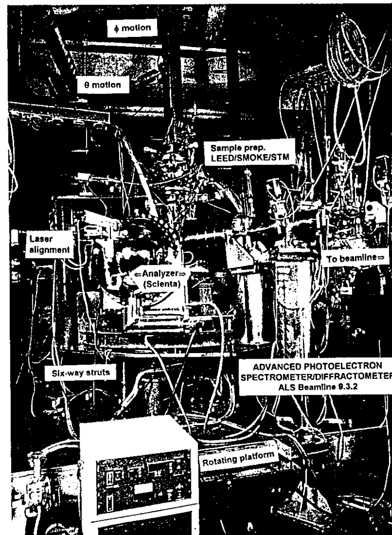
Fig. 7. Photograph of the APSD system in Fig. 6.
