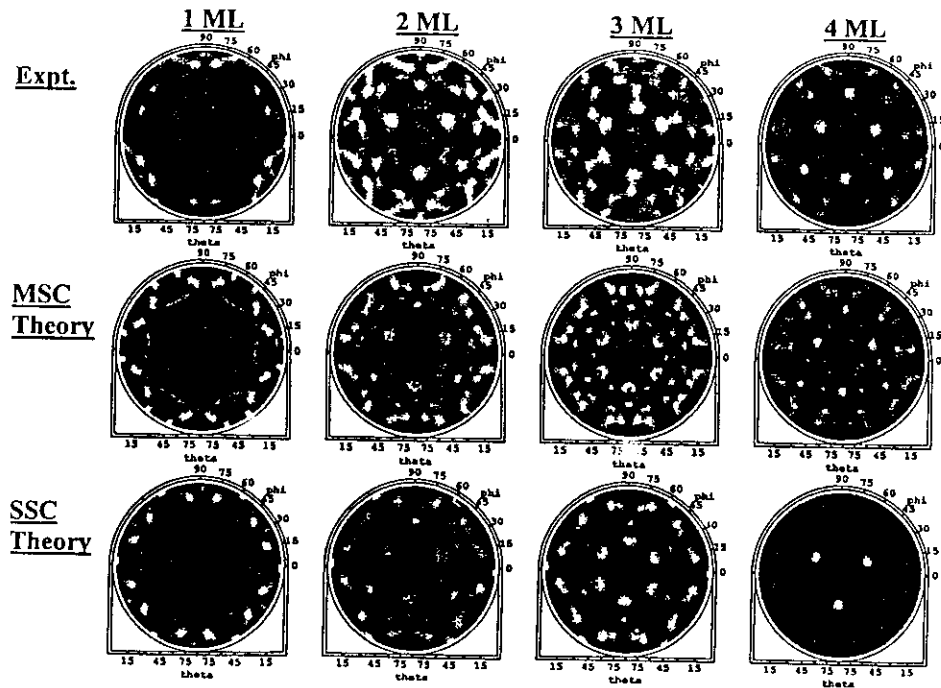
Fig. 5. X-ray photoelectron diffraction from the Cu 2p_{3/2} level of Cu on Ru(0001), for coverages of Cu from 1 to 4 ML. The kinetic energy is 556 eV. Also shown are the results of multiple scattering cluster (MSC) and single scattering cluster (SSC) calculations in which the interplanar spacings have first been varied to achieve best agreement with experiment. [From ref. 27(c).]
