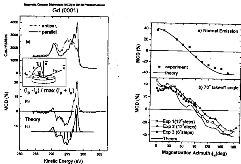
Fig. 15. (Upper left) (a) Gd 4d photoemission spectra taken at a photon energy of 450 eV using left circular polarized light. The solid-curve spectrum was taken with the sample magnetization \vec{M} parallel to the azimuth of the light incidence direction ( \Phi_M=0^\circ ), and the dotted-curve spectrum an antiparallel arrangement ( \Phi_M=180^\circ ). (b) The normalized difference of the spectra in (a) or MCD asymmetry. (c) A free-atom theoretical calculation of the MCD asymmetry, taken from ref. 42. The inset shows the experimental geometry. [From ref. 41.]
