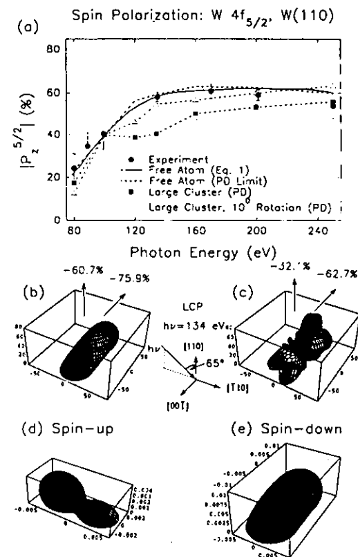
Fig. 20. Spin-polarization in W 4f spectra excited by circular-polarized light from W(110): (a) the absolute value of the 4f_{5/2} polarization as a function of photon energy, with experiment compared to both free-atom and MS cluster PD calculations; (b) the three-dimensional spin polarization for a free atom in the experimental geometry shown in the inset and with an excitation energy of 134 eV; (c) as (b), but for a MS cluster PD calculation in a 5-atom cluster (an emitter below 4 surface scatterers); (d),(e) the separate spin-up and spin-down intensities excited in a free-atom. [From ref. 48.]
