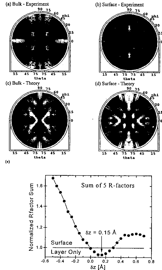
Fig. 9. Full-solid-angle W 4f_{7/2} photoelectron diffraction patterns: (a) bulk-resolved experiment, (b) surface-resolved experiment, (c) bulk theory for the optimum interlayer distance, (d) surface theory for the optimum interlayer distance; and (e) R-factor comparison between experiment and multiple-scattering theory for the surface-atom W 4f_{7/2} photoelectron diffraction pattern of Fig. 9(b). The curve represents a normalized sum of five R-factors. The horizontal line corresponds to an R-factor for calculations in which no bulk scatterers were present [From ref. 29.]
