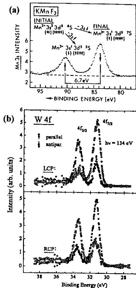
Fig. 17. Spin-polarized core photoelectron spectra: (a) a Mn 3s spectrum from \text{KMnF}_3 , with the electronic states and spin polarizations relative to the emitting \text{Mn}^{2+} ion indicated [From ref. 9(e).]; (b) a spin-resolved W 4f spectrum from W(110), excited by LCP light (top panel) and by RCP light (bottom panel). [From ref. 46.] In (b), the spin-resolved intensities as measured parallel or antiparallel to the light incidence direction \hat{q} are indicated.
