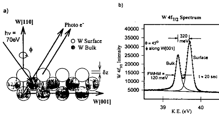
Fig. 8. (a) Experimental geometry used to study clean W(110), showing the two types of W atom sites resolved. (b) High-resolution W 4f_{7/2} spectrum from W(110), showing surface and bulk components. [From ref. 29.]
