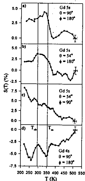
Fig. 19. Experimental spin asymmetry S(T) derived from Gd 5s and 4s multiplet intensity ratios R = I_{\uparrow} / I_{\downarrow} as a function of temperature T for (a) Gd 5s emission along the normal ( \theta = 90^\circ , \phi = 180^\circ along the "c" axis), (b) Gd 5s emission ( \theta = 54^\circ , \phi = 180^\circ along the "-b" axis), (c) Gd 5s emission ( \theta = 54^\circ , \phi = 90^\circ along the "a" axis), and (d) Gd 4s emission ( \theta = 90^\circ , \phi = 180^\circ along the "c" axis). Note the strong angle and level dependence of these results, with broad peaks in (a) and (b) for 5s, no visible effect in (c) for 5s, and two distinct features in (d) for 4s.
