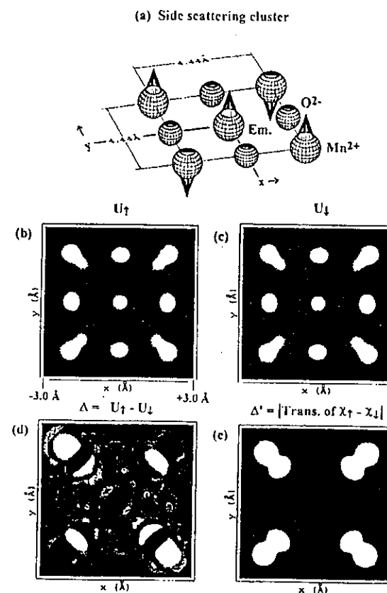
Fig. 23. A theoretical simulation of spin-polarized photoelectron holography: (a) a nine-atom cluster representing the (001) surface of MnO, with an emitter in its center; (b),(c) normal holographic images U_{\uparrow}(\vec{r}) U_{\downarrow}(\vec{r}) generated for the two different photoelectron spins by using Eq. (2) and holograms at 10 energies between 127 and 278 eV; (d) the spin-sensitive holographic image \Delta generated by using Eq. (3); (e) the spin-sensitive holographic image \Delta'(\vec{r}) generated by using Eq. (4). [From refs. 49(c),(d).]
