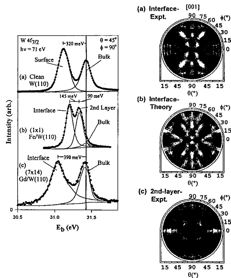
Fig. 10. (Upper left) W 4f_{7/2} photoelectron spectra taken with a photon energy of 71 eV from (a) the clean W(110) surface, (b) 1 ML of Fe in a (1x1) overlayer on W(110), and (c) 1 ML of Gd in a (7x14) Moiré superstructure on W(110). [From ref. 30.]
