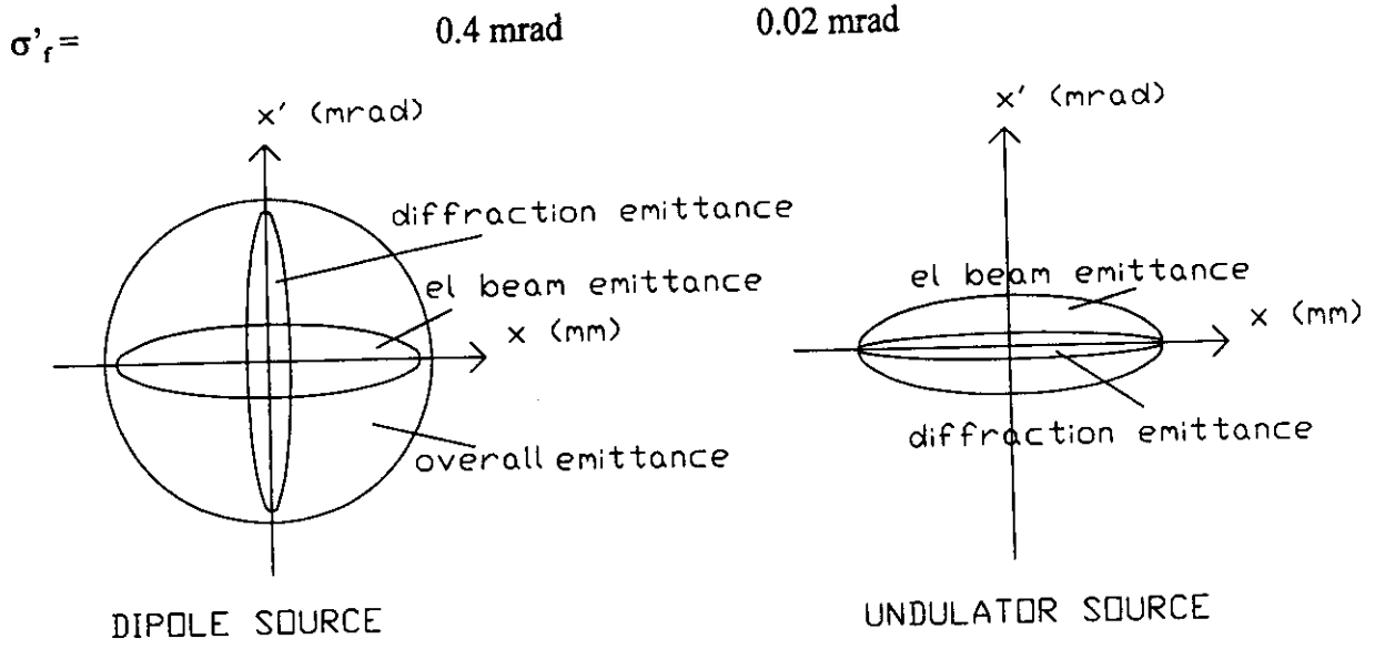
Fig. 11. Electron and photon beam emittances (horizontal).
