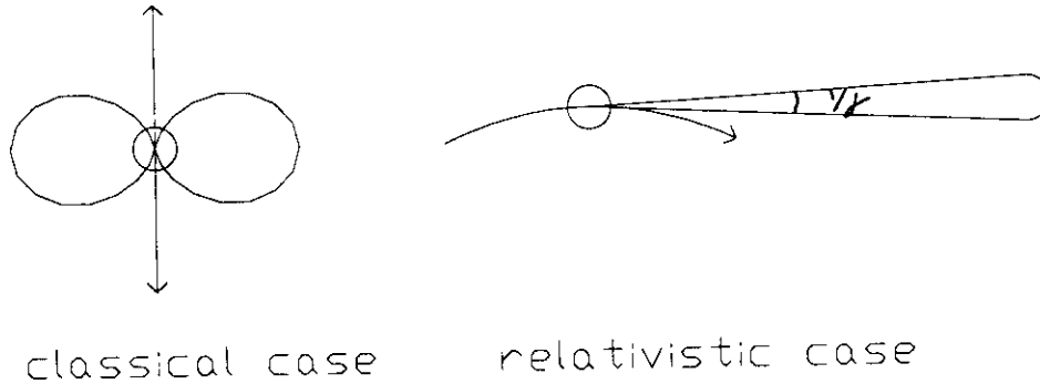
Fig. 3. Light intensity distribution in rest frame and lab frame systems.
