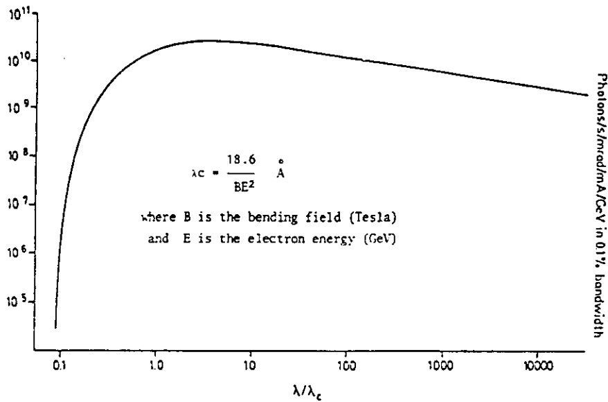
Fig. 9. Synchrotron radiation spectral distribution .
