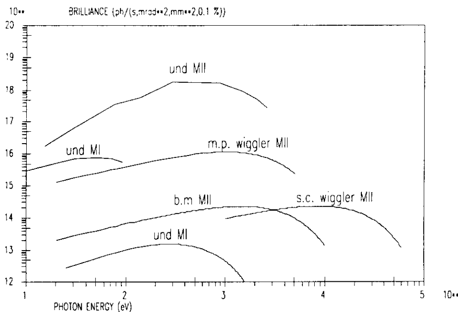
Fig. 13. Brilliance from dipoles and undulators in MAX II.
