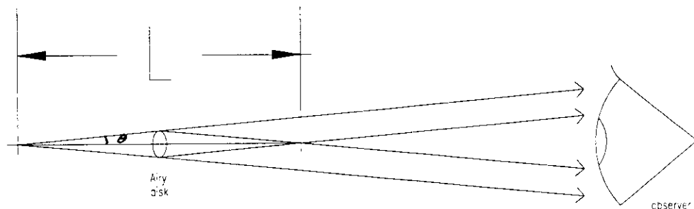
Fig. 10. Light emitted from a long, thin light source.
