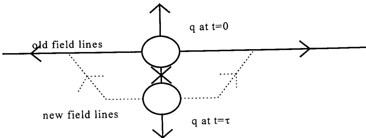
Fig. 1. Electric field from an accelerated charge.
