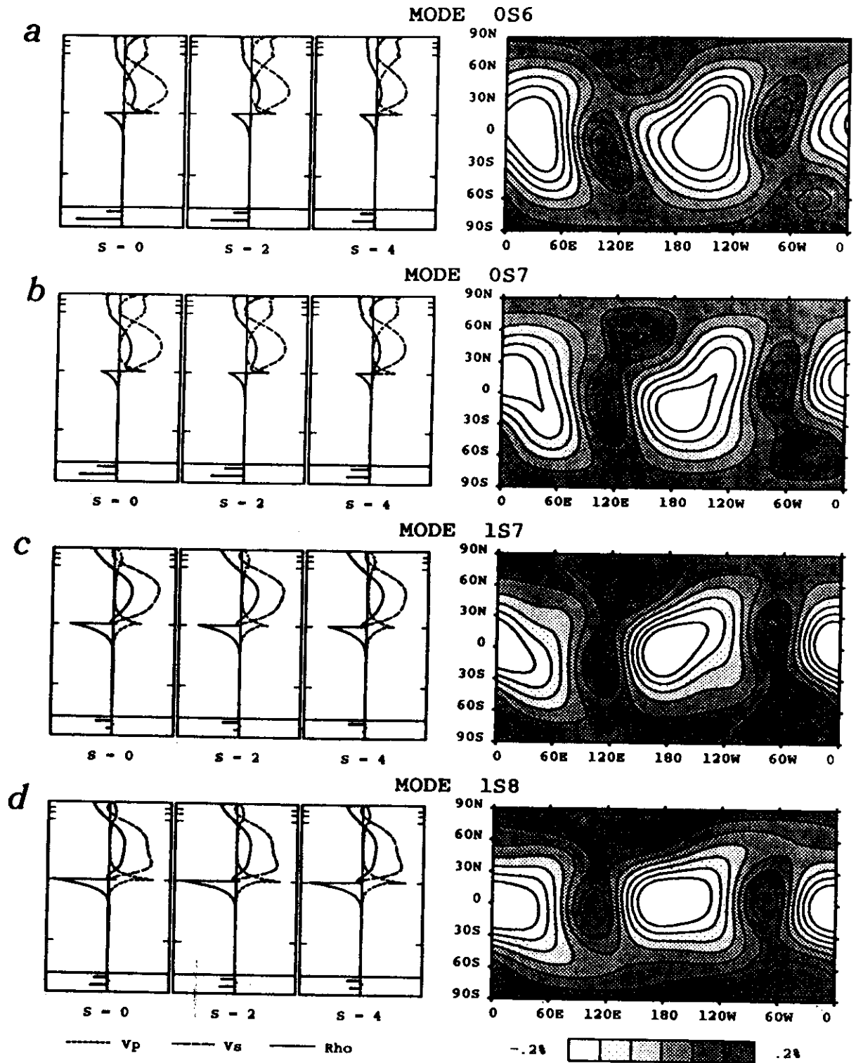
Differential kernels and splitting functions for modes 0S_6 , 0S_7 , 1S_7 , and 1S_8 , dominated by sensitivity to v_s structure in the lower mantle and having large kernels in the outermost core and in the proximity of the core-mantle boundary. See caption to Figure 7 for details.
