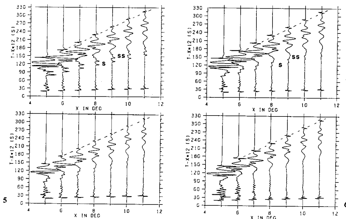
Fig. 5. Vertical (top) and radial (bottom) ground velocity components due to a vertical single force at 300 m depth
