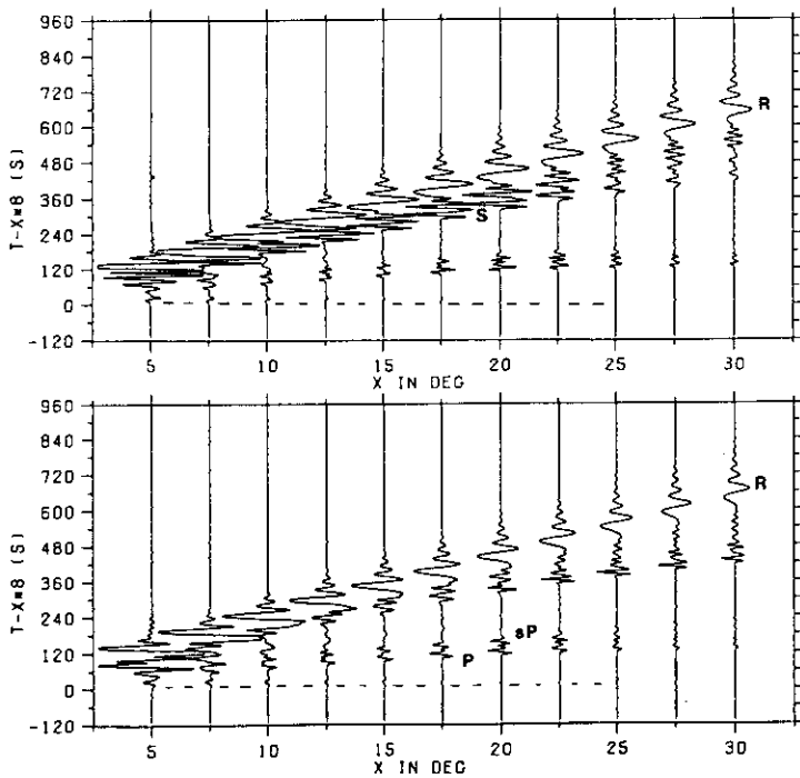
Fig. 4. Vertical (top) and radial (bottom) ground velocity components due to a vertical single force at 100 km depth. All other parameters are identical with those in Figure 3
