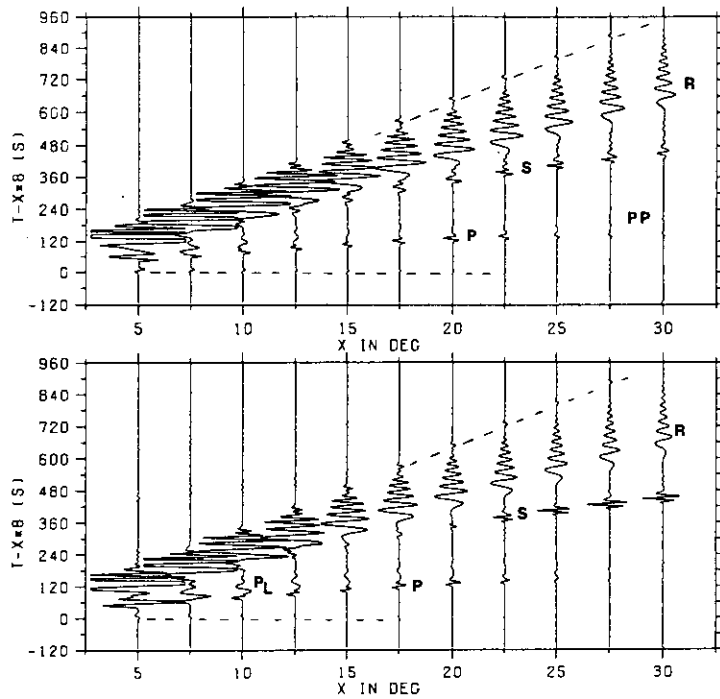
Fig. 3. Vertical (top) and radial (bottom) displacement components due to an explosive source in 300 m depth (Jeffreys-Bullen model). Lower and upper cut-off phase velocities are 2.8 and 15 km/s, respectively, cut-off period is 8.4 s. No amplitude correction due to the earth-flattening approximation is applied in this figure and in Figure 4. The decay of the P amplitudes with distance is too fast because the halfspace was assumed at a too shallow depth
