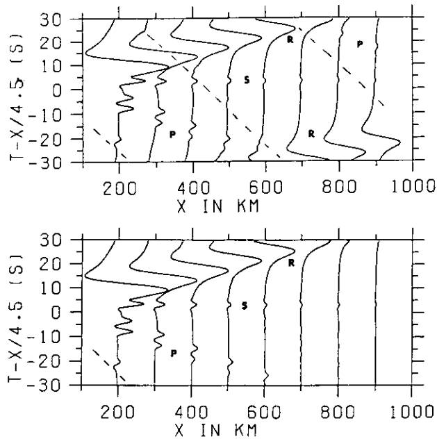
Fig. 3. Theoretical seismograms for two different \omega -integration methods: Top: constant \omega -spacing. Bottom: Variable \omega -spacing. The source is a single vertical force at 30 km depth in a halfspace. The dashed line indicates a numerical phase connected with the limit of the k -integration. All phases due to aliasing have disappeared in the bottom case. R: Rayleigh wave; P: P-wave; S: S-wave
