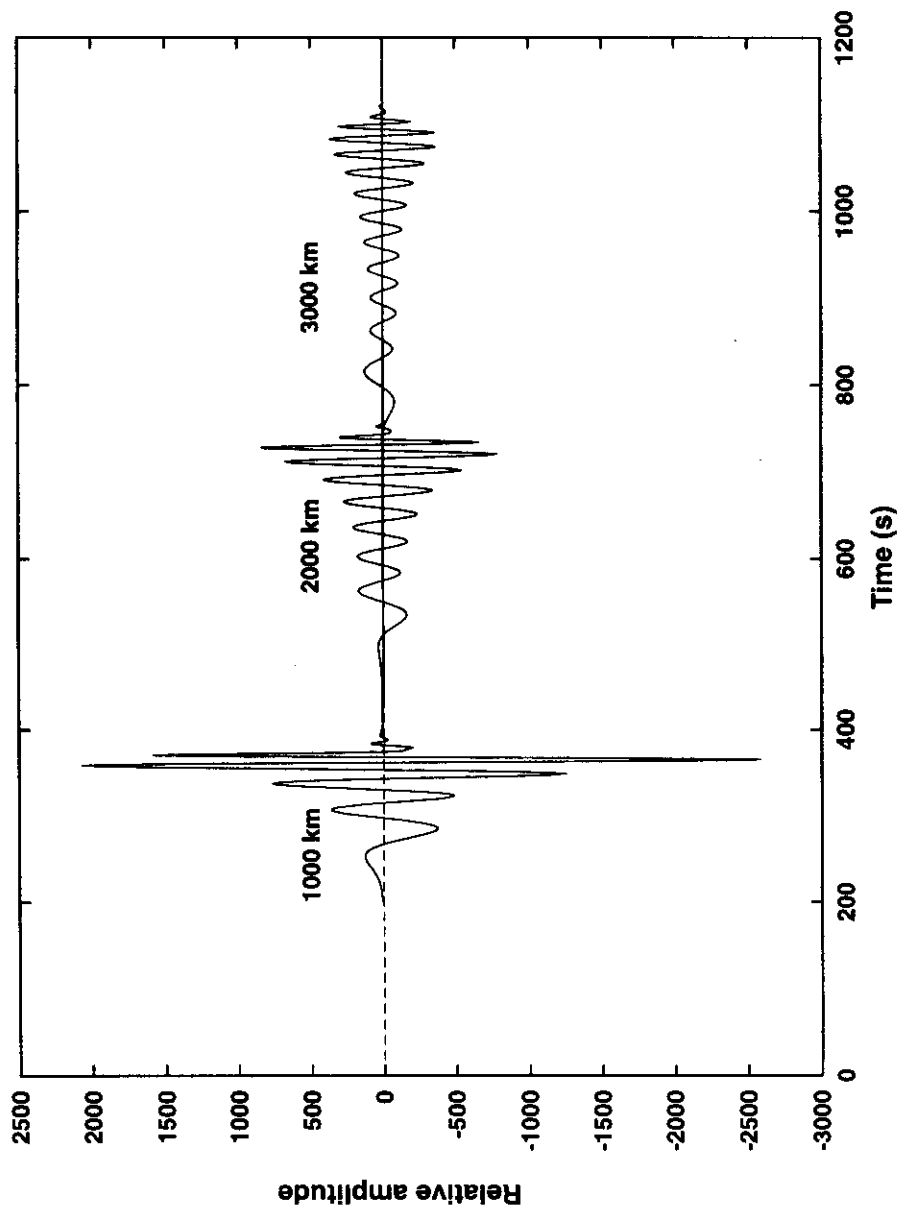
Figure 5. Synthetic seismograms of the vertical component of the Rayleigh wave (model EUS)
