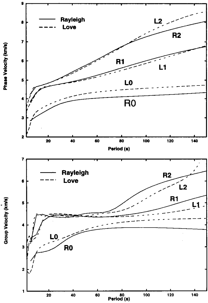
Figure 3. Phase and group velocities of the three first modes of Rayleigh and Love waves at the continental model EUS
