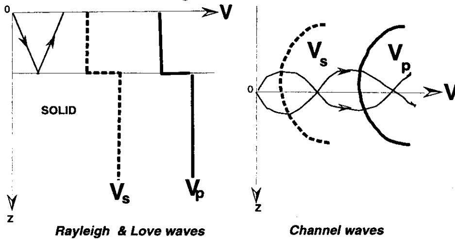
Figure 1. When surface or channel waves may exist.
