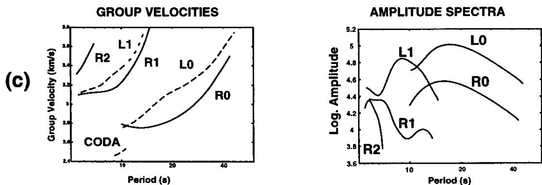
Figure 8. The earthquake at Iran-Turkmenistan border recorded at AAK (epicentral distance 1560 km): (a) records; (b) FTAN diagrams; (c) group velocities and amplitude spectra. Strong higher modes and fundamental modes of Rayleigh and Love waves are present.
