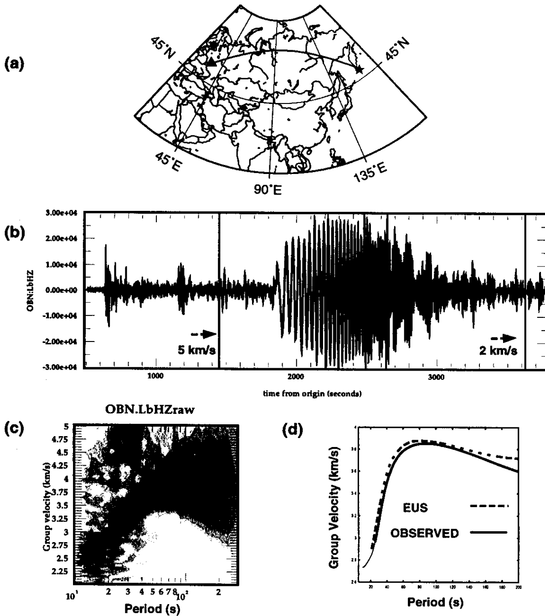
Figure 10. Rayleigh wave propagation along a continental path: (a) Wave path across Eurasia (from N. Kuril Island to Moscow); (b) Record of the vertical component; (c) FTAN diagram; (d) observed group velocity and prediction from the average continental model.
