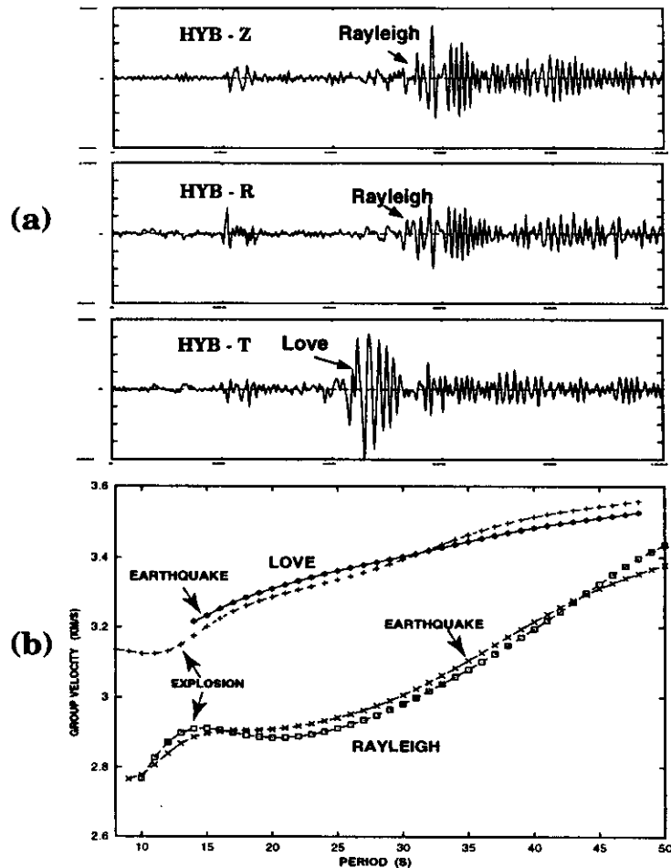
Figure 15. Tectonic release from the nuclear underground explosion at Lop Nor, China: (a) Love waves have the highest intensity for the three-component seismogram of the explosion on 05/21/1992 recorded at HYB; (b) Group velocity curves for this event and an earthquake near Lop Nor on 11/03/1990 are very similar.
