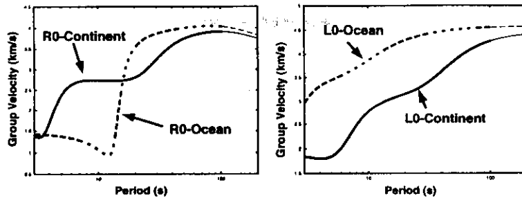
Figure 9. Group velocities of fundamental Rayleigh and Love waves along continental and oceanic paths.
