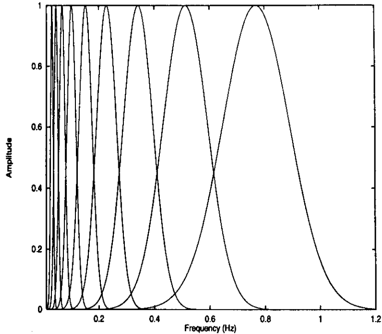
Figure 1. A comb of Gaussian frequency domain filters with constant relative bandwidth used in FTAN.
