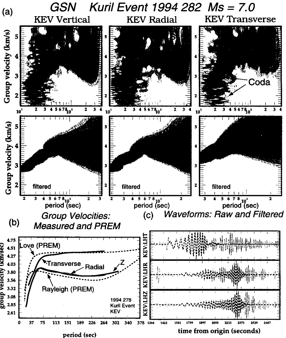
Figure 2. (a) Group velocity - period diagrams for the vertical, radial, and transverse components recorded at the GSN station at Kevo, Finland for an event in the Kurils (10/9/94, M_s = 7.0 , \Delta = 58.5 degrees). Estimated group velocity curves are shown. (b) Rayleigh and Love wave group velocity measurements compared with predictions from PREM. (c) Raw (thin solid) and filtered (bold dashed lines) waveforms for KEV.
