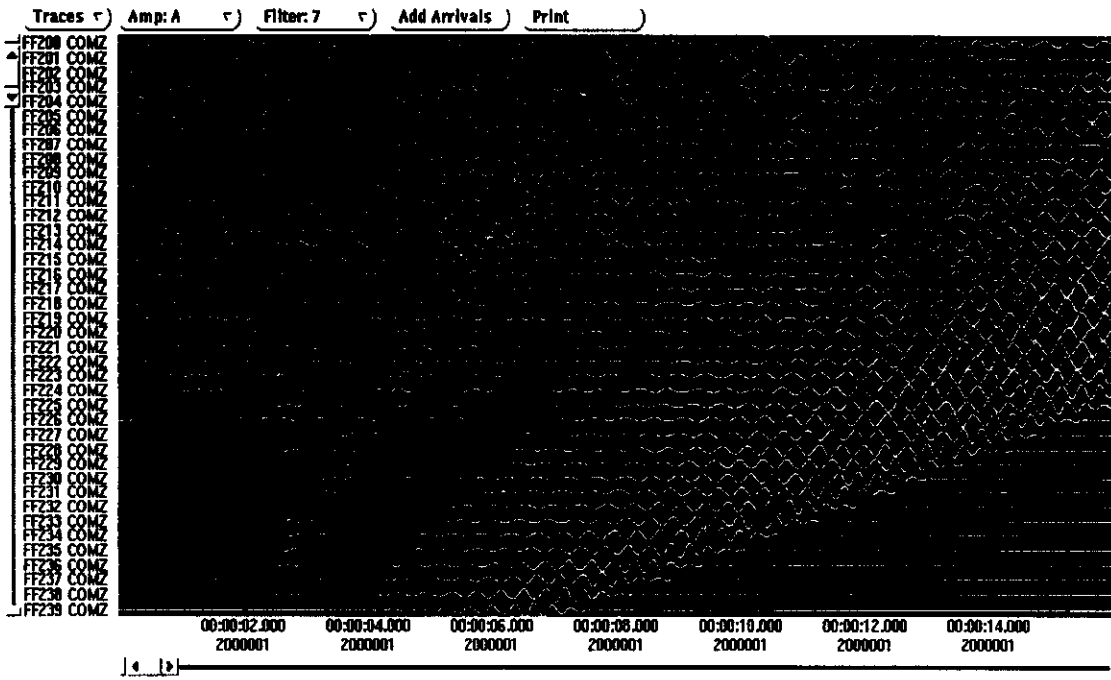
Figure 4. Sea-bottom records filtered by a low-pass filter with 3 Hz corner frequency.
