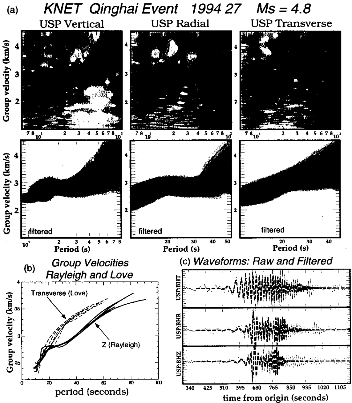
Figure 3. (a) Group velocity - period diagrams for the vertical, radial, and transverse components recorded at the KNET station USP for an event in the Qinghai Province (1/27/94, Ms = 4.8, \Delta = 16 degrees). Estimated group velocity curves are shown. (b) Rayleigh and Love wave group velocities measured across the array for the same event. (c) Raw and filtered waveforms for the station USP.
