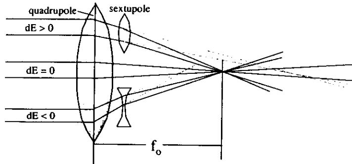
Figure 17: Correction of Chromatic Aberrations
