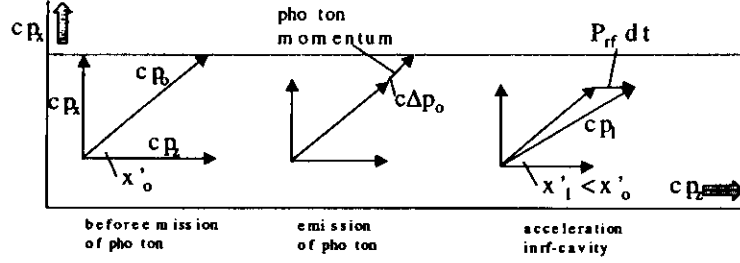
Figure 11: Transverse Damping Effects
