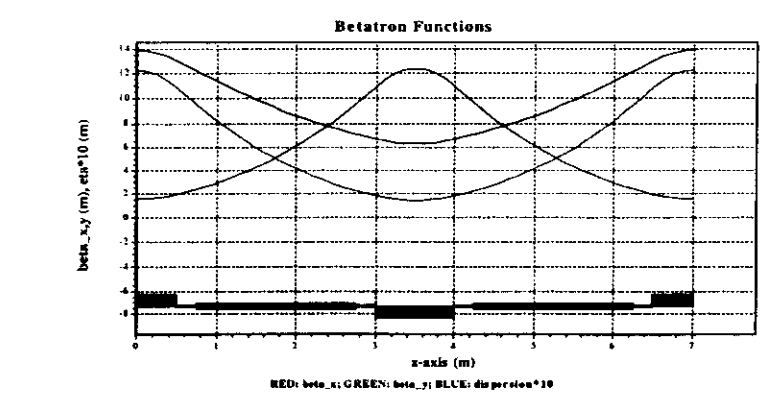
Figure 9: Betatron Functions in a FODO-Lattice
