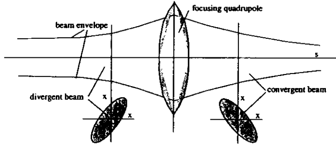
Figure 7: Variation of a Phase Space Ellipse along a Drift Space
