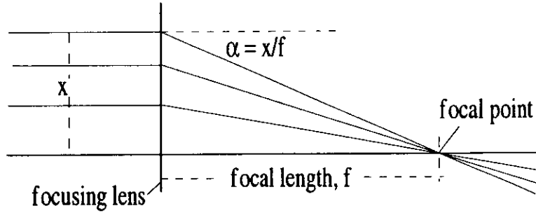
Figure 3: Principle of Focusing
