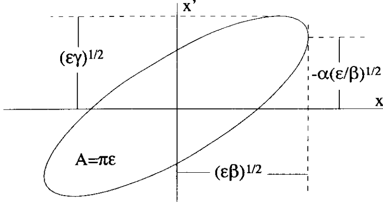
Figure 6: Phase Space Ellipse
