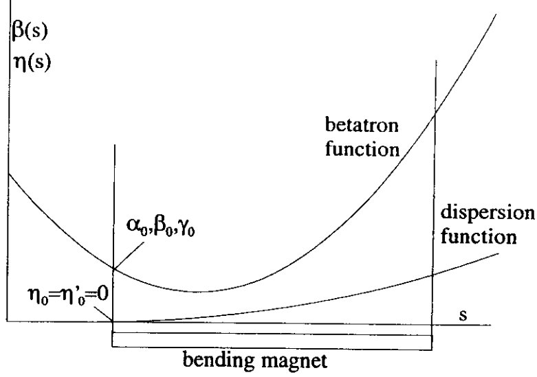
Figure 12: Betatron Functions within a Bending Magnet
