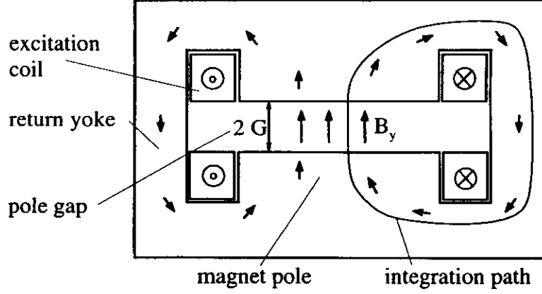
Figure 2: Bending Magnet Cross Section
