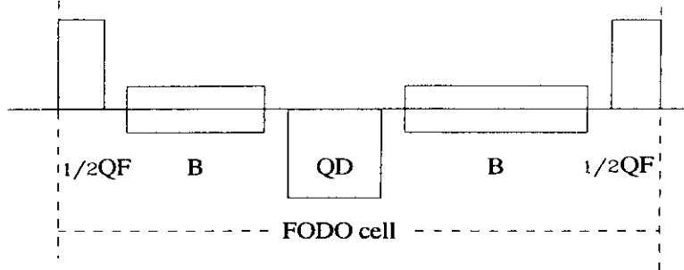
Figure 5: FODO Lattice schematic
