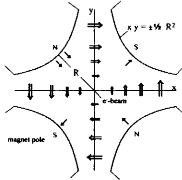
Figure 4: Cross section of a quadrupole magnet, schematic
