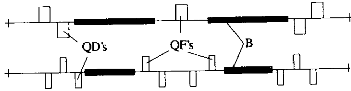
Figure 13: dba-Lattice,schematic
