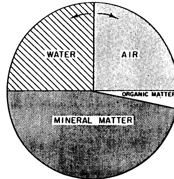
Fig. 1. Schematic composition of a medium-textured soil at a water content considered favorable for plant growth.
