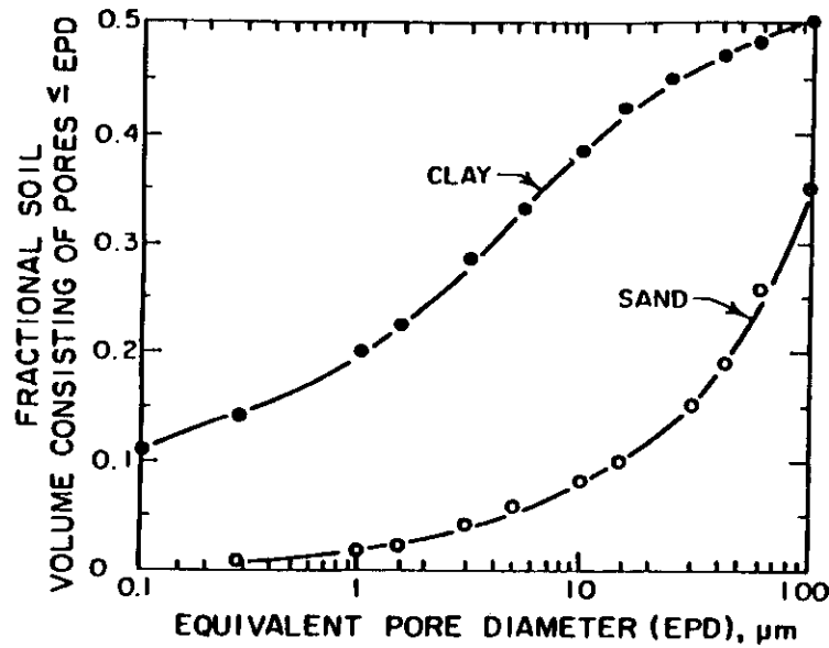
Fig. 6. Pore-size distribution of a clay and a sand soil.
