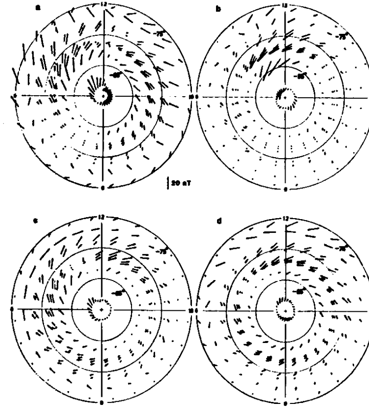
Fig. 3. The equivalent current vector distributions over the southern polar cap related to the IMF: a) B_z < 0 ; b) B_z > 0 ; c) B_z < 0 ; d) B_z > 0 . Arrows indicate the scale factor 20 nT. Corrected geomagnetic latitude ( \theta ) — magnetic local time (MLT).
