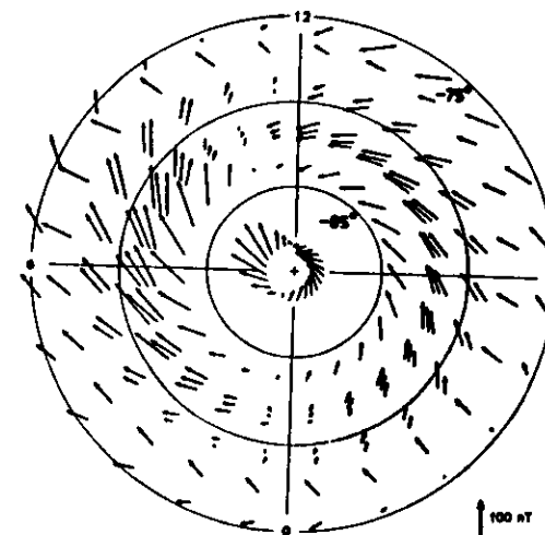
Fig. 4. The equivalent current vector distribution over the southern polar cap for the free term of the multiregressional equation. Scale factor is 100 nT.
