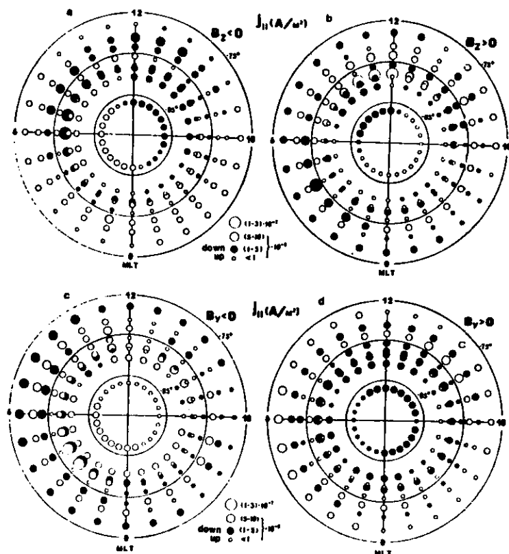
Fig. 5. Field-aligned current distributions over the southern polar cap related to the IMF: a) B_z < 0 ; b) B_z > 0 ; c) B_y < 0 ; d) B_y > 0 . Black circles—downward currents, open circles—upward currents. Scale factors (from large to small circles) are (1-3) \cdot 10^{-7} , (5-10) \cdot 10^{-8} , (1-5) \cdot 10^{-8} and less than 1 \cdot 10^{-8} A/m 2 respectively.
