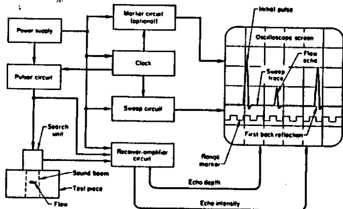
Typical A-scan setup, including video-mode display, for a basic pulse-echo ultrasonic-inspection system
