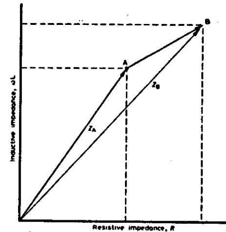
Figure 14. Impedance plane diagram demonstrating amplitude and phase change experienced in eddy-current testing. Impedance, Z , of test coil
