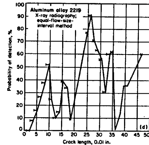
Fig.26 Charts of lower-bound probability of detection of fatigue cracks of various lengths
