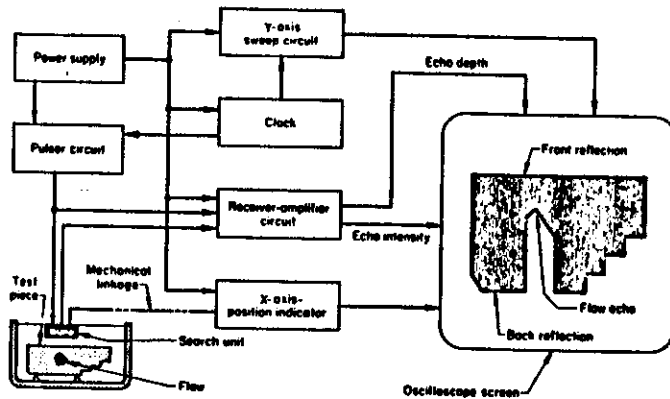
Typical B-scan setup, including video-mode display, for a basic pulse-echo ultrasonic-inspection system
