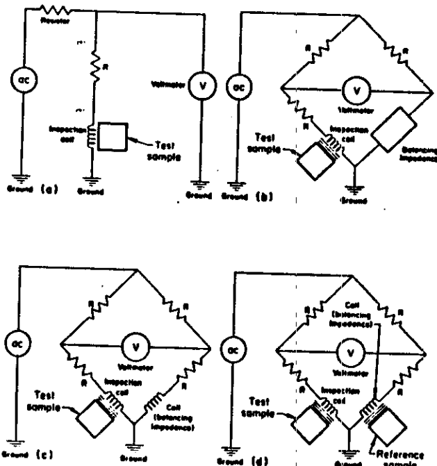
Fig. 12. Four types of eddy-current instruments: (a) a simple arrangement, in which voltage across the coil is monitored; (b) typical impedance bridge; (c) impedance bridge with dual coils; and (d) impedance bridge with dual coils and a reference sample in the second coil
