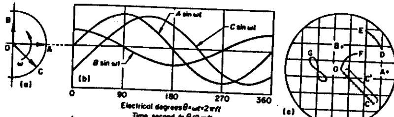
Fig16 Phasor representation of sinusoids.
