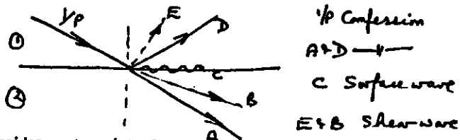
General non-90° incidence at an interface.
