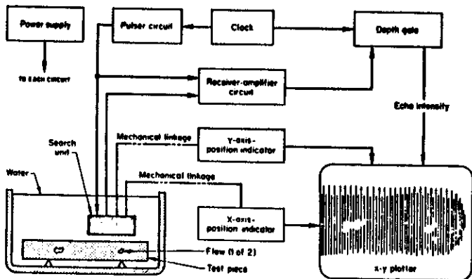
Typical C-scan setup, including display, for a basic pulse-echo ultrasonic-inspection system
