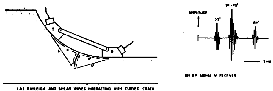
(A) RAYLEIGH AND SHEAR WAVES INTERACTING WITH CURVED CRACK
