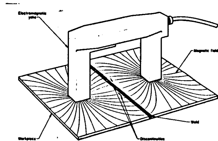
Fig 36 Electromagnetic yoke, showing position and magnetic field for detection of discontinuities parallel to a weld bead. Discontinuities across a weld bead may be detected by placing the contact surfaces of the yoke next to and on either side of the bead (rotating yoke about 90° from position shown here).
