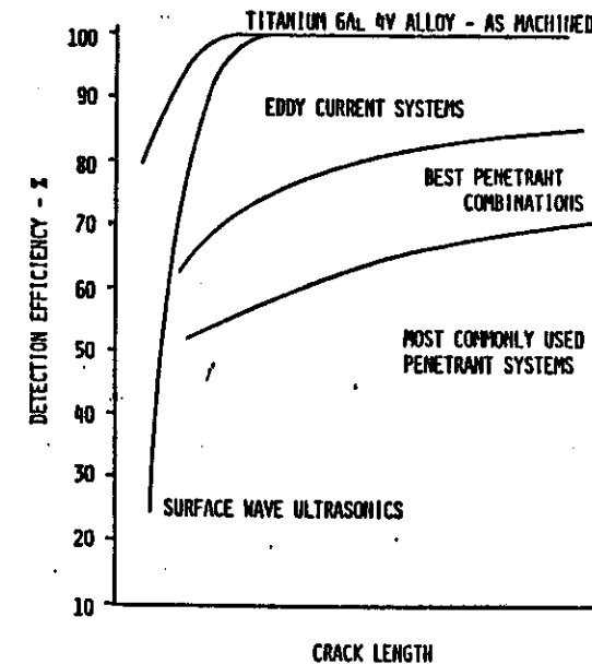
Comparison of the typical detection performance of eddy current inspections with other surface sensitive processes
