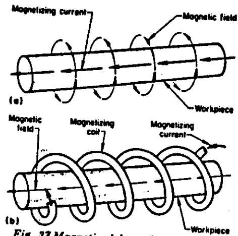
Fig. 32 Magnetized bars showing directions of magnetic field: (a) circular and (b) longitudinal
