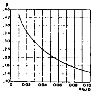
Fig. 10. Nomograph for the determination of B in the Dagan equation (DAGAN, 1964).
