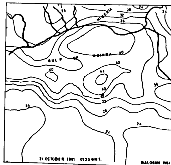
FIG. 32. Precipitable water over gulf of Guinea (in mm) from NOAA-6 satellite.
