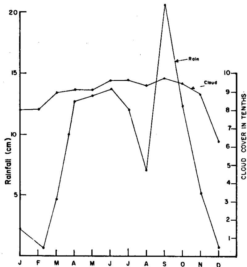
FIG. 20. Monthly mean cloud amount and monthly mean rainfall between the coast and Lat. 10°N over Nigeria.
