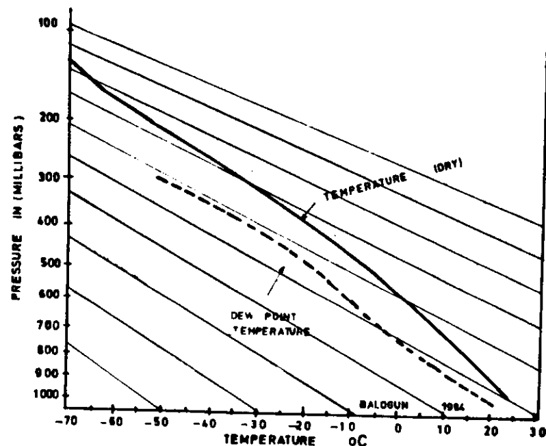
FIG. 27. Vertical distribution of temperature at lat. 12.45^\circ\text{N} , long 8.43^\circ\text{E} from NOAA-6 satellite measurements, 21 October 1981.
