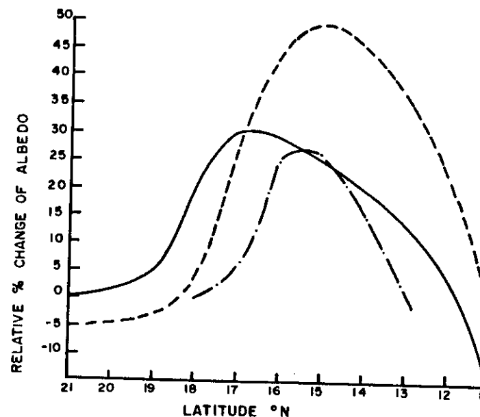
FIG. 24. Seasonal surface albedo change over the Sahel (after Norton et al. , 1979).
