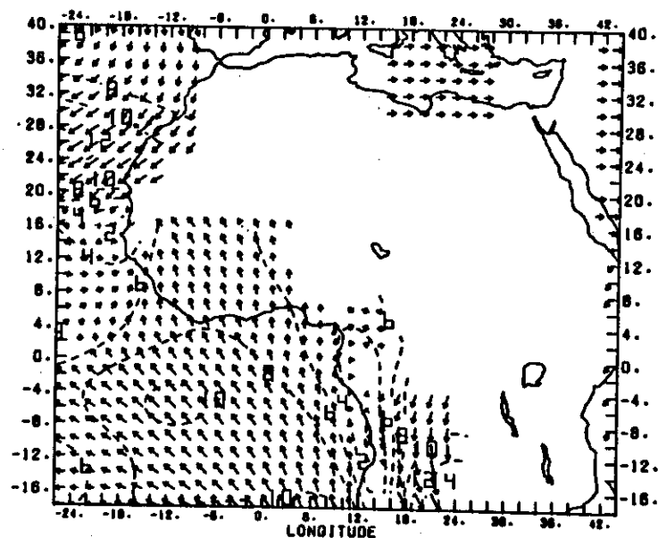
Fig. 14. Satellite-derived low level winds for 1200Z, July 18, 1979.
