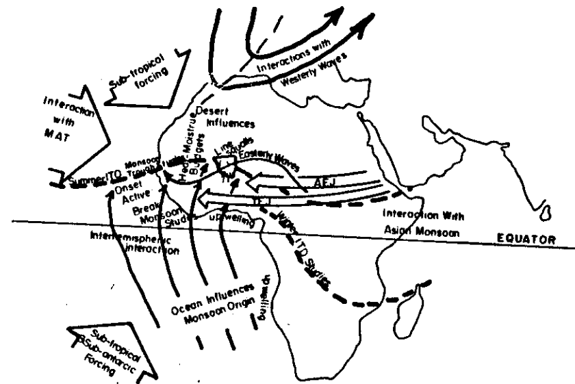
FIG. 1. Some atmospheric systems which influence weather events in Tropical Africa. (Adapted from GARP. Publication series No 21. World Meteorological Organization).
