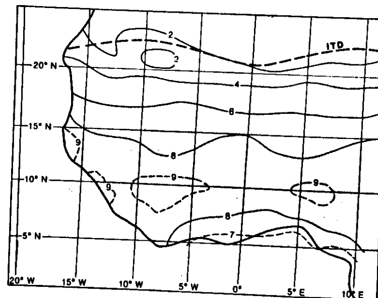
FIG. 3. Mean cloud cover in tenths for the period July 15th to August 15th, 1979, using infrared imagery from the Meteosat.
