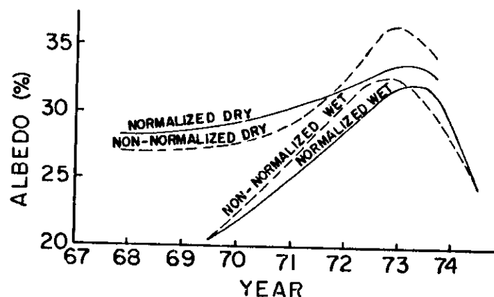
FIG. 25. Quasi-annual variation of the Saharan mean albedo (12°N to 18°N) for wet and dry season (after Norton et al. , 1979).
