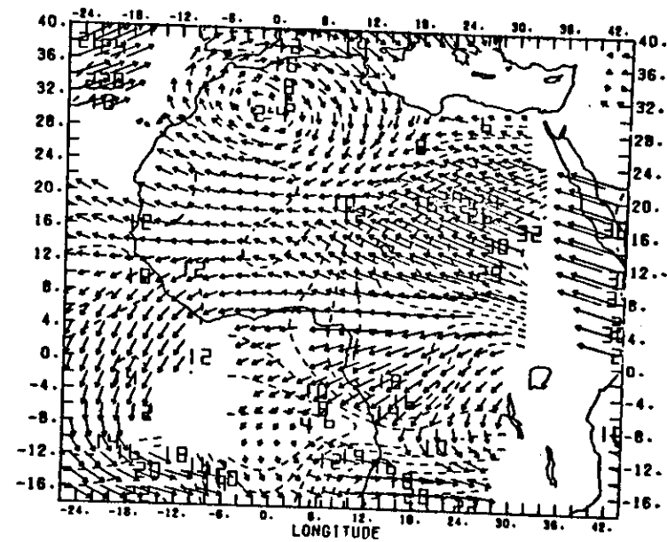
FIG. 18. Satellite-derived upper level winds at 1200Z, July 23, 1979.
