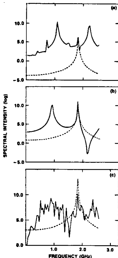
FIG. 3. Computed output intensity spectra for a frequency ratio \omega_0/\omega_{ext} = 0.59 and different modulation depths, m . The external modulation is shown as the dashed line. (a) m = 0.01 ; quasiperiodic (b) m = 0.1 ; phase-locked (c) m = 0.3 ; chaotic. Note that in this sequence the winding number is not fixed. The parameters used in Eqs. (1)–(3) are I = 1.2 , G = 3.0 \times 10^3 , \tau = 3 \times 10^{-4} , \beta = 5.0 \times 10^{-5} , h = 240 , S_0 = 0.001 . The spontaneous carrier lifetime is 3.0 ns.
