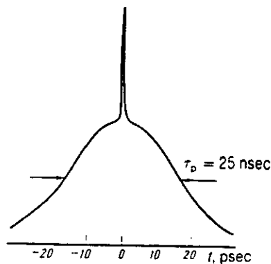
FIG. 6. Autocorrelation function radiation at the Stokes wavelength ( \lambda_s \approx 1.33 \mu ).
