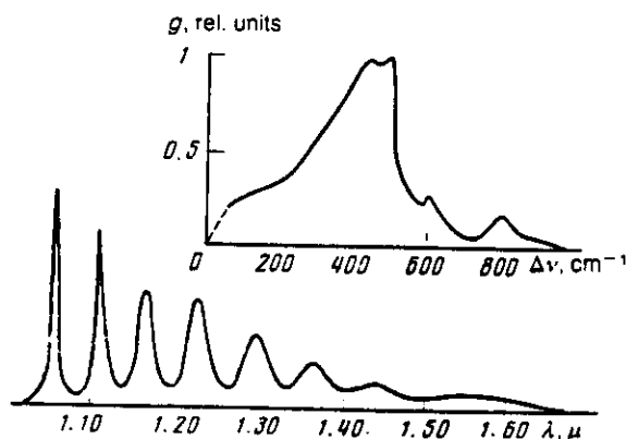
FIG. 1. Overall spectrum of multistage StRS in a fiber waveguide of length 250 m pumped with pulses of \lambda_p = 1.064\ \mu wavelength and \tau_p \approx 150\ \text{nsec} duration. The inset shows the spectrum of the StRS gain g of fused quartz ( \lambda_p = 1.064\ \mu ) plotted using the data of Ref. 6.
