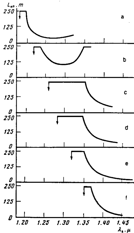
FIG. 3. Dependences of the effective length of the region of interaction between the pump and Stokes waves on the Stokes wavelength \lambda_s calculated for different pump wavelengths \lambda_p (identified by arrows) allowing for the dispersion of the group velocities in the case of pulses of \lambda_p = 30 psec duration.
