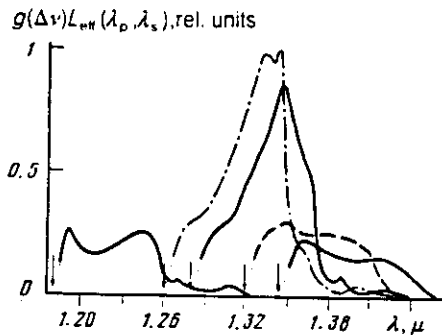
FIG. 4. Spectral dependences of the StRS gain increment ( I_p = \text{const} ) obtained for different pump wavelengths \lambda_p (identified by arrows) as a result of multiplication of the g(\Delta\nu) curves from Fig. 1 and L_{\text{eff}}(\lambda_p, \lambda_s) from Fig. 3.
