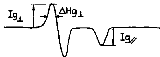
typical Q-band ESR signal
