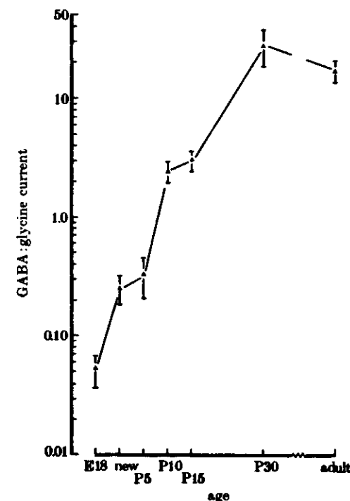
FIGURE 3. Ratios of GABA to glycine response sizes in individual oocytes. Each point represents the average of 8–35 oocytes taken from 2–4 donors; bars indicate standard error of mean. For each developmental age data from 1–3 mRNA preparations were used. Glycine responses in oocytes injected with mRNAs from older ages (P30 and adult) were often undetectable (less than 1 nA) and those data were not included in the mean.
