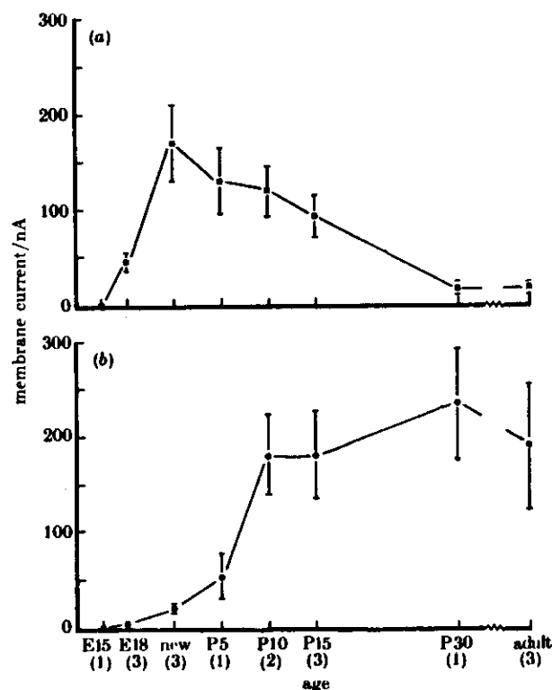
FIGURE 2. Peak sizes of membrane currents recorded from oocytes injected with cerebral cortex mRNA (except for the E15 and one E18 mRNA preparation in which the entire cerebral hemispheres were used) from different stages of rat development, measured from records like those in figure 1. Each point represents the mean \pm standard error of measurements from 8–38 oocytes from 7 donors. The numbers of replicate mRNA preparations examined are indicated below each age. Oocytes from each donor were injected with several mRNAs, except for E15 mRNA, which was used in three donors which were not injected with the other mRNAs. (a) Glycine, 10^{-3} M; (b) GABA, 10^{-3} M.
