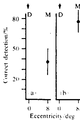
Figure 3. Eccentric enhancement of single letters from the first group of subjects used (experiment 1). (a) Unlike letters were presented simultaneously at the fixation point (0 deg) and at 8 deg eccentricity. (b) Like letters were presented at these locations. Averages of correct identifications are given by the solid dots, standard deviations by the vertical bars. The resulting difference between the averages is significant ( p < 0.001 ).
