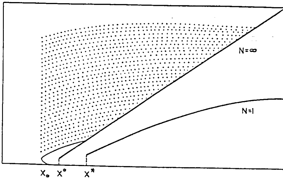
Figure 5. Threshold investment in a whale fleet as a function of initial whale stock level. N = \infty vs N = 1 . The logistic model is with parameter values from Clark and Lamberson (1982).
