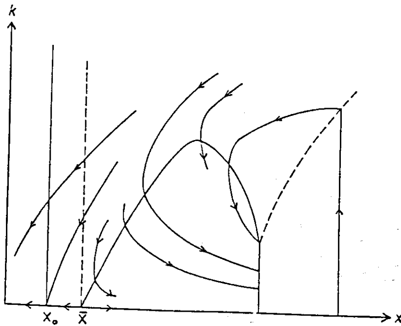
Figure 3. Phase-plane portrait: N = \infty ; (a) depensation and (b) over-depensation.
