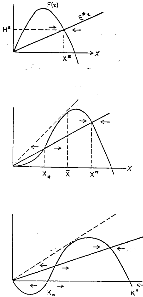
Figure 1. Growth curves F(x) : (a) compensatory, (b) depensatory, and (c) over-depensatory. Equilibrium under constant-effort harvest E is at intersection of the graph of F(x) with the straight line qx E . Arrows show non-equilibrium direction of motion.
