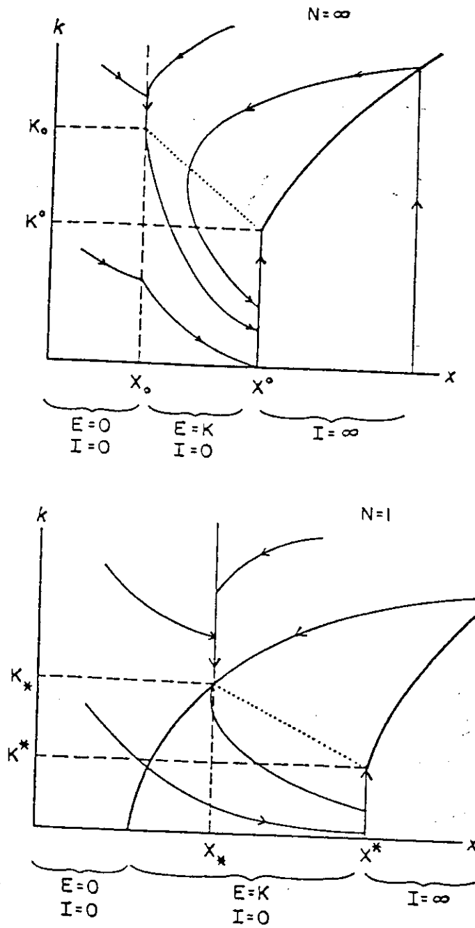
Figure 2. Phase-plane portrait: Compensatory model, (a) N = \infty and (b) N = 1 . (After, respectively, McKelvey 1985, and Clark et al. 1979).
