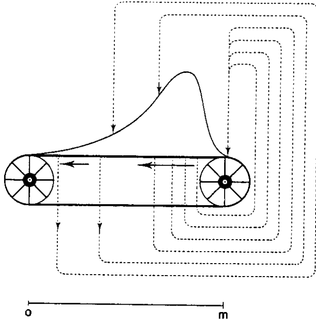
Fig. 2. Conveyor belt representation of a structured population model.
