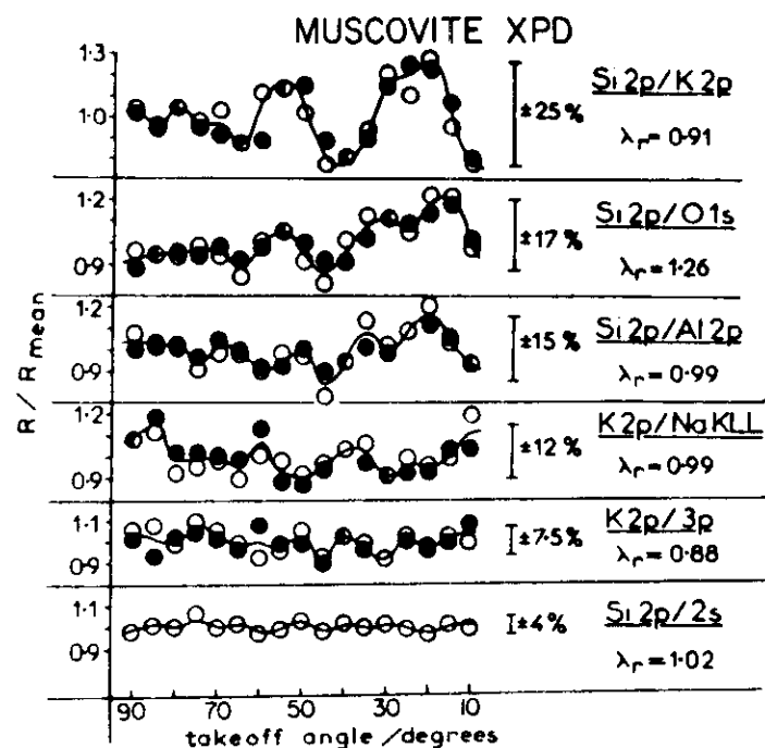
Fig. 32. Experimental polar dependence of normalized core intensity ratios for different peaks resulting from a single crystal of the mineral muscovite ( K(Al_2)(Si_3Al)O_{10}(OH)_2 ). The full range of excursion is indicated as a percentage, and \lambda_r denotes the ratio of de Broglie wavelengths of the two peaks involved in a given ratio. (From Adams, Evans, and Thomas, ref. (66).)
