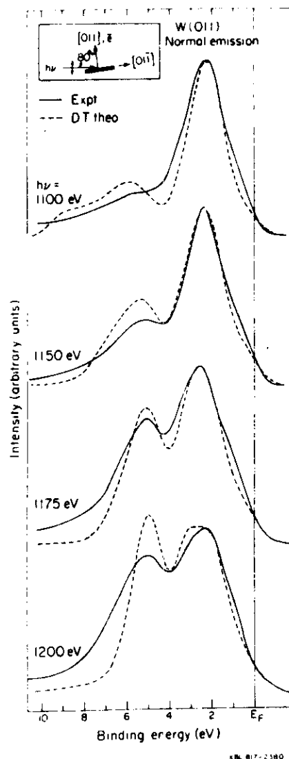
Fig. 68. Comparison of direct-transition theory to the first XPS valence-band experiments making use of tunable synchrotron radiation. Emission was normal to a W(011) surface; the geometry is shown as an inset. (From Hussain et al., ref. (10).)
