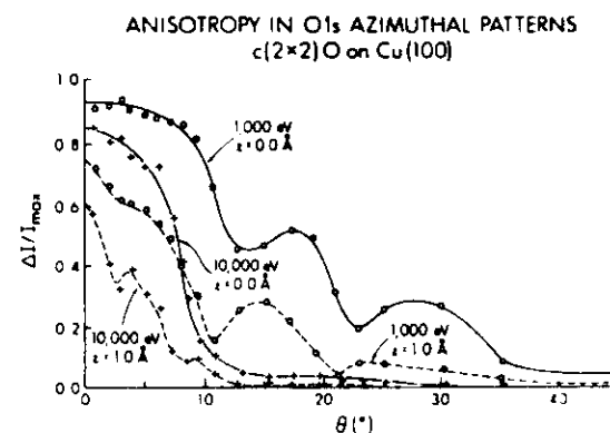
Fig. 59. Dependence of overall XPD anisotropy \Delta I/I_{max} on emission angle \theta , adsorbate z position, and electron kinetic energy for c(2x2)O on Cu(001). In general, increasing \theta , moving the adsorbate from in-plane ( z = 0.0 Å) to above-plane ( z = 1.0 Å), or increasing energy from 1,000 eV to 10,000 eV tends to decrease the anisotropy. (From Thompson, ref. (80).)
