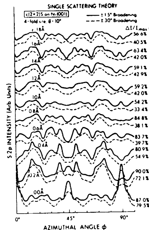
Fig. 50. The effect of reducing analyzer acceptance from \pm 3.0^\circ to \pm 1.5^\circ on azimuthal XPD. Theoretical SSC curves for the azimuthal dependence of S2p intensity from c(2 \times 2)\text{S} on Ni(001) at \theta = 10^\circ are shown for the two angular acceptances and a range of 4-fold-coordinate z values from 0.0 \text{ \AA} to 1.8 \text{ \AA} . (From Connelly, ref. (33).)
