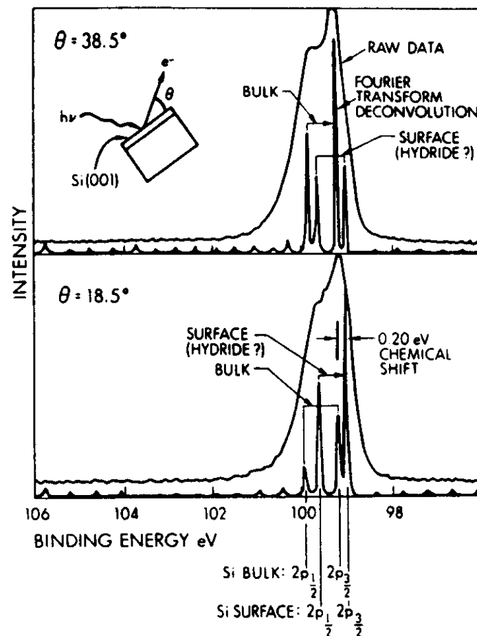
Fig. 8. Si2p spectra at two exit angles from a chemically-cleaned Si surface thought to have a surface hydride present. The raw data and curves obtained via a Fourier-transform (FT) deconvolution procedure are shown. Note the enhancement of the hydride FT peak at \theta = 18.5^\circ . (From Vasquez et al., ref. (20).)
