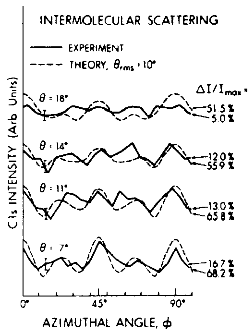
Fig. 42. Comparison of experiment and SSC theory for the azimuthal dependence of Cls emission from c(2 \times 2)\text{CO} on \text{Ni}(001) . The diffraction effects seen are due to intermolecular scattering (cf. Fig. 41). (From Orders and Fadley, ref. (81).)
