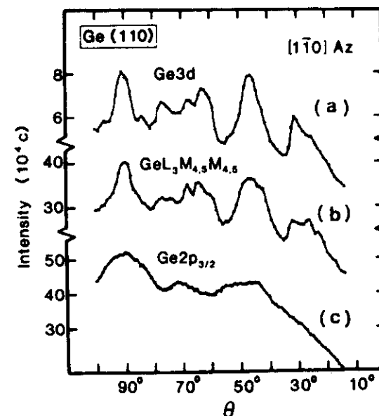
Fig. 28. Experimental polar dependence of Ge XPS and Auger intensities above a Ge(110) surface for \theta scans in a [1\bar{1}0] azimuth. Ge3d and Ge 2p_{3/2} XPS intensities are shown together with the Ge L_3M_{4,5}M_{4,5} Auger intensity. No allowance has been made for the instrument response function. (From Owari et al., ref. (64).)
