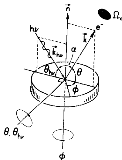
Fig. 1. General geometry for an angle-resolved photoemission experiment. Specimen rotations on the two perpendicular axes shown vary \theta , \phi , and \theta_{h\nu} over their full allowed ranges. \hat{n} is the surface normal. Movement of the electron analyzer relative to the radiation source also can be used to vary \alpha and choose any \theta , \phi , \theta_{h\nu} , \phi_{h\nu} combination, but in XPS this has been done very little to date.
