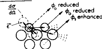
Fig. 51. Schematic explanation of how azimuthal XPD experiments in a
