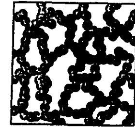
FIG. 2. Schematic diagram of the structure suggested for silica aerogel.
