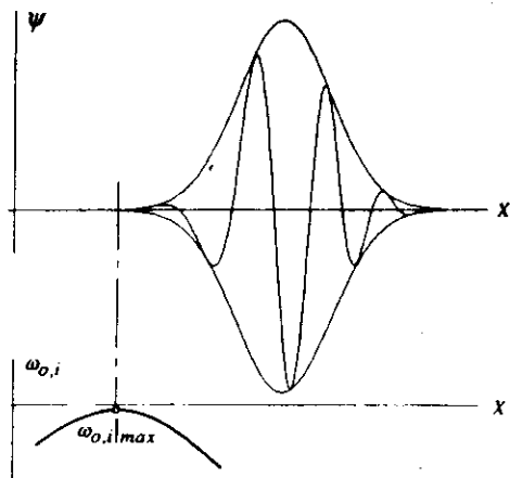
Figure 6 Global mode in spatially developing flows according to the Ginzburg-Landau model with the underlying absolute growth rate \omega_{0,i}(x) .
