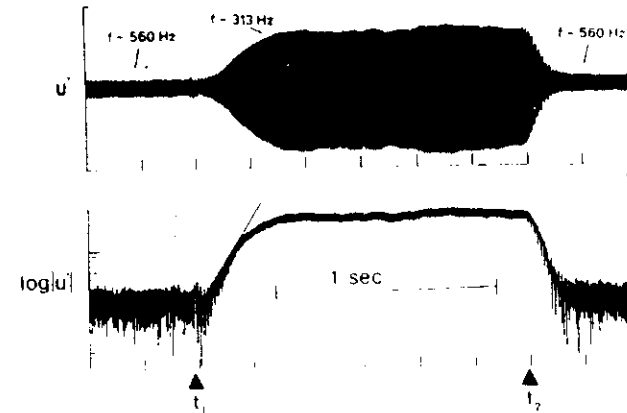
Figure 17. Suppression of vortex shedding behind an oblong cylinder by high-frequency forcing during t < t_1 and t > t_2 at R = 81 ( R_c = 80 ) (from Berger & Schumm 1988, with permission).
