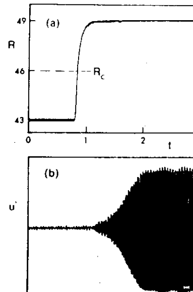
Figure 10 The onset of von Kármán vortex shedding after a step increase of the Reynolds number (from Strykowski 1986, Strykowski & Sreenivasan 1989, with permission). (a) mean velocity (low-pass filtered below 30 Hz); (b) fluctuating velocity
