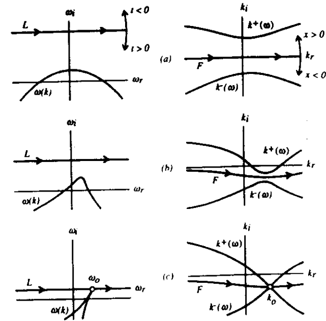
Figure 2 Loci of spatial branches k^+(\omega) and k^-(\omega) as L -contour is displaced downward in the complex \omega -plane. (a), (b), and (c) refer to different stages of the pinching process.
