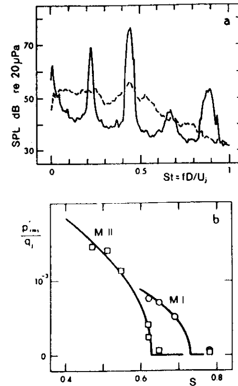
Figure 18 (a) Near-field pressure spectrum in a round air jet at (x/D, r/D) = (0.2, 1.0) (from Monkewitz et al. 1989c). —, hot jet with S \equiv \rho_c/\rho_a = 0.47 and R = 7500 ; ---, cold jet ( S = 1 ) of equal dynamic head. (b) Amplitude of the dominant near-field pressure oscillation at R = 7500 , normalized by the jet dynamic head, versus S (from Monkewitz et al. 1989a). —, Equation (58) fitted to the data.
