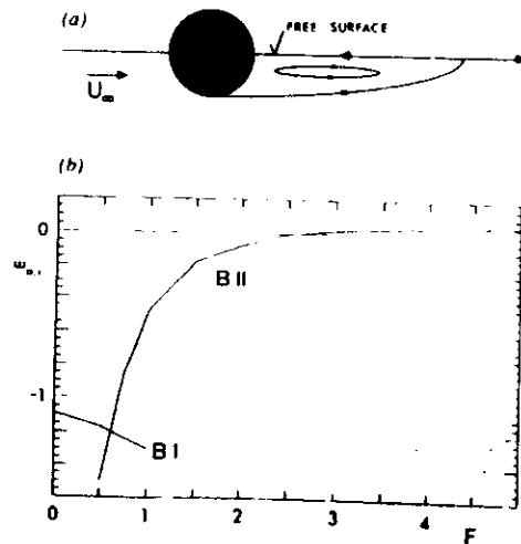
Figure 11 The stability of the floating wake (from Triantafyllou & Dimas 1989, with permission). (a) schematic of the mean flow; (b) absolute growth rate versus Froude number.
