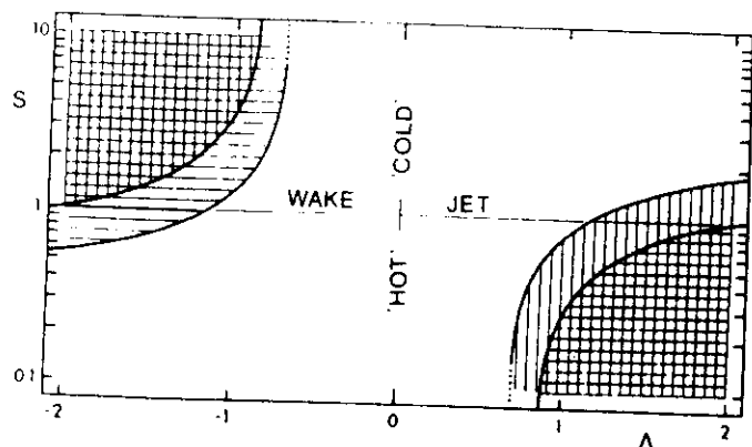
Figure 13. Regions of absolute instability in the (S, \Lambda) -plane for the sinuous mode (horizontal hatching) and the varicose mode (vertical hatching) in an inviscid, incompressible jet wake bounded by vortex sheets (from Yu & Monkewitz 1988).
