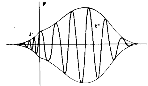
Figure 5 Sketch of response to time-harmonic forcing in spatially developing flows.
