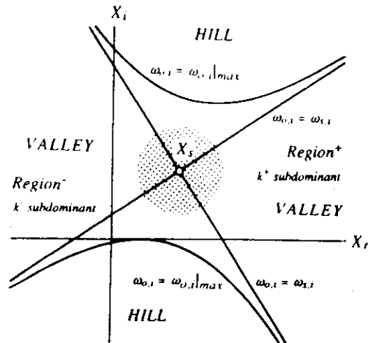
Figure 7. Sketch of different regions in the complex X -plane ( X = X_r + iX_i ). The curves represent contours \omega_0(X) = \text{constant} in the vicinity of the saddle point X_s . Shaded area denotes the
