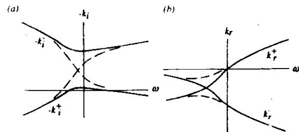
Figure 3. Spatial branches k^+ and k^- of the Ginzburg-Landau equation in the convectively unstable case (—). (a) spatial growth rate -k_i , versus real frequency \omega ; (b) k_r , versus \omega .
