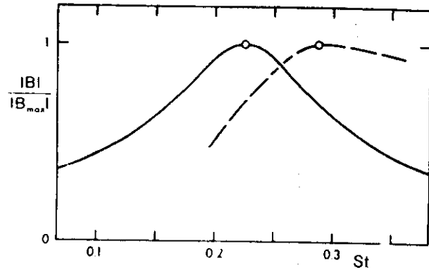
Figure 9 Normalized gain in a two-dimensional jet from Equation (57) (—) and from locally parallel theory (---) (from Monkewitz et al. 1987)
