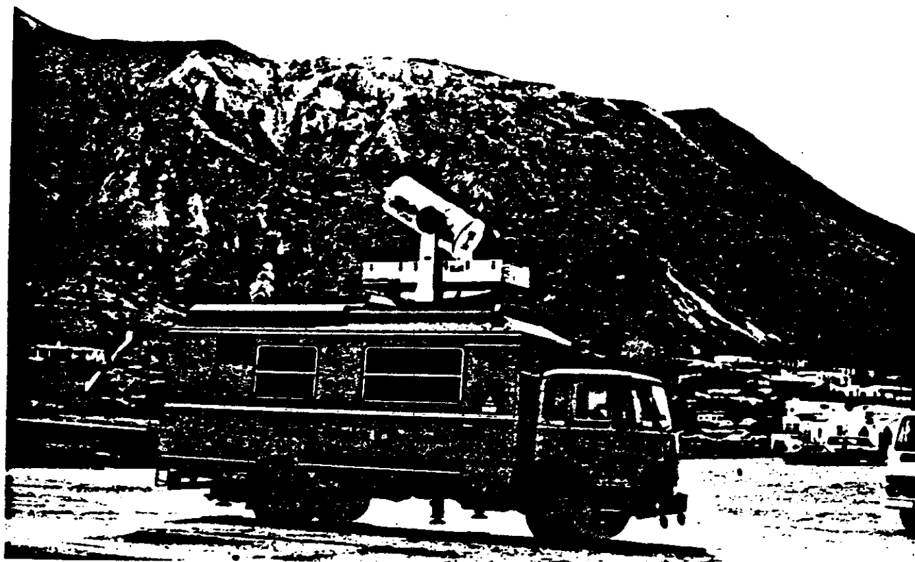
FIGURE 15. CISE-ENEL DIAL system. This picture was taken in 1983 during the campaign for the detection of sulfur dioxide emitted by the fumaroles of a volcano in Vulcano Island (Italy).
