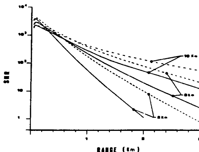
FIGURE 13. Signal-to-noise ratios relevant to the signals in Figure 12.
