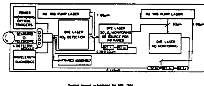
FIGURE 21. Block diagram of the mobile DIAL of National Physical Laboratory, Teddington, UK (NPL). (Courtesy of National Physical Laboratory.)
