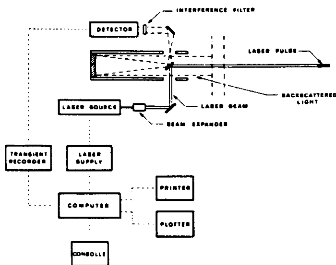
FIGURE 1. Block diagram of a DIAL system.
