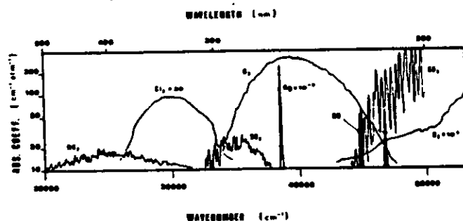
FIGURE 5. Absorption spectra and absorption coefficients (in units \text{cm}^{-1} \text{atm}^{-1} ) of some gases in the range 200 to 500 nm (20,000 to 50,000 \text{cm}^{-1} ): \text{SO}_2 , 137-140,143-145 \text{NO}_2 , 140-141 \text{Cl}_2 , 142 \text{NO} , 138,143 \text{O}_2 , 146 \text{Hg} , 151 \text{O}_3 , 78,92
