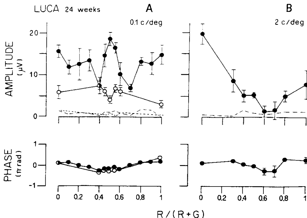
FIGURE 16. Amplitude and phase of VEPs as a function of colour-ratio for infant Luca, 24 weeks of age, at two spatial frequencies, 0.1 c/deg (A) and 2 c/deg (B). Contrast was 80% for the solid circles, and 20% for the open circles, and temporal frequency 5 Hz. Each point is the mean of 200 sums, with vertical bars indicating standard error, and broken lines indicating noise amplitudes.
