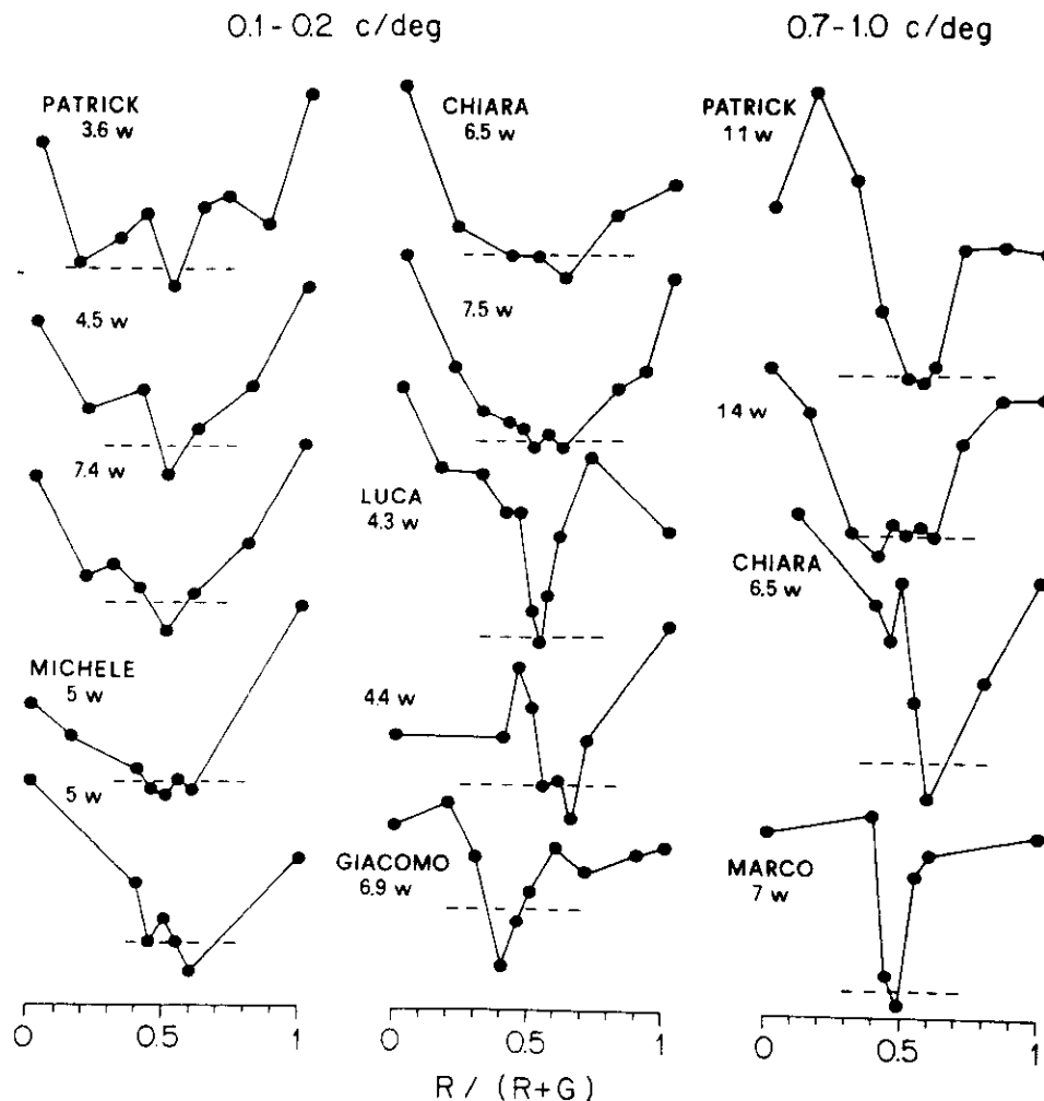
FIGURE 4. Further examples where there was no reliable response at equiluminance, at 0.1–0.2 c/deg (two left-hand columns) and 0.7–1.0 c/deg (right-hand column). The amplitudes have been scaled arbitrarily to accommodate all the curves on the figure. The dashed line shows the average asynchronous-noise for all colour-ratios in that session.
