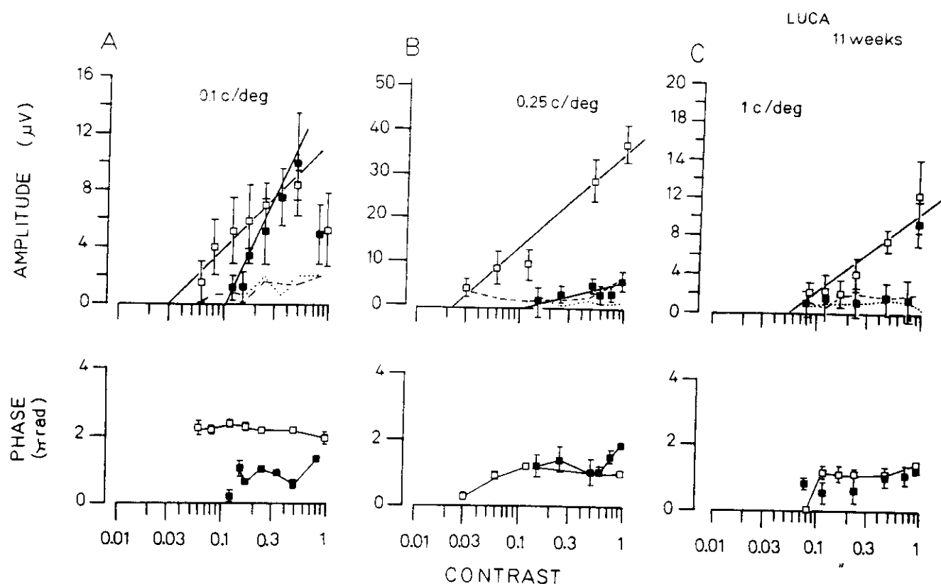
FIGURE 7. Amplitudes and phases of VEPs as a function of contrast for infant Luca, 11 weeks old, for three stimulus spatial frequencies, all measured at 3 Hz: 0.1 (A), 0.25 (B), and 1.0 (C) c/deg. Open squares: green-black pattern (colour-ratio 0), solid squares: red-green pattern (colour-ratio 0.5). Other conventions as for Fig. 6.
