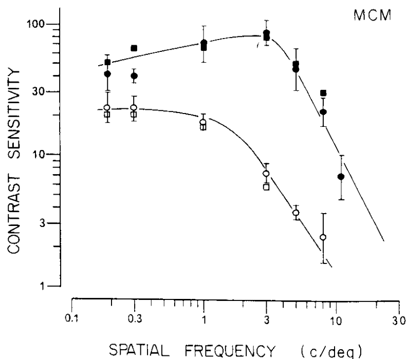
FIGURE 10. Contrast sensitivities as a function of spatial frequency for an adult subject (MCM). The circles indicate estimates from extrapolating VEP contrast response curves, and squares thresholds from direct psychophysical measurement, using standard method-of-adjustment techniques. The solid symbols refer to red-black luminance patterns (colour-ratio 1.0), and open symbols to red-green equiluminant patterns (colour-ratio 0.52). The temporal frequency was 5 Hz in all cases.
