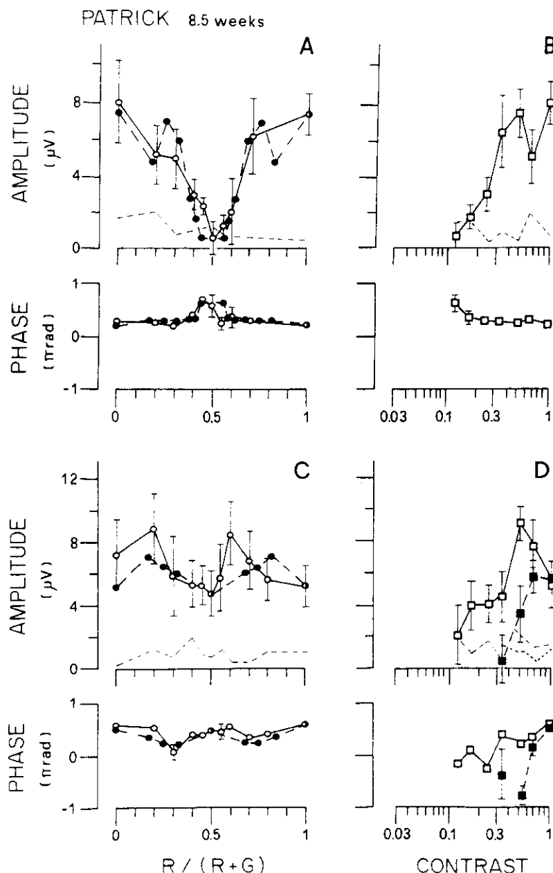
FIGURE 8. (A) and (C) Amplitude and phase of VEPs recorded from infant Patrick at 8.5 weeks of age, as a function of colour-ratio (open circles). The stimulus was 0.4 c/deg [(A) and (B)] or 0.1 c/deg [(C) and (D)], 3 Hz and 100% contrast. In (B) and (D), the amplitude and phase of VEPs are plotted against contrast for a plaid pattern of colour-ratio 1 (red-black, open squares) or 0.5 (red-green, solid squares). Noise amplitudes are indicated by the broken lines, except for those relative to the red-green pattern in (D), indicated by a dotted line. The solid circles in (A) and (C) are amplitudes and phases predicted from the data reported in (B) and (D), respectively, as explained in the text.
