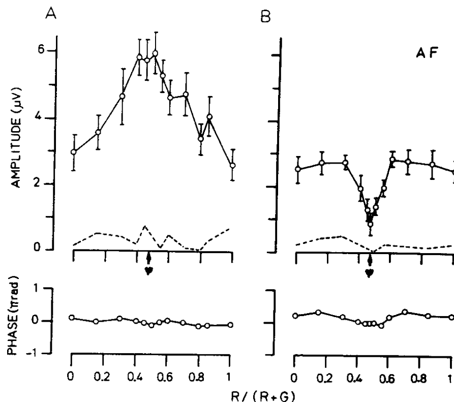
FIGURE 1. Amplitude and phase of VEPs recorded from an adult subject (AF) for plaid patterns of various colour-ratios. Colour-ratio 0 represents a green-black pattern, and 1 a red-black pattern, both of pure luminance contrast. The arrow indicates the ratio of red-to-total luminance corresponding to the equiluminance value evaluated psychophysically. Each point is the mean of 240 and 400 sums for (A) and (B) respectively, with the vertical bars indicating standard error. The amplitude of the asynchronous noise estimates are represented by the broken line. Stimulus spatial frequency: 1 c/deg, temporal frequency 6.2 Hz (A), 7.5 Hz (B). Contrast 90% (A), 30% (B). One condition leads to a local maximum in amplitude, the other to a local minimum.
