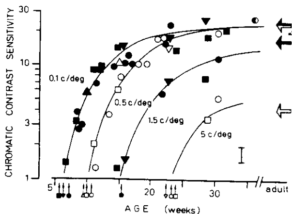
FIGURE 14. Development of contrast sensitivity for red-green patterns of four different spatial frequencies. The different symbols refer to longitudinal measurements of different infants, and adult values are indicated by the arrows on the right. The arrows below the abscissa indicate, for each spatial frequency, the last recording session at which no response could be elicited by chromatic stimuli at 100% contrast. The vertical bar is the average standard error of the experimental points. The symbols refer to different infants: circles, Patrick; squares, Luca; upright triangles, Felix; inverted triangles, Michele.
