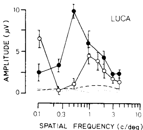
FIGURE 17. VEP amplitudes as a function of spatial frequency for infant Luca, 11 weeks of age. Stimulus contrast was 95%, and temporal frequency 4.3 Hz. Solid circles refer to red-black patterns (colour-ratio 0), and open circles to red-green pattern (colour-ratio 0.5). Each point is the mean of 160 sums. Noise amplitudes corresponding to the red-black and red-green stimulus conditions, are indicated by dashed and dotted lines (respectively).
