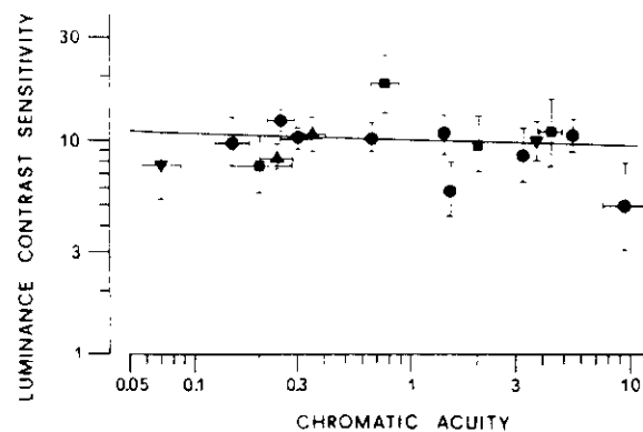
FIGURE 15. Luminance contrast sensitivity at the resolution limit for chromatic response, as a function of the chromatic resolution limit. The vertical and horizontal error bars indicate the standard errors in the two estimations, and the continuous line the linear regression (weighting for standard error). The different symbols refer to different infants: circles Patrick, measured at 7.4, 8, 8.5, 11, 14, 15, 21, 23 and 35 weeks; squares, Luca, 6, 11, 14 and 29 weeks; upright triangles, Felix, 8.5 and 9.2 weeks; inverted triangles, Michele, 6 and 22.5 weeks.
