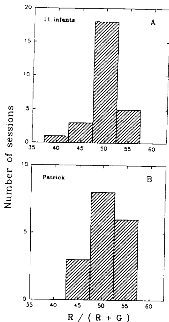
FIGURE 5. Distribution of colour-ratios producing equiluminance (defined as either a local minimum or maximum in the amplitude vs colour-ratio functions). (A) Shows 27 separate estimates from 11 of the infants (discounting Patrick), and (B) shows 17 separate measurements of equiluminance for Patrick. The estimates were made at various ages, temporal frequencies and spatial frequencies (all < 1 c/deg).
