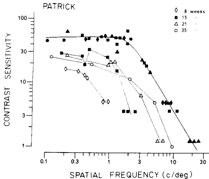
FIGURE 13. Contrast sensitivity for infant Patrick (taken from Fig. 11), where the data from the earlier sessions have been rescaled in both sensitivity and resolution to cause the luminance sensitivities (solid symbols) to fall as near as possible to those measured at 35 weeks. The scaling factors (in log-units) for sensitivity and resolution (respectively) were: 0.7, 0.6 at 8 weeks; 0.55, 0.3 at 15 weeks; 0.1, 0.3 at 21 weeks; and 0, 0 at 35 weeks. Note that while this rescaling aligns the luminance sensitivities along a common curve, the chromatic sensitivities measured at different ages remain quite distinct.
