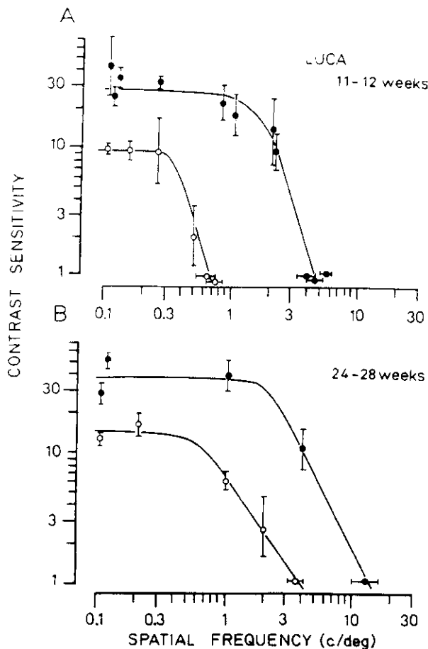
FIGURE 12. VEP contrast sensitivity for infant Luca at 11-12 (A) and 24-28 (B) weeks. Solid circles refer to luminance patterns, and open circles to red-green patterns (colour-ratio between 0.5 and 0.6). The temporal frequency was 5 Hz.
