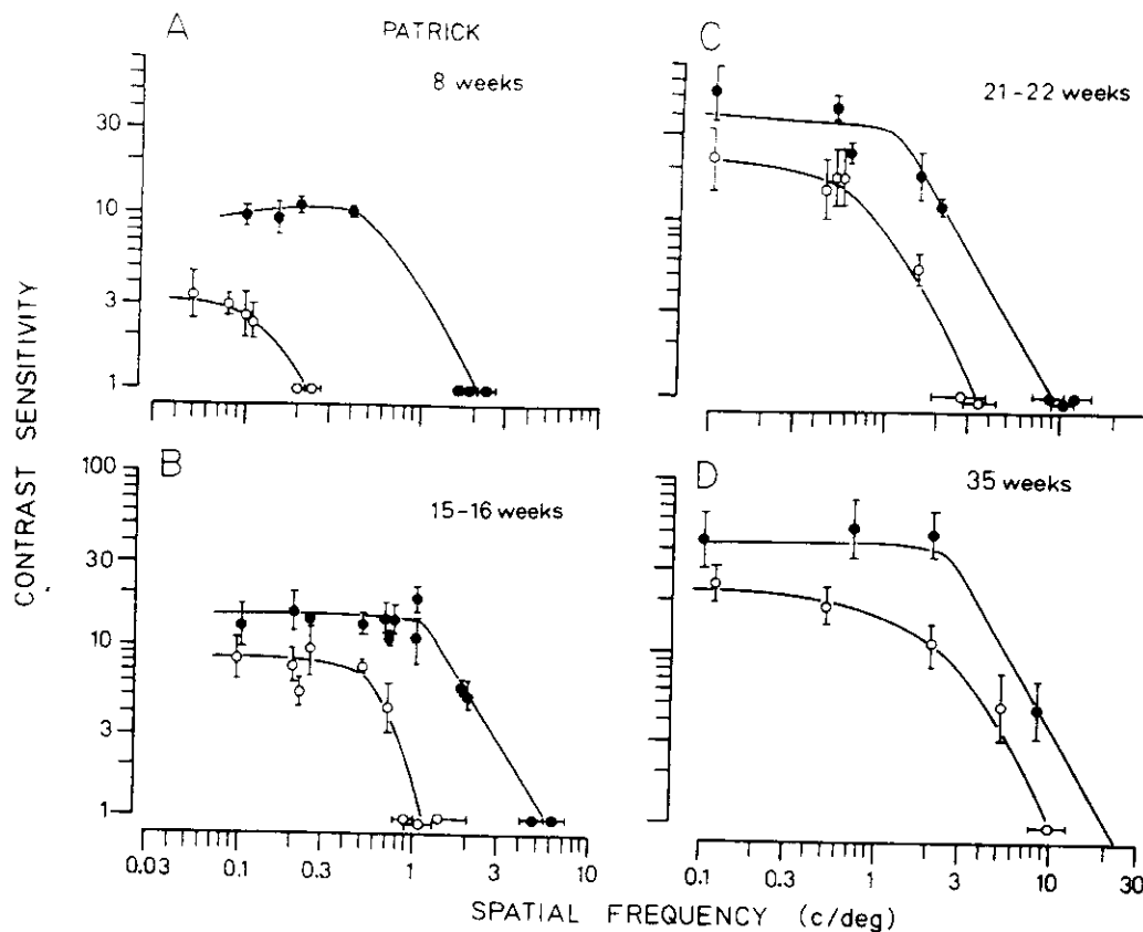
FIGURE 11. Contrast sensitivity estimated from VEPs, as a function of spatial frequency for infant Patrick at ages of 8 (A), 15-16 (B), 21-22 (C) and 35 (D) weeks. Solid circles refer to luminance patterns, and open circles to red-green patterns at equiluminance (colour-ratio between 0.45 and 0.5). The temporal frequency was 3 Hz for (A) and (B) and 5 Hz for (C) and (D). Vertical bars (for contrast sensitivity data) and horizontal bars (for acuity data) indicate standard error.
