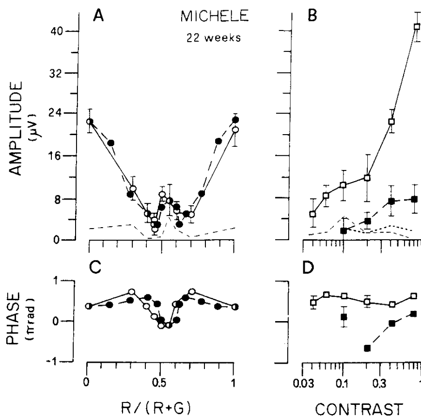
FIGURE 9. Same conventions as Fig. 8, for infant Michele at 22 weeks. The stimulus was 1 c/deg, 5 Hz and for the measurements as a function of colour-ratio, 40% contrast. Equiluminance was evaluated as r = 0.55 , and this value was considered to give maximal chromatic contrast and zero luminance contrast. Where there were no corresponding measurements of luminance and chromatic response of exactly appropriate contrast, we interpolated linearly between adjacent points.
