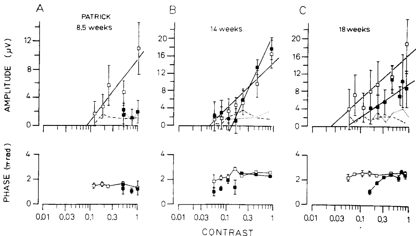
FIGURE 6. Amplitudes and phases of VEPs as a function of contrast for infant Patrick at the age of 8.5 (A), 14 (B), and 18 (C) weeks, for a stimulus of 0.2 c/deg, 3 Hz. Open squares indicate luminance patterns [colour-ratio 1.0 for (A) and 0 for (B) and (C)], and solid squares red-green patterns (colour-ratio 0.5). Each point has between 140 and 280 sums, with vertical bars indicating standard errors, derived from the variation of the partial-sum packets (see Fig. 2). The lines are best fit linear regressions, weighting each point for standard error. Noise amplitudes are indicated by dashed and dotted lines for luminance and chromatic stimuli (respectively). Phase data corresponding to amplitudes larger than noise have been connected by solid lines.
