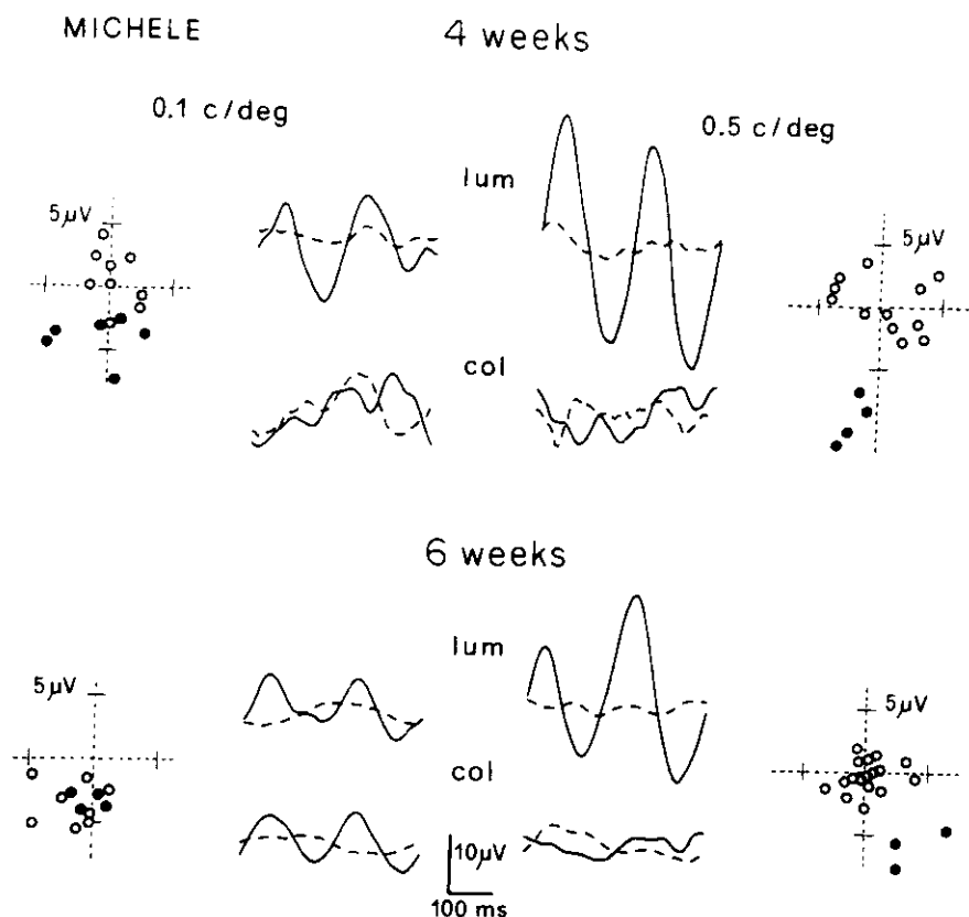
FIGURE 2. Examples of VEP records for luminance and equiluminant stimuli from infant Michele at 4 and 6 weeks to two different spatial frequencies. The continuous traces show the VEP averaged in synchrony with the stimulus reversal rate, and the dashed lines that averaged at 1.1 times the stimulus rate (which provides an estimate of noise). The adjacent polar plots show the amplitude (norm) and phase (argument) of partial (20 sum) packets, with solid symbols for the luminance stimuli and open symbols for the chromatic stimuli, both of 100% contrast. These give an indication of the variability of the response (from which the standard errors of all subsequent plots were calculated). While the response to luminance was reliable at all conditions (shown both by the relative amplitude of the signal to noise in the averaged records and by the relatively close clustering of the partial packets), only at 0.1 c/deg and 6 weeks did the chromatic stimulus produce a reliable response.
