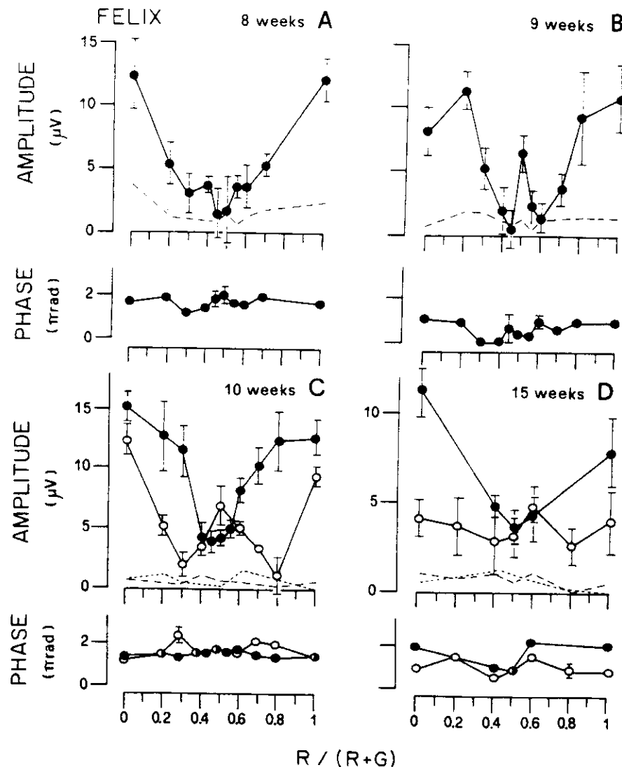
FIGURE 3. Amplitude and phase of VEPs as a function of colour-ratio, recorded from infant Felix at the age of 8 (A), 9 (B), 10 (C) and 15 (D) weeks. Each point is the mean of 200 sums in (A) and (C), and 140 in (B) and (D). The stimulus was 0.3 c/deg and 3 Hz: the solid circles refer to contrasts of 100%, and the open circles to contrasts of 50%.
