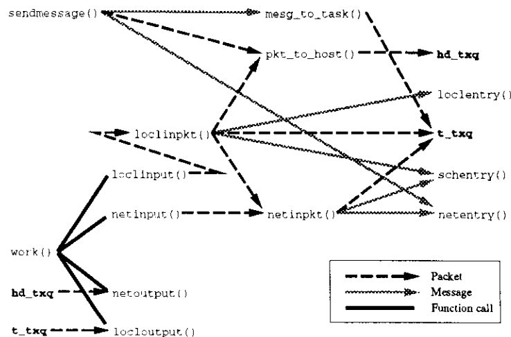
Figure 16: Packet and Message Routing
