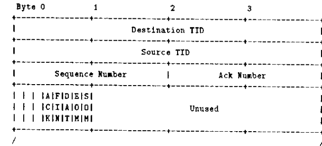
Figure 13: Pvmd-pvmd Packet Header
