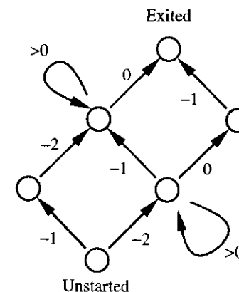
Figure 18: Output States of a Task
