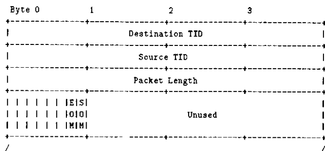
Figure 15: Pvmd-Task Packet Header
