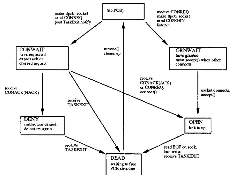
Figure 17: Task-Task Connection State Diagram
