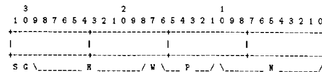
Figure 11: MPP Task ID
